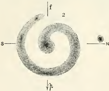
FIGURE 1. SPIRAL NEBULA.
