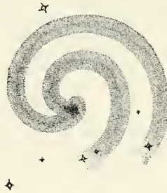
FIGURE 2. SPIRAL NEBULA.
