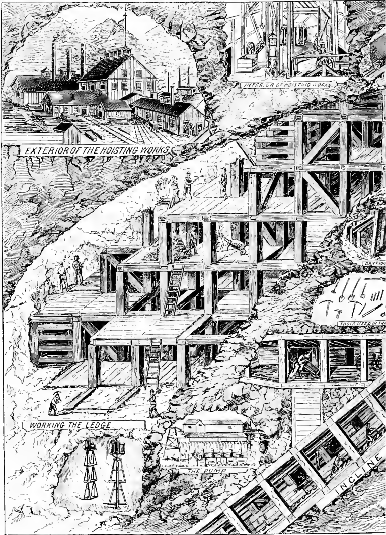
Sectional View
