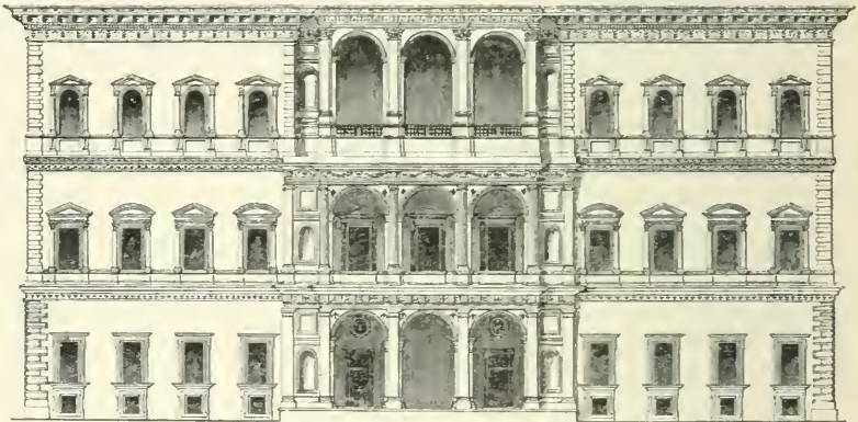
58. Garden front of the Farnese Palace, Rome. Scale 100 feet to 1 inch. From Letarouilly.
