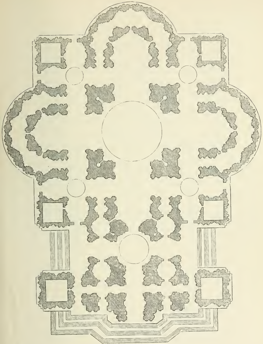
24. Plan of St. Peter's as proposed by Sangallo. From Bonanni. No scale.
