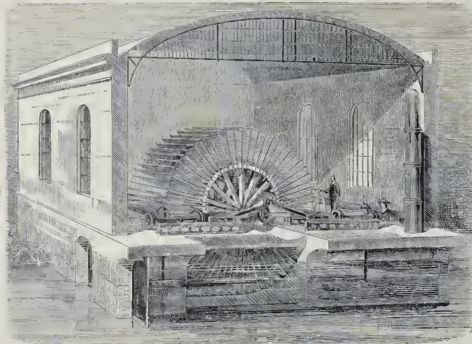
LA MACHINE DE MARLY.
