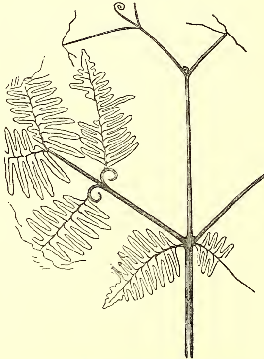
FIG. 28.—Habit of Gleichenia Hantonensis restored.
