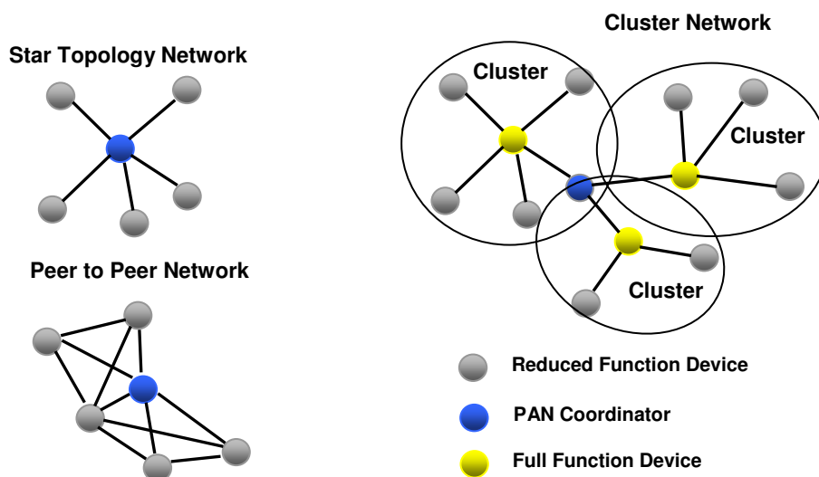
Figure 3 – IEEE 802.15.4 Network Topologies (from ref. [6])
