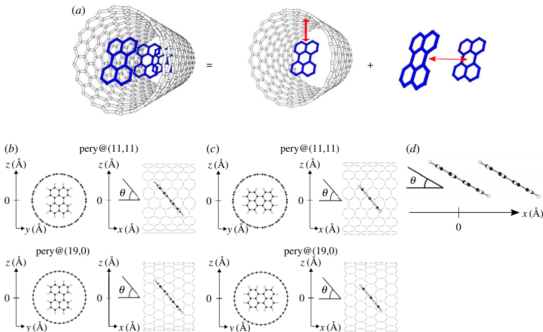
Figure 1. (a) A structural model to calculate the formation energy of a CNT encapsulating a perylene chain, which is decomposed into the encapsulation energy of perylene in the CNT and the interaction energy between adjacent perylene molecules. White and blue cylinders denote the covalent networks of the CNT and perylene. Structural models to calculate the encapsulation energy of perylene in (11,11) and (19,0)CNTs in which perylene is rotated by an angle \theta with respect to its C_2 axis (b) parallel and (c) perpendicular to the zigzag edges. (d) A structural model for investigating the interaction between adjacent perylene molecules. Black and white circles denote C and H atoms, respectively.
