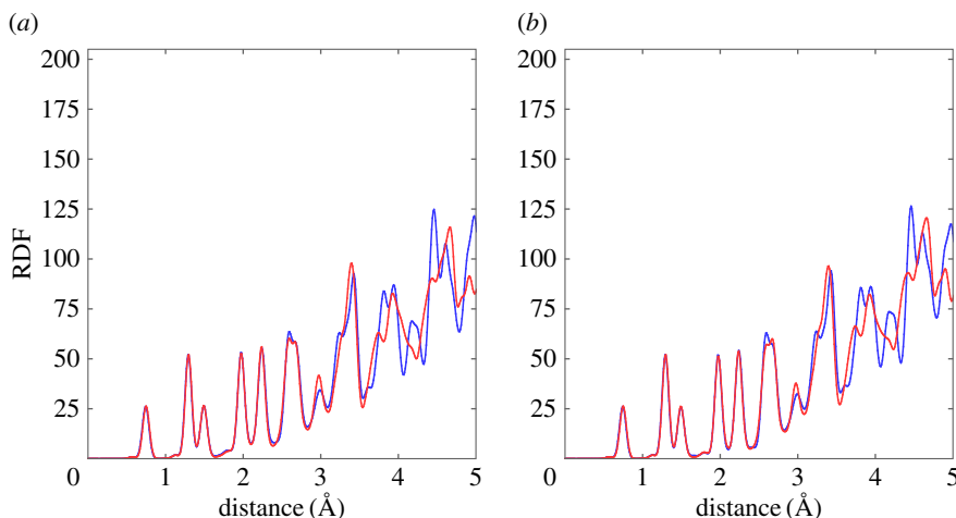
Figure 3. RDFs of CNTs encapsulating perylene with a tilt angle \theta of (a) 0^\circ and (b) 70^\circ with respect to the C_2 axis parallel to the zigzag edges of perylene. Blue and red lines denote the radial distribution functions of perylene encapsulated in (11,11) and (19,0)CNTs, respectively.
