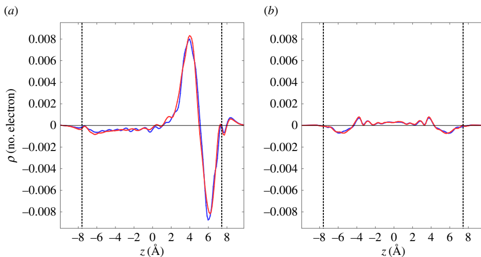
Figure 4. Plane averaged charge redistribution along the z direction inside a CNT upon perylene encapsulation with molecular tilt angles of (a) 0^\circ and (b) 70^\circ with respect to the C_2 axis parallel to the zigzag edges of perylene. Blue and red lines denote the electron density of (11,11) and (19,0)CNTs, respectively, encapsulating perylene. The vertical dashed lines indicate the position of the CNT walls.
