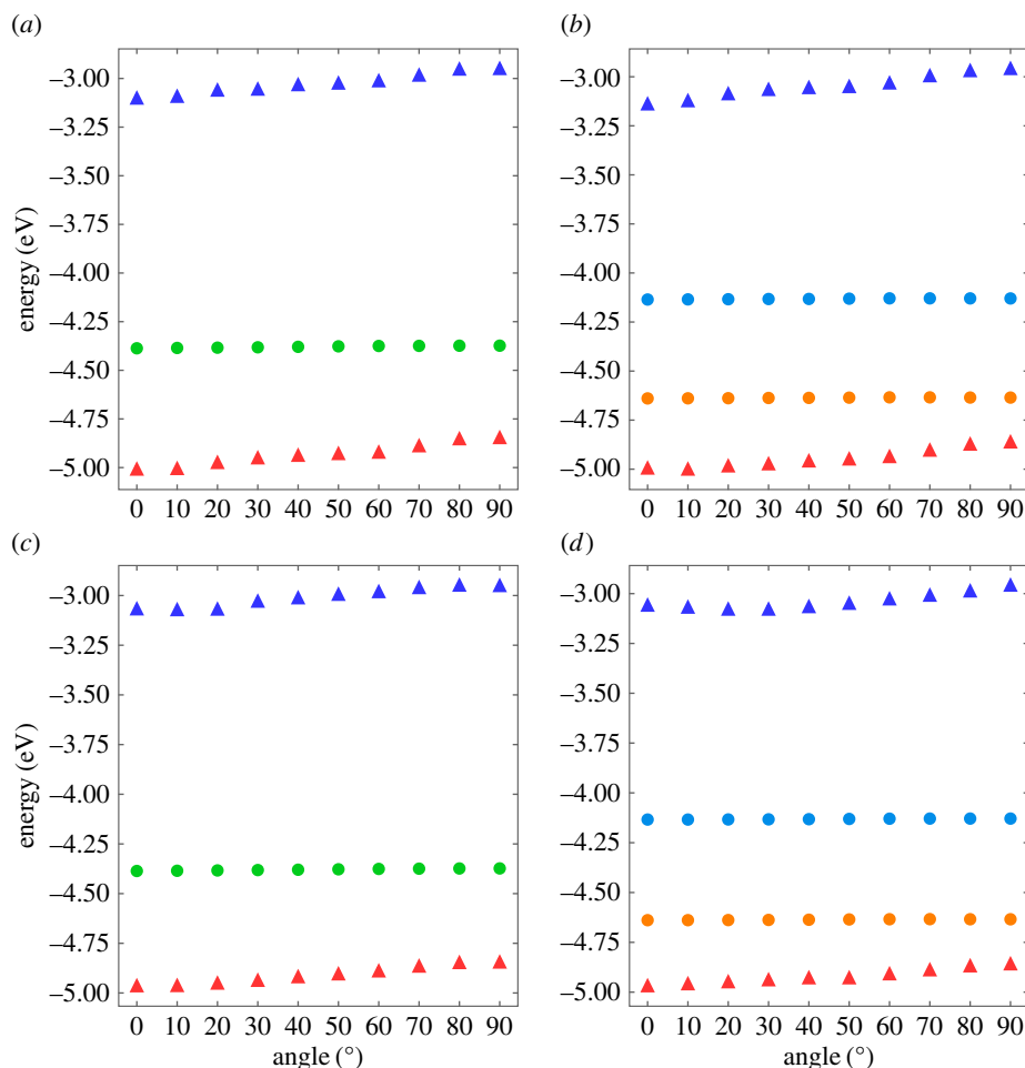
Figure 5. Electronic energy levels near the Fermi level of (a) (11,11)CNT and (b) (19,0)CNT encapsulating a perylene molecule as a function of the rotational angle \theta with respect to the C_2 axis parallel to the zigzag edges of perylene. Electronic energy levels near the Fermi level of (c) (11,11)CNT and (d) (19,0)CNT encapsulating a perylene molecule as a function of the rotational angle \theta with respect to the C_2 axis parallel to the armchair edges of perylene. Red triangles, blue triangles, green circles, orange circles and light blue circles denote the HO state of perylene, the LU state of perylene, the Dirac point of (11,11)CNT, the valence band top of (19,0)CNT and the conduction band bottom of (19,0)CNT, respectively. The energies are measured from that of the vacuum level.
