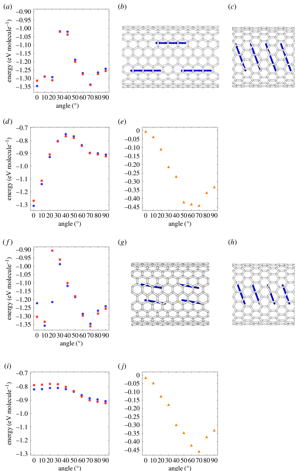
Figure 2. (a) The formation energies of (11,11) and (19,0)CNTs encapsulating perylene as a function of the rotational angle \theta with respect to the C_2 axis parallel to the zigzag edges of perylene. Optimized structures of the ground state perylene arrangements in (b) (11,11)CNT and (c) (19,0)CNT. Decomposed interaction (d) between CNT and perylene and (e) between perylene molecules as a function of the rotational angle \theta with respect to the C_2 axis parallel to the zigzag edges of perylene. (f) The formation energies of (11,11) and (19,0)CNTs encapsulating perylene as a function of the rotational angle \theta with respect to the C_2 axis parallel to the armchair edges of perylene. Optimized structures of the ground state perylene arrangements in (g) (11,11)CNT and (h) (19,0)CNT. Decomposed interactions (i) between CNT and perylene and (j) between perylene as a function of the rotational angle \theta with respect to the C_2 axis parallel to the armchair edges of perylene. White and blue cylinders denote the covalent networks of CNT and perylene, respectively. Blue circles, red squares and orange triangles denote the energies associated with perylene-(11,11)CNT, perylene-(19,0)CNT and a perylene pair, respectively.
