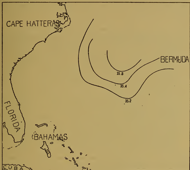
FIG. 21.—Salinity at 1,000 meters.
