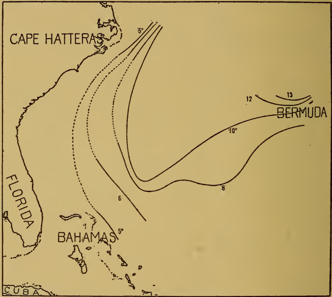
FIG. 20.—Temperature at 1,000 meters.
