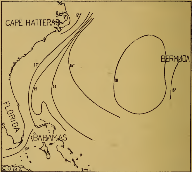
FIG. 18.—Temperatures at 600 meters.
