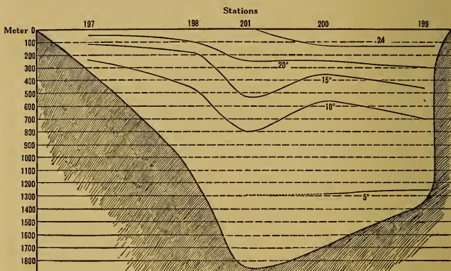
FIG. 24.—Temperature profile, Key West-Habana.
