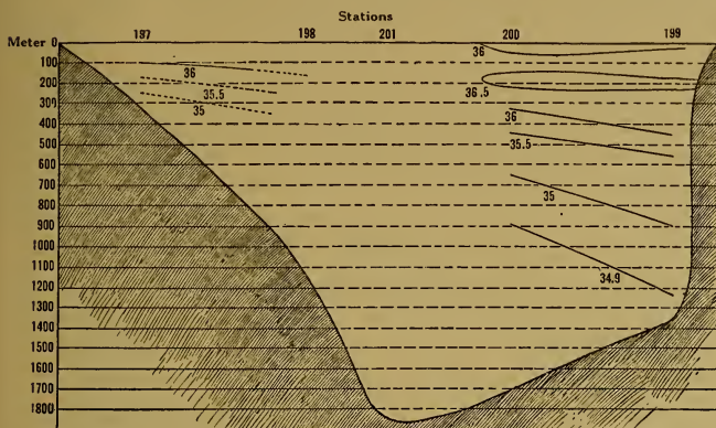
FIG. 25.—Salinity profile, Key West-Habana.
