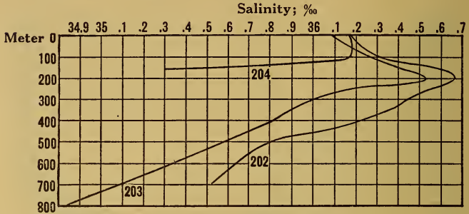
Fig. 27.—Salinity sections on the Gun Cay-Cape Florida line; stations 10202, 10203, 10204.
