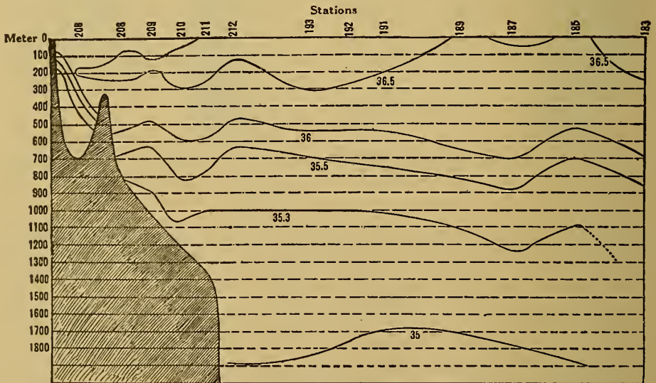
FIG. 16.—Salinity profile of the upper 1,800 meters, from Florida to a point 200 miles southwest of Bermuda.
