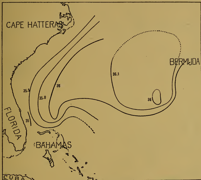
FIG. 19.—Salinity at 600 meters.
