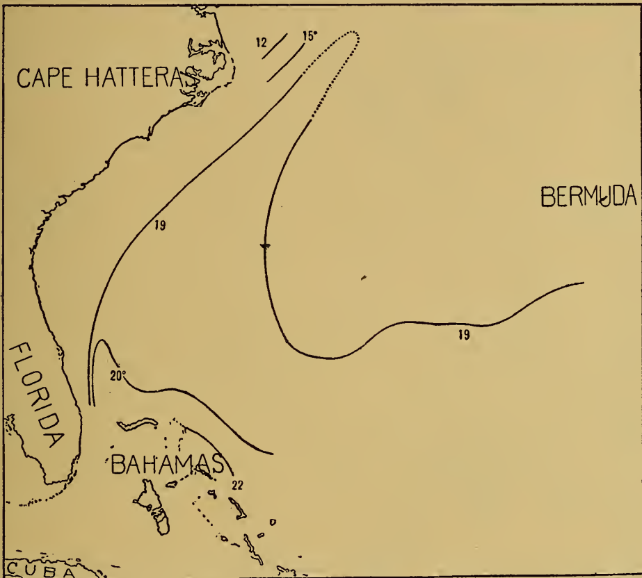
FIG. 17.—Temperatures at 200 meters.
