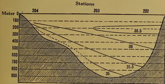
FIG. 29.—Salinity profile across the Straits of Florida, Gun Cay to Cape Florida.
