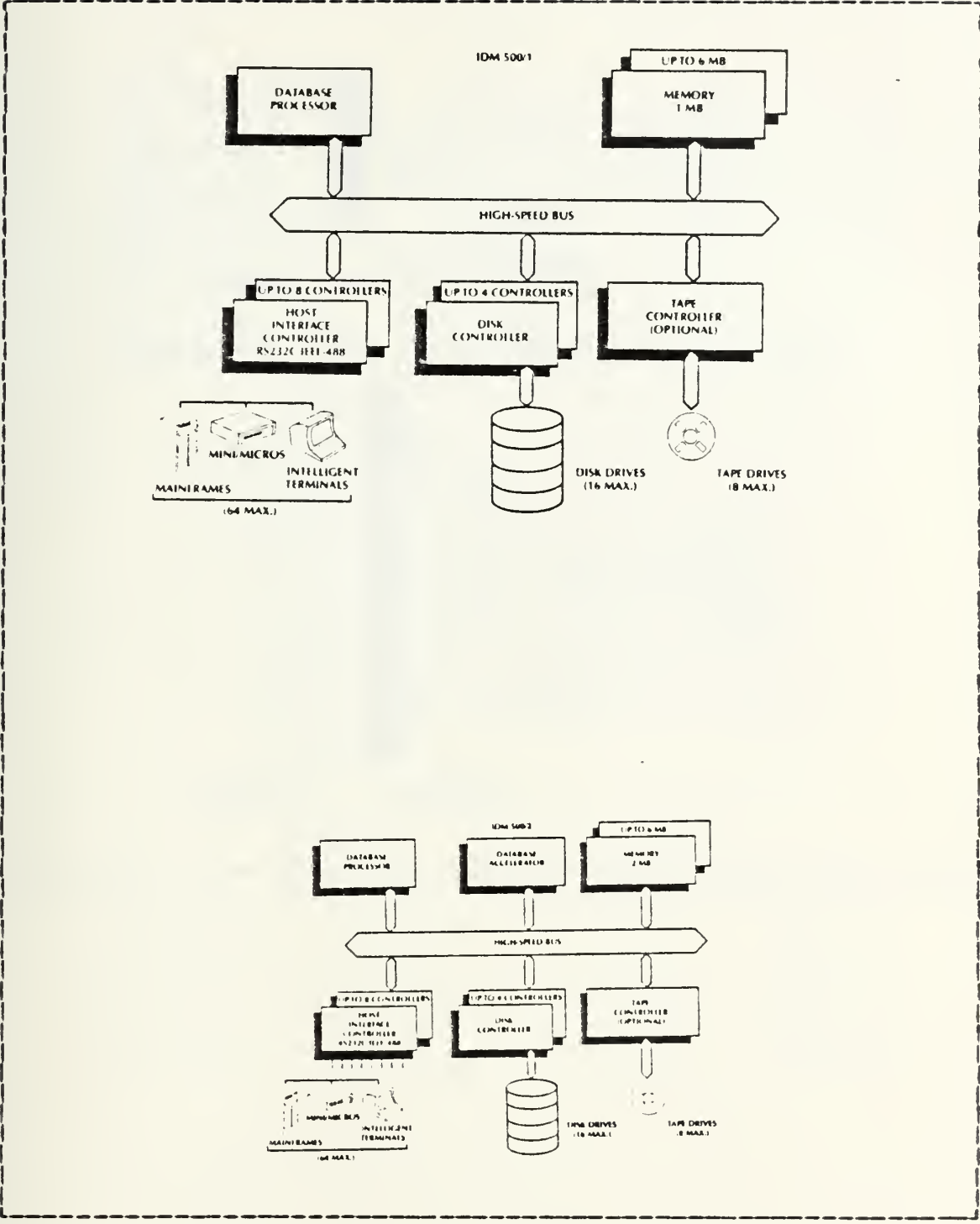
Figure 4.2 Architecture of the IDM 500/1 and 500/2.
