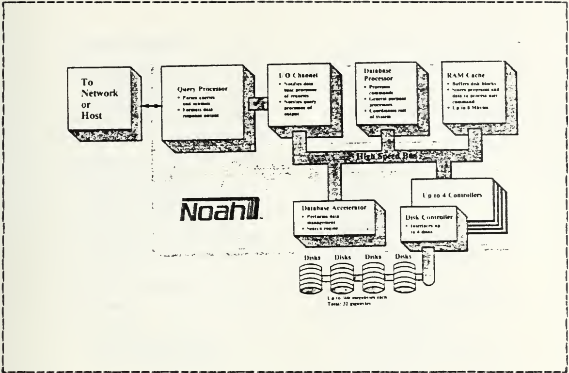
Figure 4.8 NOAH's Hardware Configuration.
