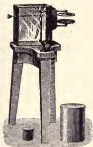
FIG. 5.—Curie's Electroscope for the study of Radio-activity.
