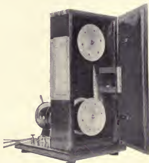
FIG. 23.—Showing Interior of Ruhmer's Photographophone.
