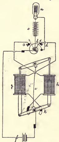
FIG. 24.—Diagram of Circuits of "Selenium" Buoy.
