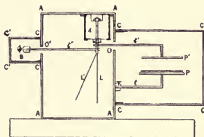
FIG. 5.—Curie's Electroscope for the study of Radio-activity.
