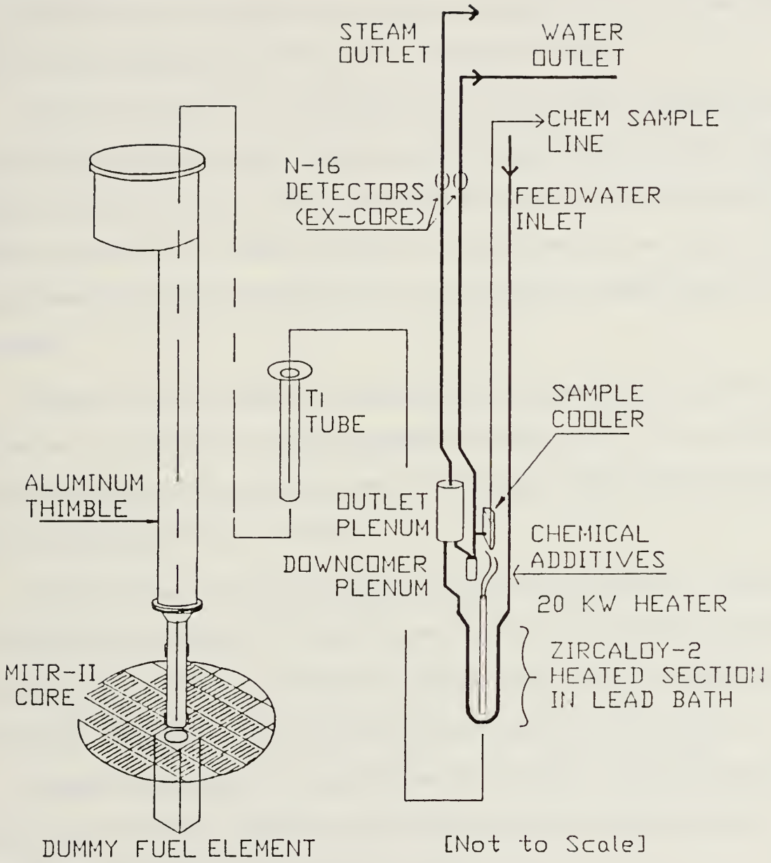
Figure 1.2: BCCL In-Reactor Components
