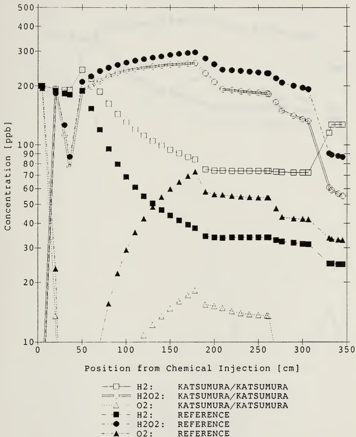
FIGURE 5.12: BCCLMIT G-VALUE COMPARISON - COMBINATION #4
