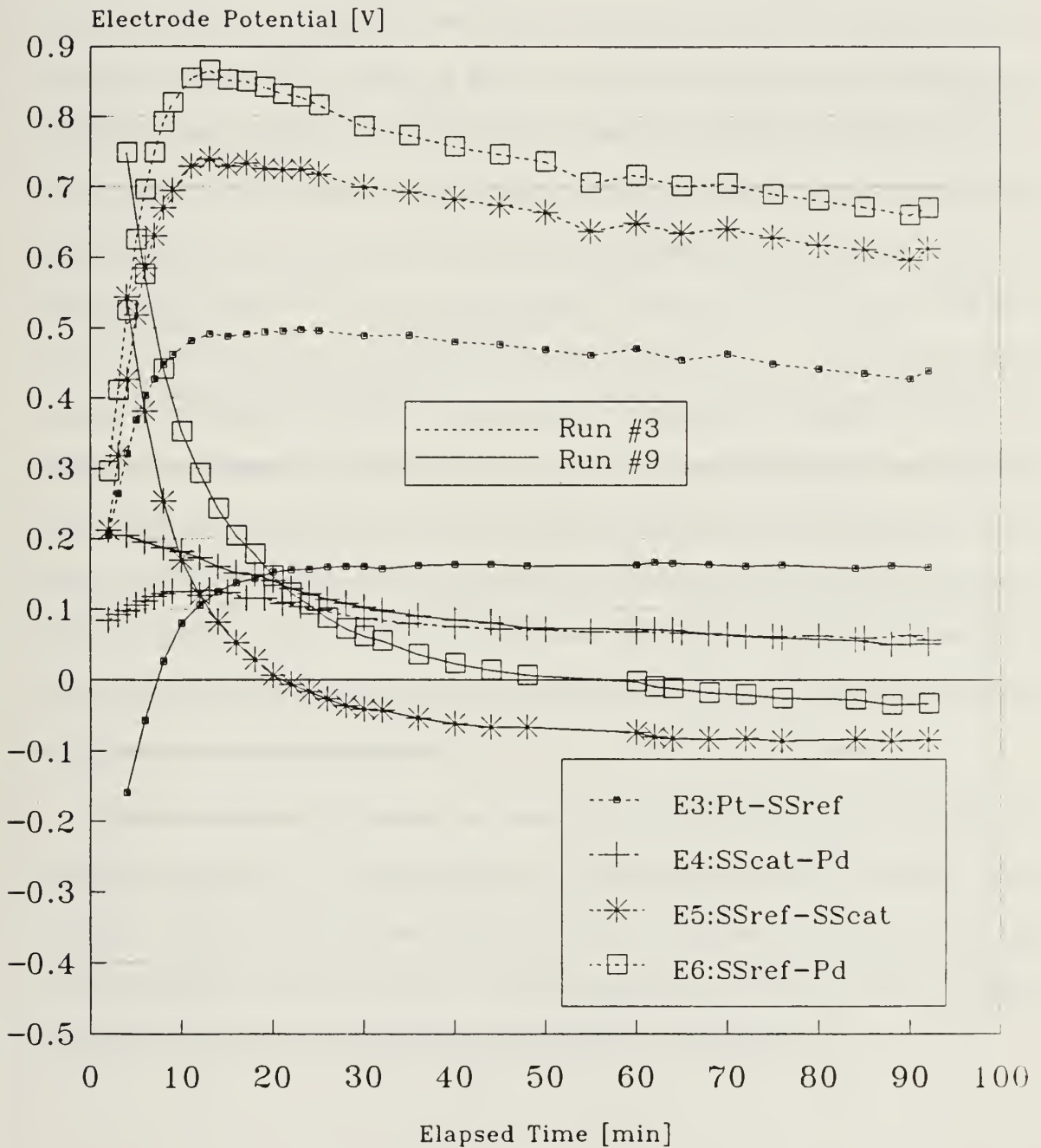
Figure 4.7: Hot Reference Run Comparison
