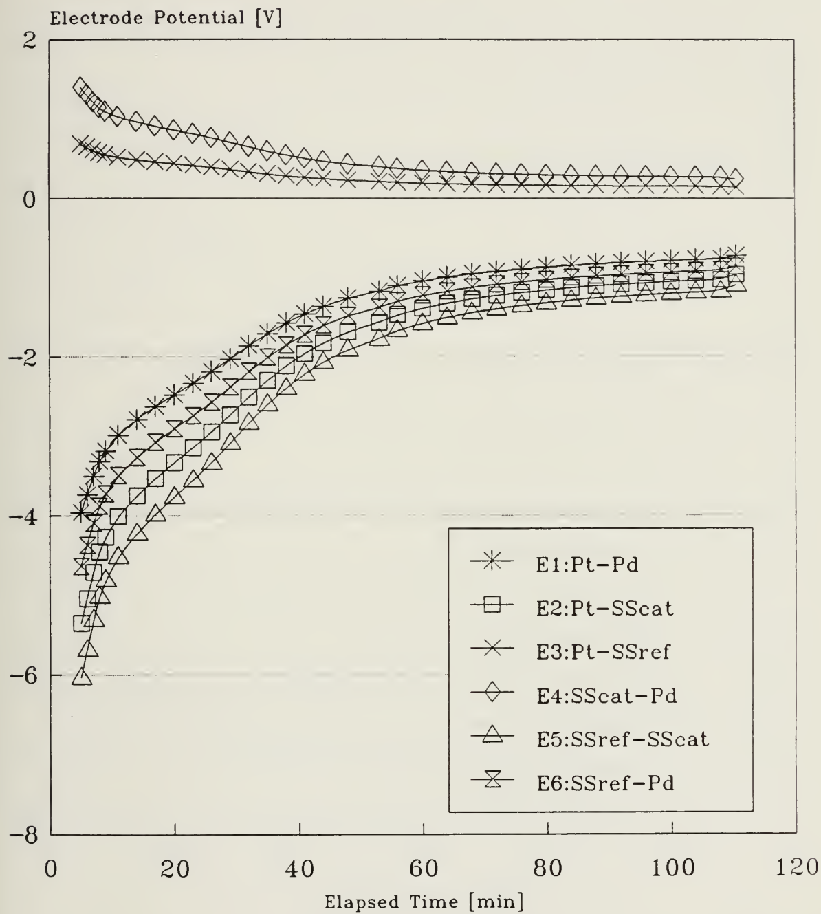
Figure C.2: Cold Reference Run #3
