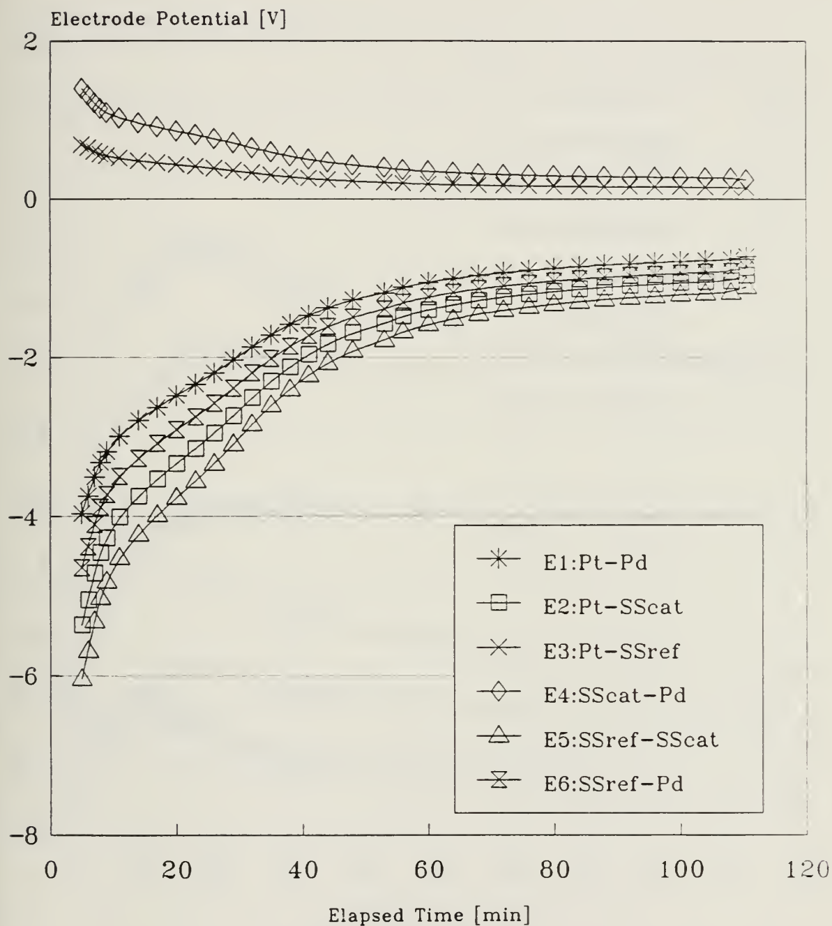
Figure C.3 Cold Reference Run #4
