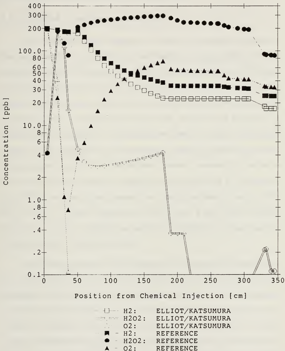
FIGURE 5.13: BCCLMIT G-VALUE COMPARISON - COMBINATION #5
