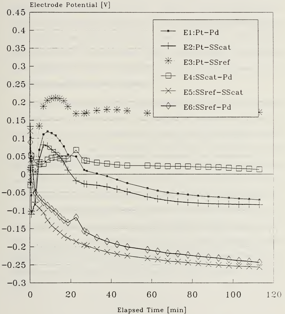
Figure 4.5: Passivated-Cold Reference Run #1
