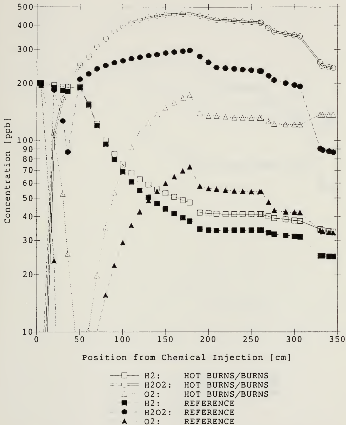
FIGURE 5.11: BCCLMIT G-VALUE COMPARISON - COMBINATION #3
