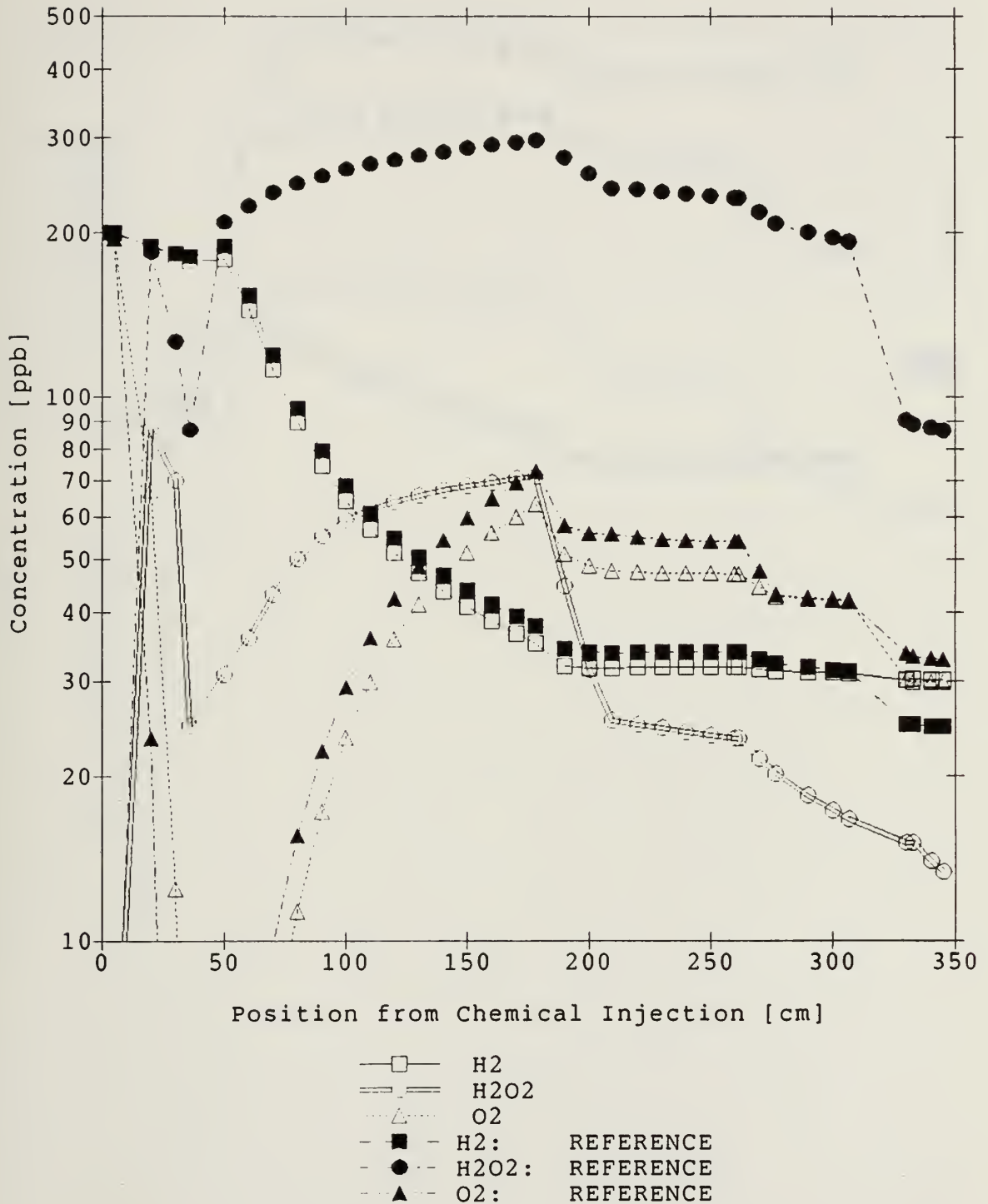
FIGURE 5.20: REVISED EQUATION SET STUDY - NOTRE DAME SET
