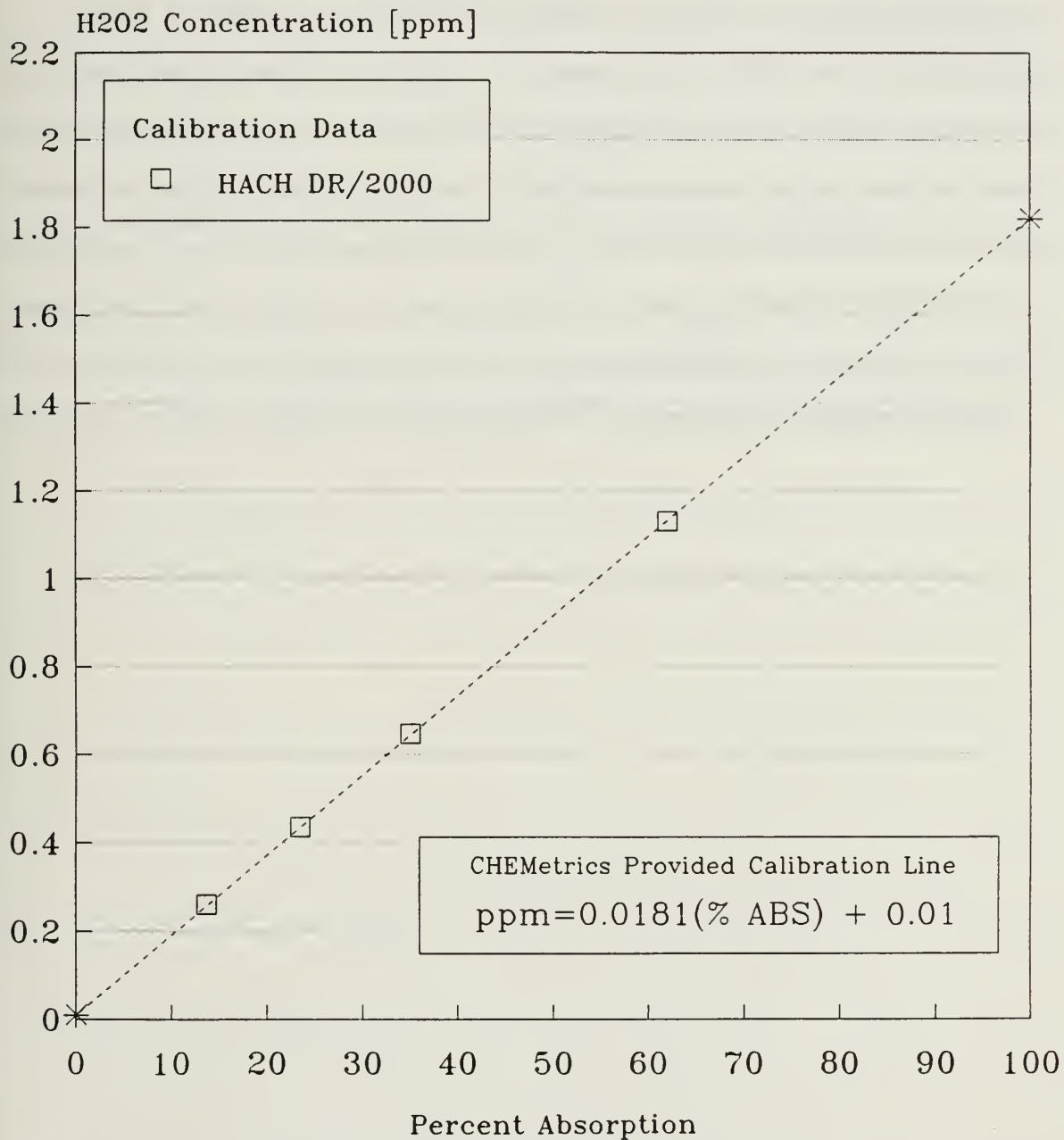
Figure A.2: HACH Spectrophotometer Calibration Curve
