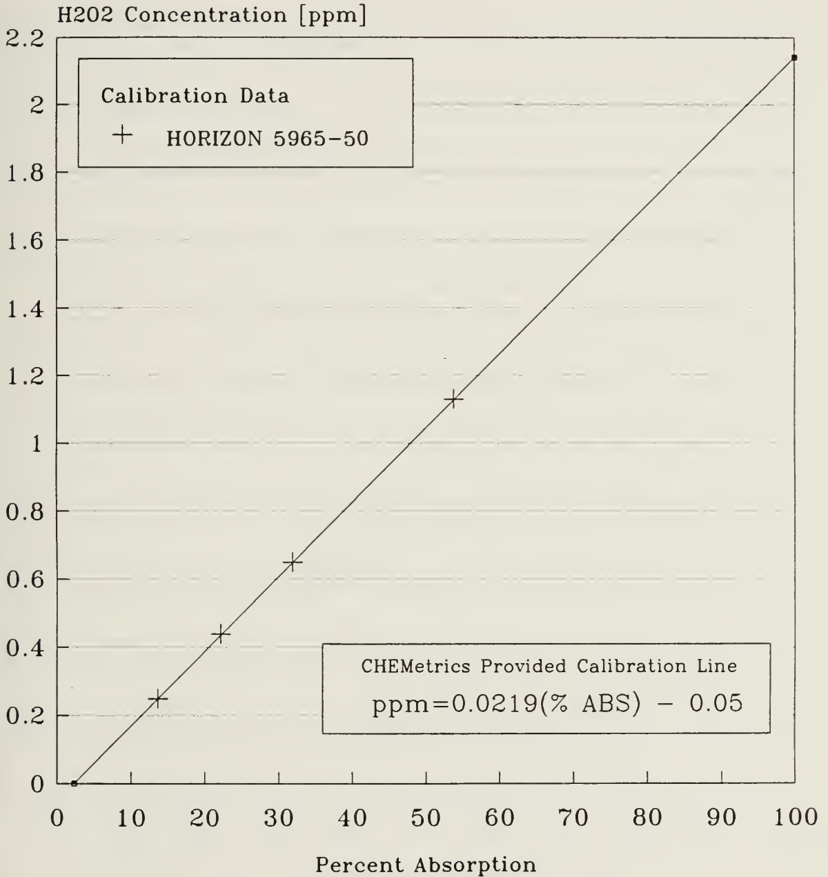
Figure A.1: HORIZON Colorimeter Calibration Curve
