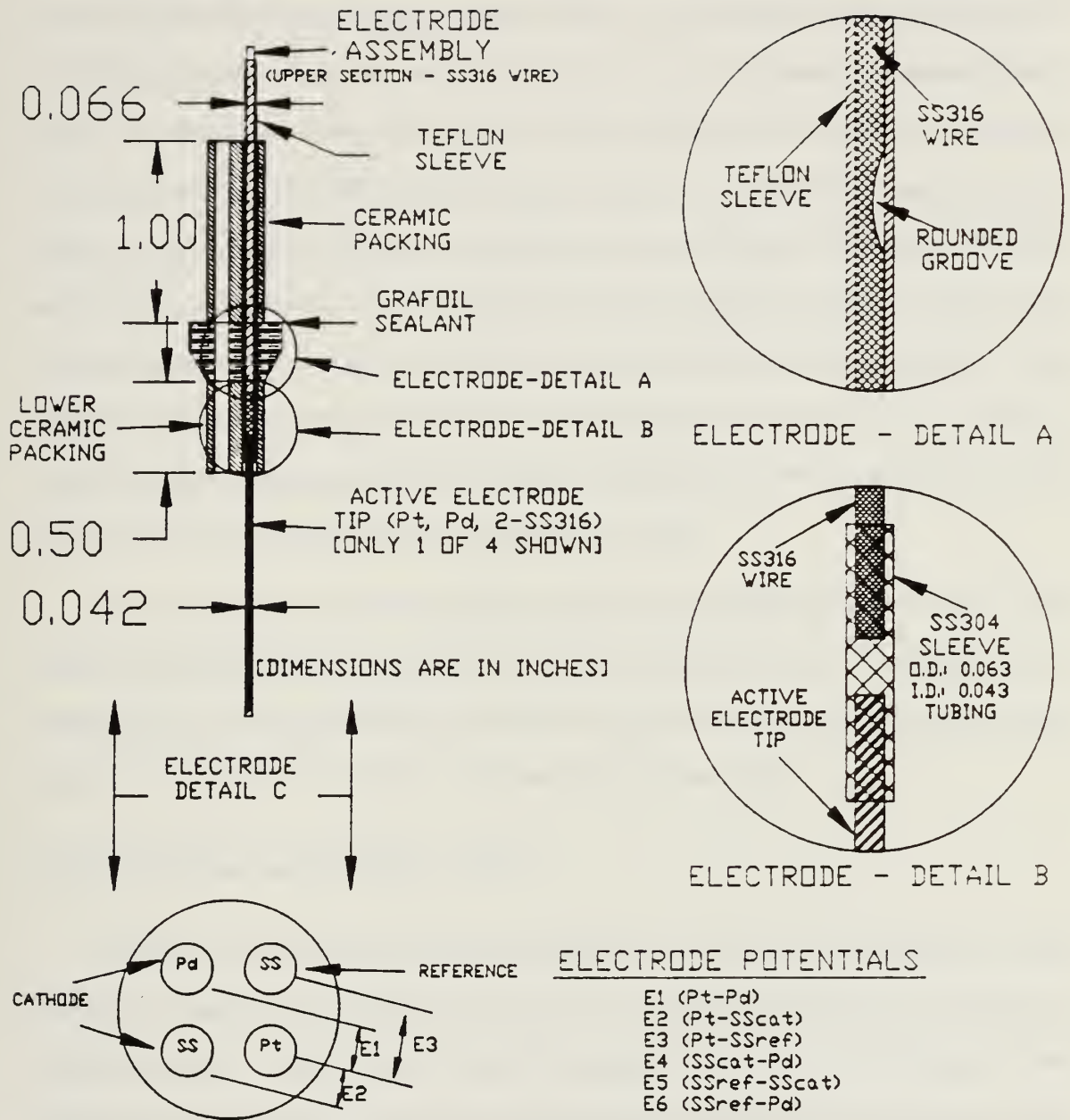
FIGURE 4.2: ELECTRODE CONFIGURATION FOR BENCH-TOP TESTING
