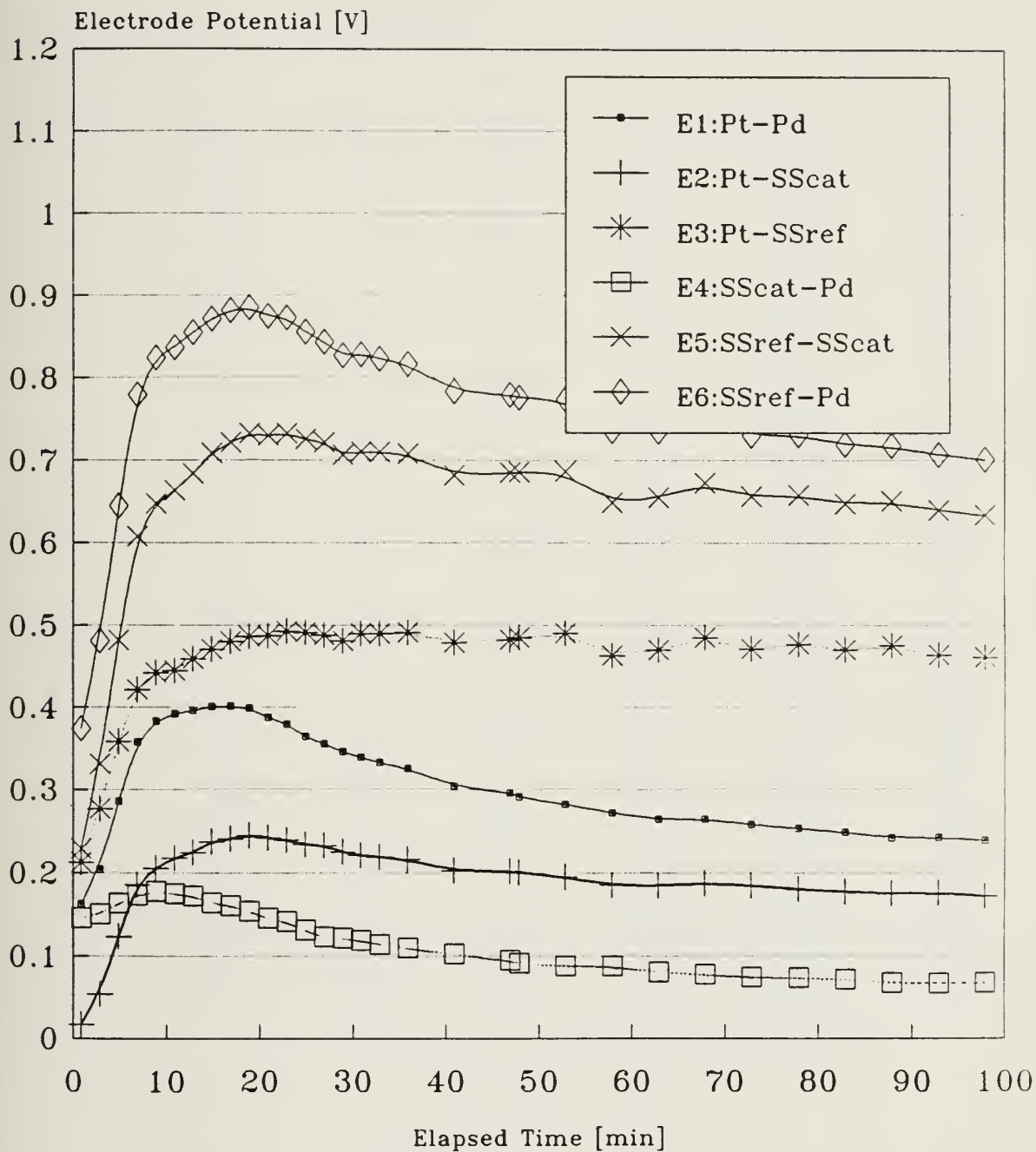
Figure C.4: Hot Reference Run #4
