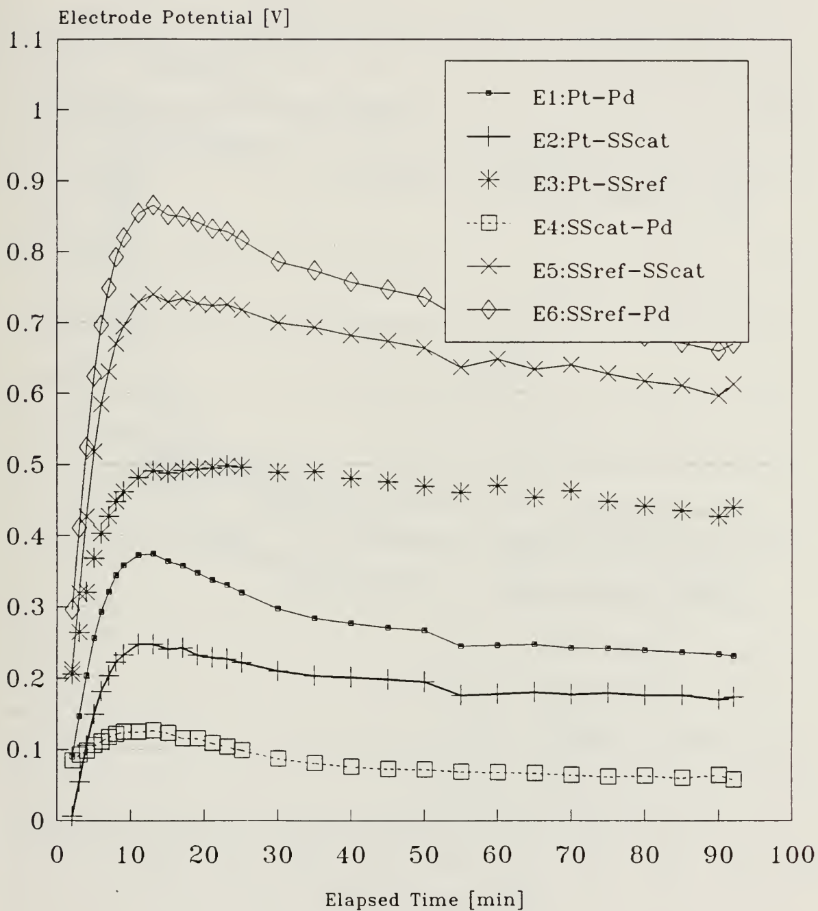
Figure 4.6: Hot Reference Run #3
