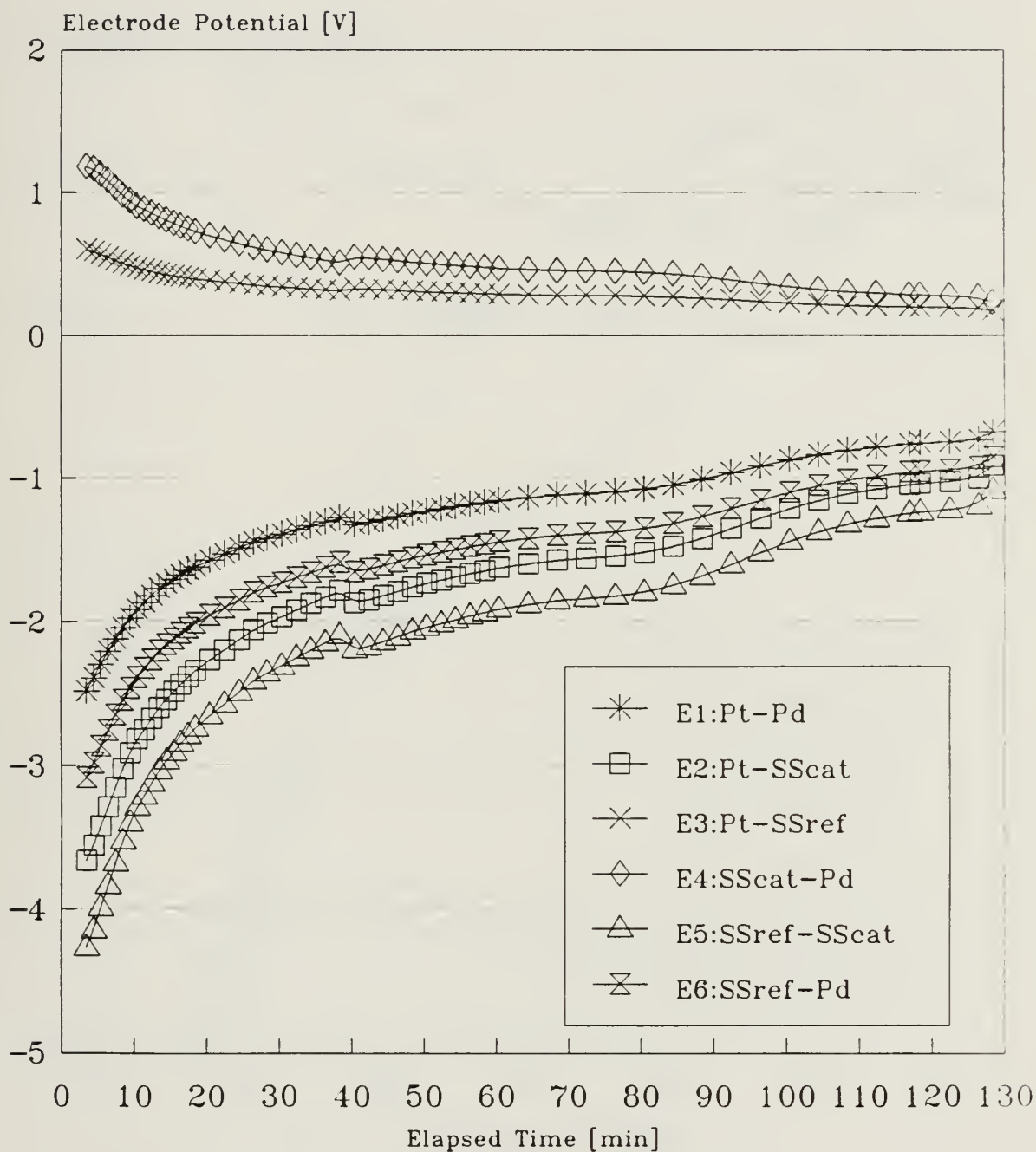
Figure 4.3: Cold Reference Run #1
