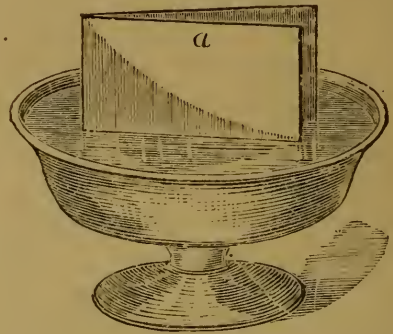
Capillary attraction between two panes of glass.
