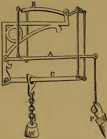
Compound levers.
