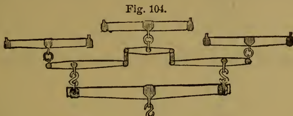
Whipple-tree for three horses.
