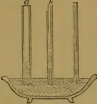
Capillary attraction in tubes.
