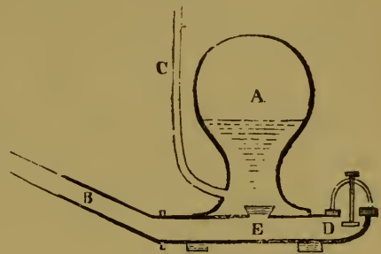
Water-ram.
