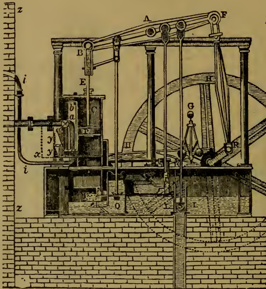
Low-pressure Steam-engine.
