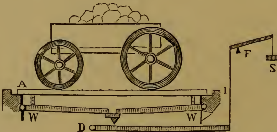
Weighing Machine.
