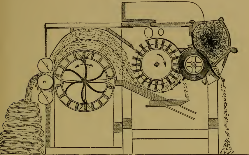
Emery's Cotton Gin, with Condenser.
