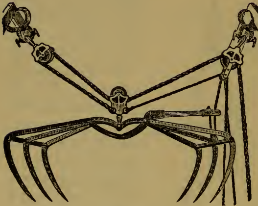
Raymond's Fork.
