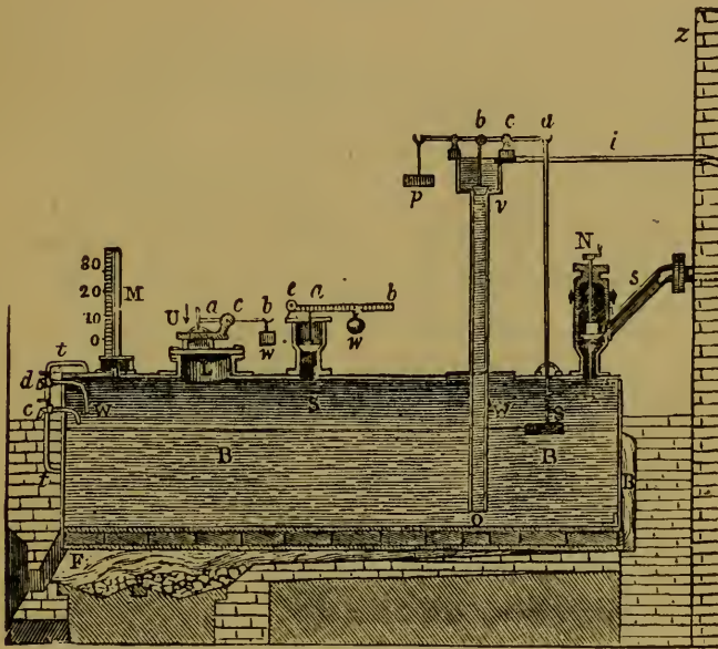
Boiler of Steam-engine.
