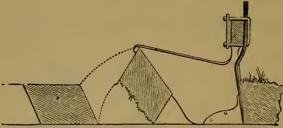
The Inclined Cutter, Laying Flat Furrows.
