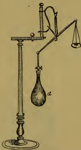
Balance for Weighing Air.
