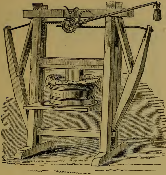
Kendall's Cheese-press.
