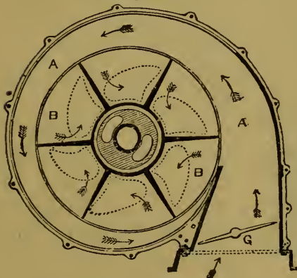
Section of Reynolds' Wheel.
