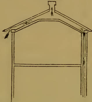
Mode of Ventilating Half-story Bed-rooms.
