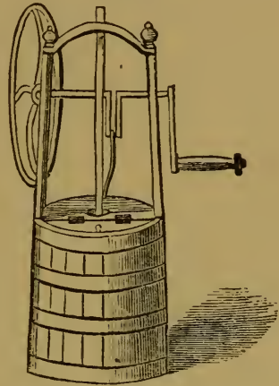
Churn with a fly-wheel, for equalizing the motion.
