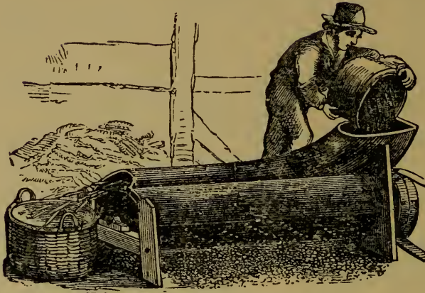
Horse-power Corn Sheller.
