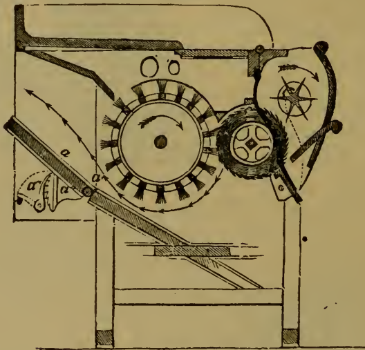
Emery's Cotton Gin—Section.
