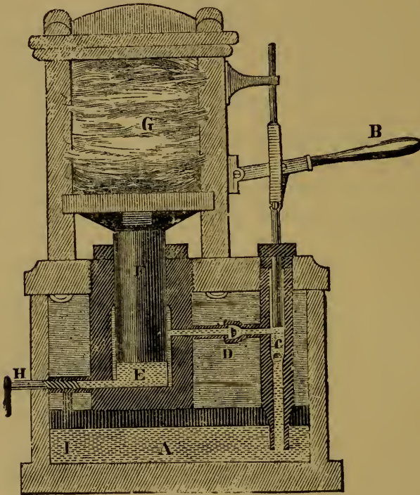
Hydrostatic Press.
