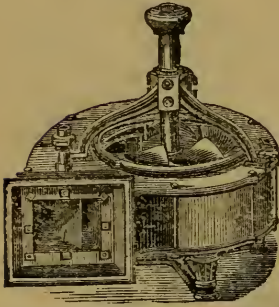
View of Reynolds' Turbine Wheel.
