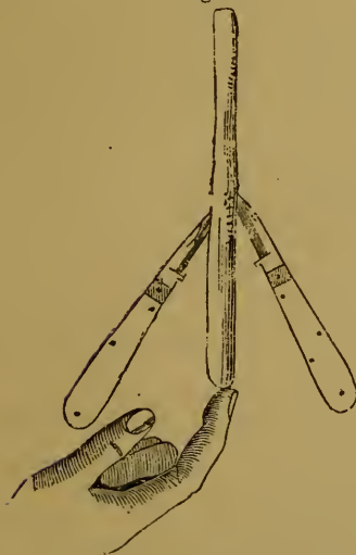
Centre of gravity maintained by two penknives.
