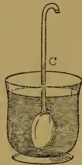
Apparatus explaining the rising of sap.
