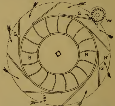
Section of Van de Water Wheel, buckets separate.
