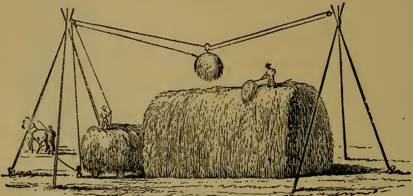
Fork on Poles for Building Stacks.
