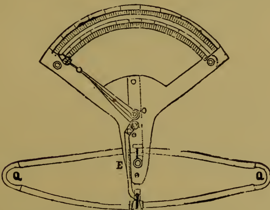
Elliptic Dynamometer.
