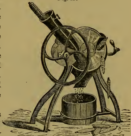
Burrall's Corn Sheller.
