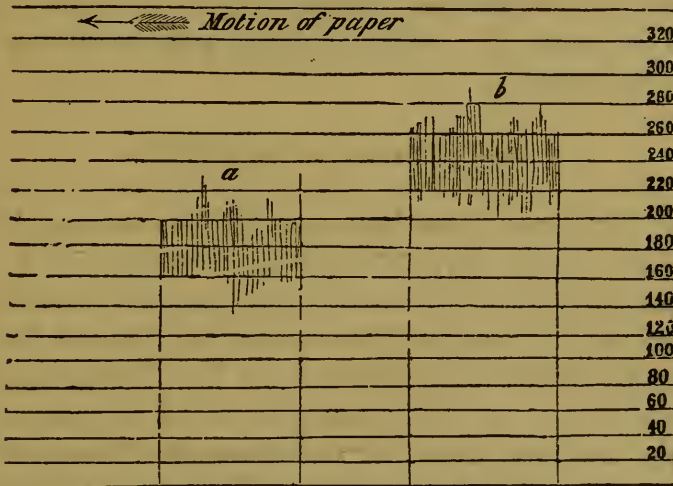
The markings of the Self-recording Dynamometer .
