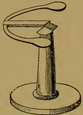
Body singularly balanced by lead knobs.
