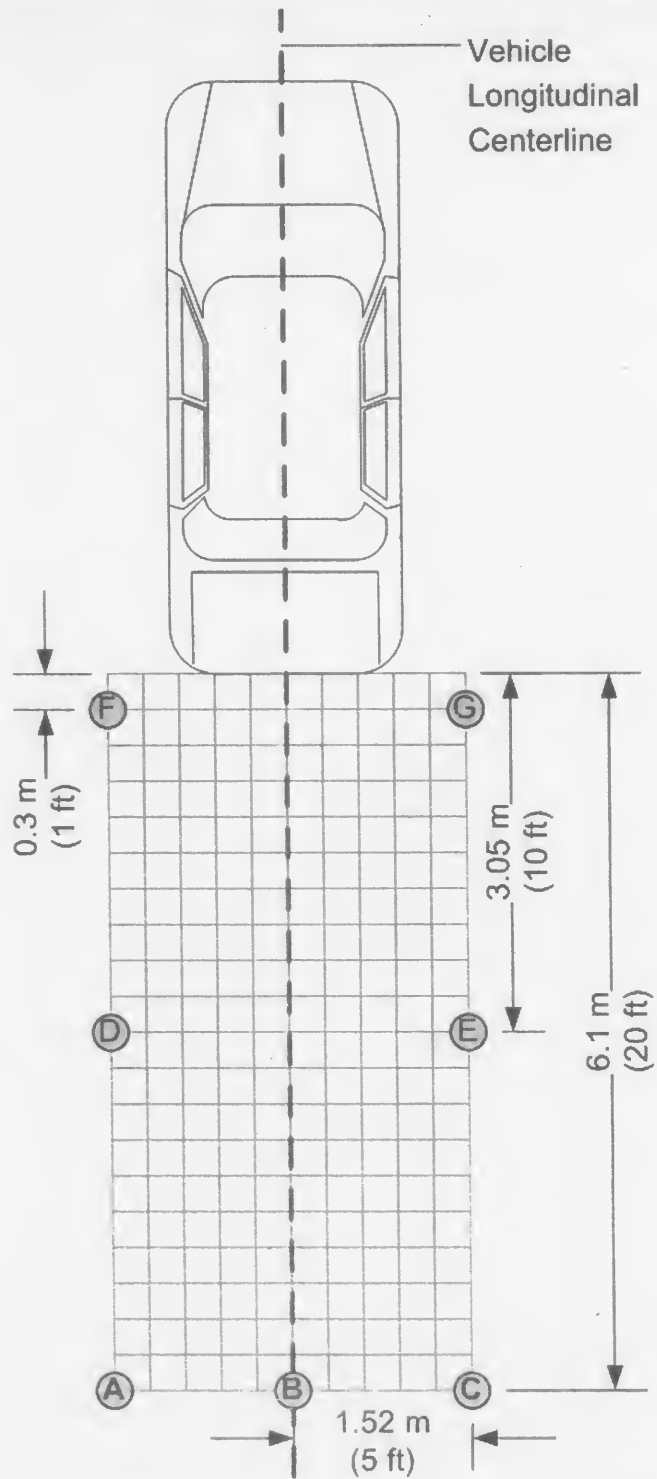
FIGURE 5: TEST CYLINDER LOCATIONS (Units in meters)
