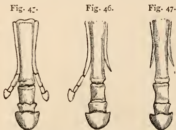
Fig. 45.—The manus of Hipparion with three functional toes. Fig. 46.—The manus of a horse with the medial digit functional. After Marsh.
