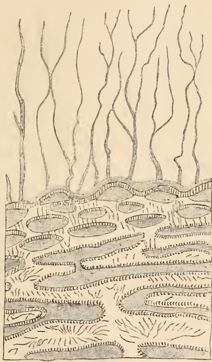
Fig. 42.—Dawson's Restoration of Eozoon.
