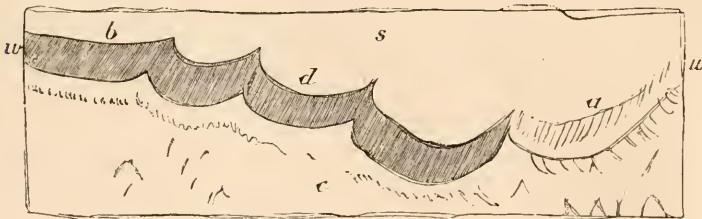
Fig. 50.—Specimen from Grenville, after King and Rowney. c , calcite; s , serpentine; w , asbestiform layer or proper wall, with the fibrous structure completely developed in places ( d ), but in an incipient stage of development at a and b ; the latter shows that the layer is an integral part of the serpentine.
