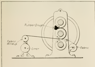
CALENDERING THE FABRIC.
