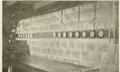
FOOTWEAR VULCANIZER EQUIPPED WITH RECORDING THERMOMETERS.
