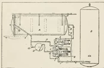
FOOTWEAR VULCANIZER.
