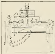
FABRIC TESTER.
