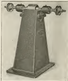
TIRE-BUFFING STAND.
