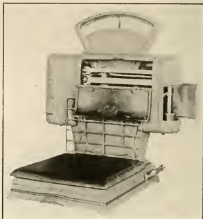
COMPOUNDING SCALE.
