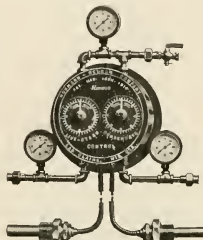
AIR-OPERATED CONTROLLER.
