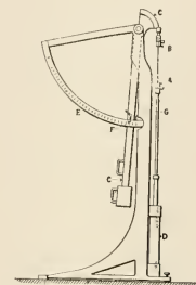
FIG. 2.—SCHOFFER FABRIC-TESTING MACHINES, INCLINATION BALANCE TYPE.
