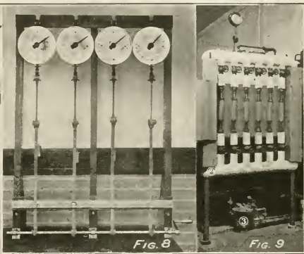
FIG. 8. APPARATUS FOR DETERMINING THE SET.
