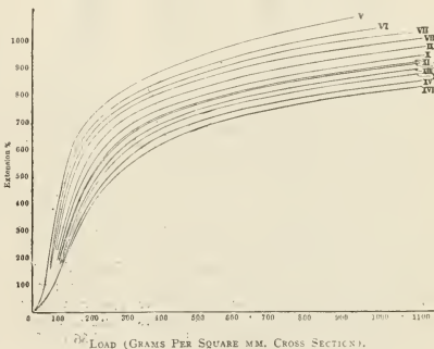
FIG. 1. STRESS-STRAIN CURVES REPRESENTING SUCCESSIVE CURES OF ONE MIXING AT 15-MINUTE INTERVALS (e. g., V = 75 MINUTES, VI = 90 MINUTES, ETC.) IN STEAM AT 286 DEGREES F.
