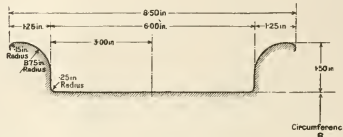
SECTION S.S. 40 ins. x 8 ins.
