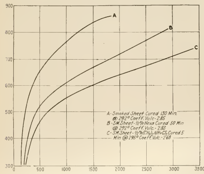
FIG. 1. STRESS-STRAIN CURVES.
