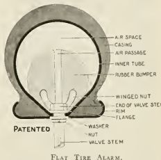
FLAT TIRE ALARM.
