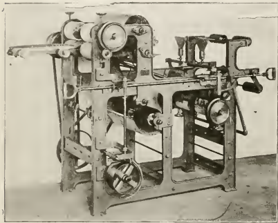
FIG. 4. KNAPP SINGEING MACHINE.
