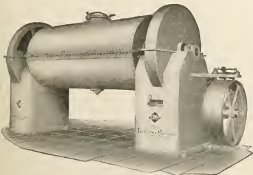
THE EIMCO CEMENT CHURN.
