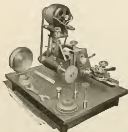
UNIVERSAL TOOL GRINDER.
