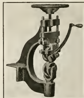
TREAD ROLLING MACHINE.
