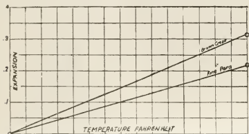
FIG. 2. CURVE SHOWING EFFECT OF RUBBER ON RATE OF EXPANSION 1698 FINE PARÁ 29, 1698 BROWN CRÉPE.
