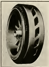
THE "MONOTWIN" TIRE.
