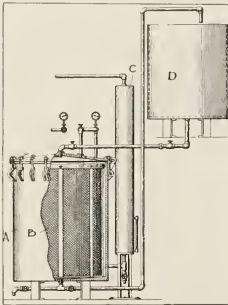
FELT IMPREGNATOR.
