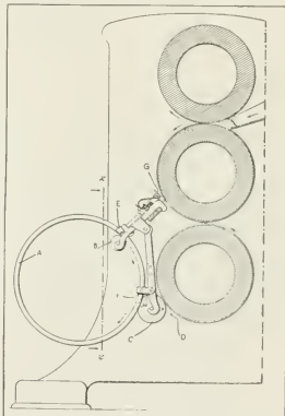
SOLID-TIRE-BUILDING MACHINE.
