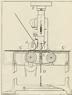
FIG. 1. ELEVATION PARTLY IN SECTION AT RIGHT ANGLE TO THE PLANE OF FIG. 2.
