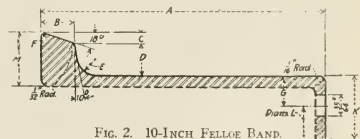
FIG. 2. 10-INCH FELLOE BAND.
