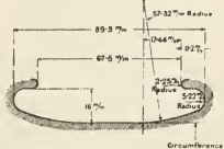
SECTION 820 AND 880 B.E.
