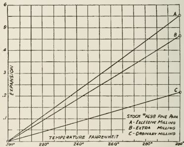
FIG. 3. CURVE SHOWING EFFECT OF MILLING ON RATE OF EXPANSION.
