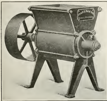
DAY HERCULES CRUSHER.
