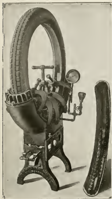
CAVITY RETREAD MOLD.
