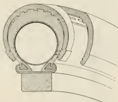
"MULLIKIN" OVERSHOE TIRE.
