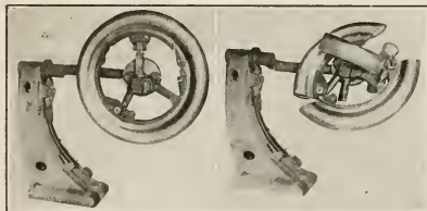
BUILDING STAND.
