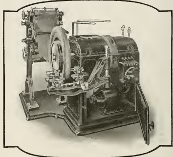
HERMAN SPECIAL TIRE BUILDER.
