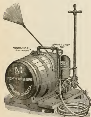
HAND-POWER SPRAYER.
