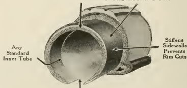
Extends to Base of Rim—Prevents Rim Blow Outs
