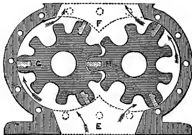
FIG. 124.—Rotary Pump.
