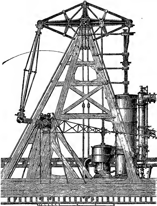
FIG. 180.—Beam-Engine.
