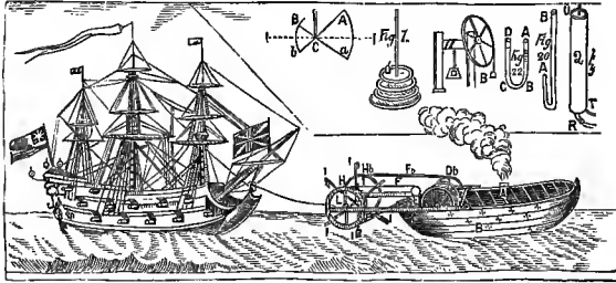
FIG. 66.—Hulls's Steamboat, 1786.
