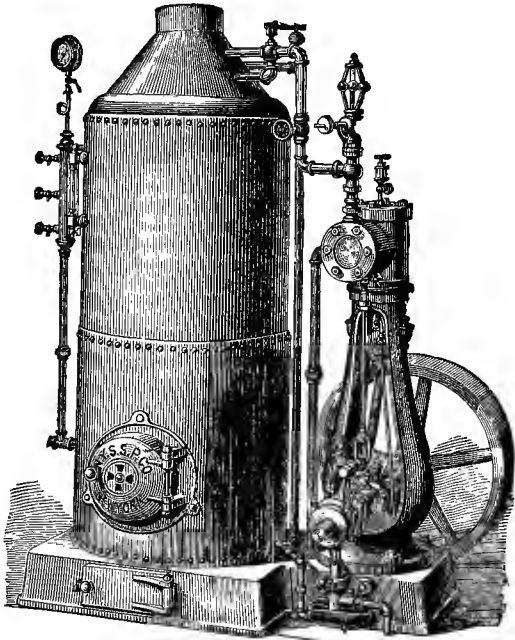
FIG. 114.—Semi-Portable Engine, 1878.
