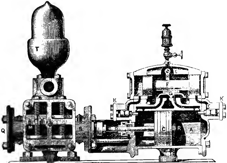
FIG. 102.—Steam-Pump.
