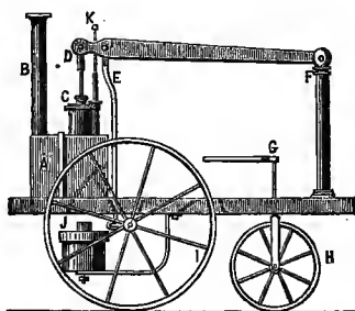
FIG. 45.—Murdoch's Model, 1784.
