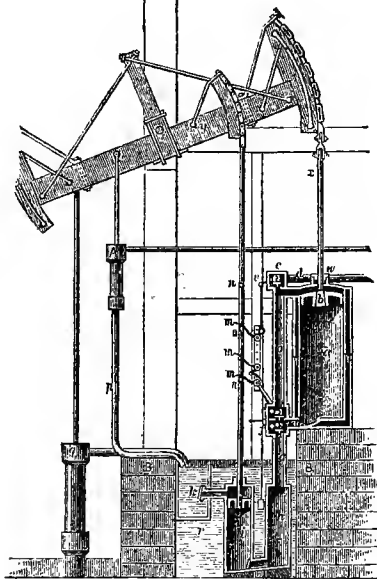
FIG. 26.—Watt's Engine, 1774.
