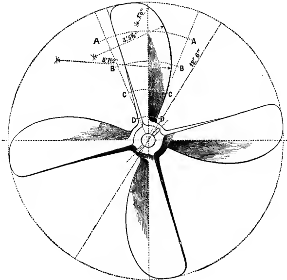
FIG. 139.—Screw-Propeller.
