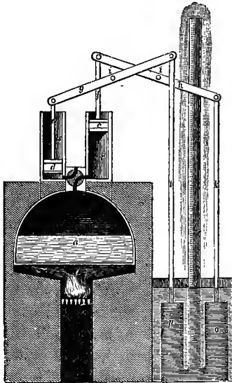
FIG. 41.—Leupold's Engine, 1720.
