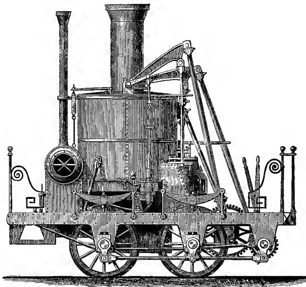
FIG. 59.—The "Atlantic," 1832.
