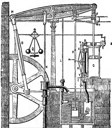
FIG. 81.—Boulton & Watt's Double-Acting Engine, 1784.
