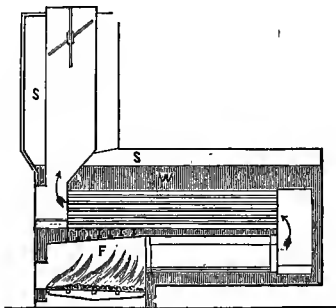
FIG. 89.—Stevens's Return Tubular Boiler, 1832.
