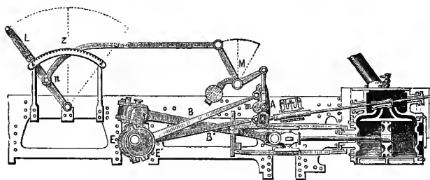
FIG. 53.—The Stephenson Valve-Gear, 1833.
