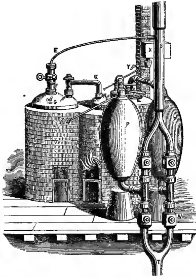
FIG. 18.—Savery's Engine, A. D. 1702.
