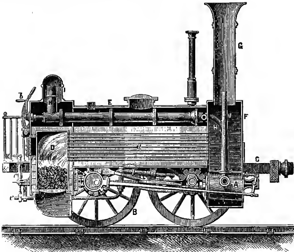
FIG. 57.—Stephenson's Locomotive, 1838.
