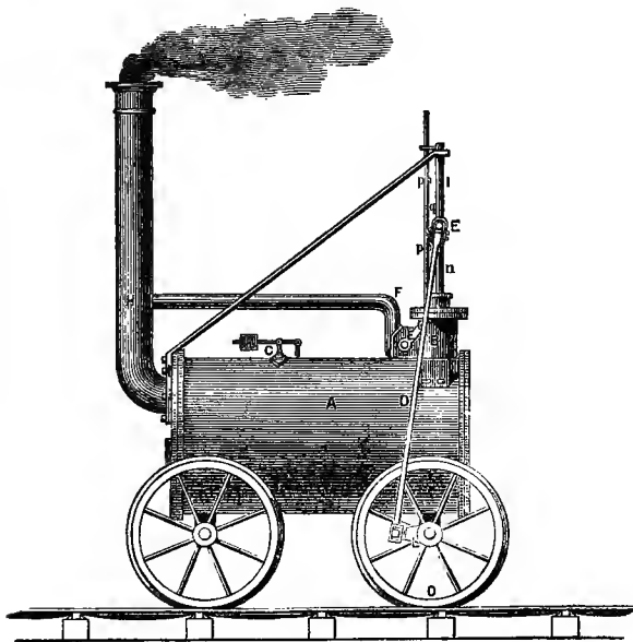
FIG. 50.—Trevithick's Locomotive, 1804.
