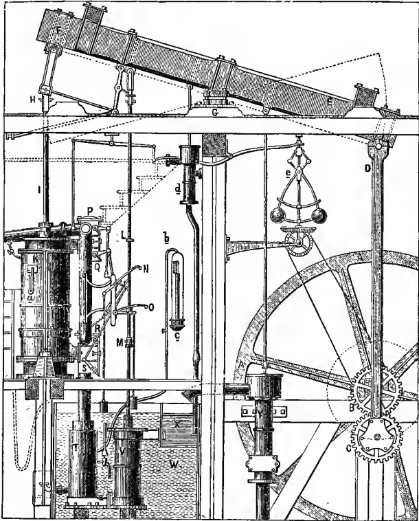
FIG. 27.—Watt's Engine, 1781.
