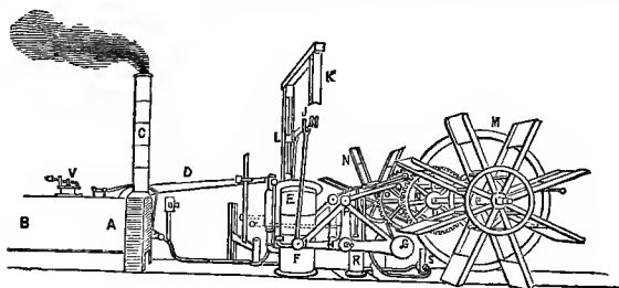
FIG. 81.—Engine of the Clermont, 1808.
