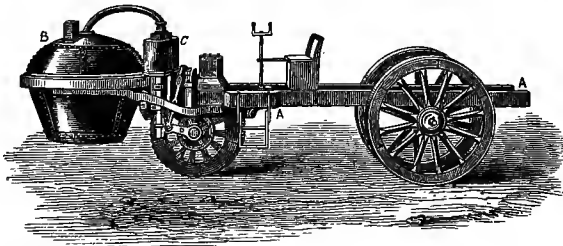
FIG. 44.—Cugnot's Steam-Carriage, 1770.
