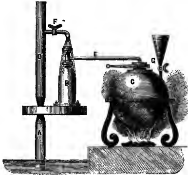
FIG. 12.—Savery's Engine, 1698.
