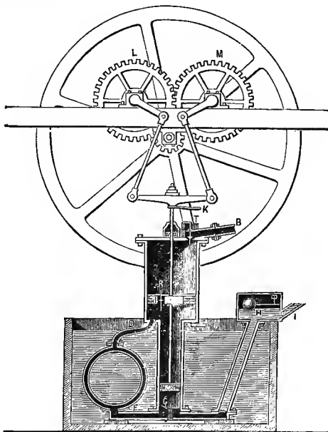
FIG. 39.—Cartwright's Engine, 1798.
