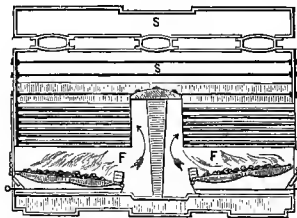
FIG. 143.—Marine High-Pressure Boiler. Section,
