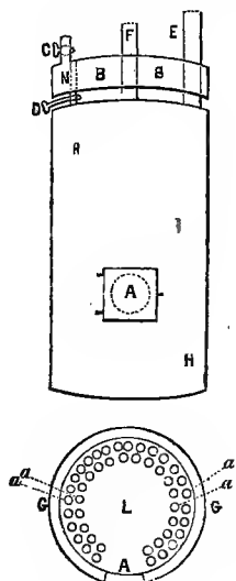
FIG. 74.—Read's Multi-Tubular Boiler, 1788.
