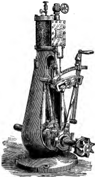
FIG. 135.—Launch-Engine.
