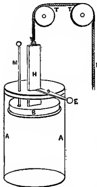
FIG. 17.—Papin's Engine.
