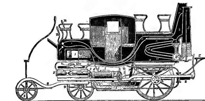
FIG. 48.—Gurney's Steam-Carriage.
