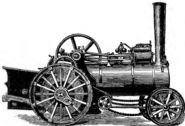
FIG. 119.—Road and Farm Locomotive.
