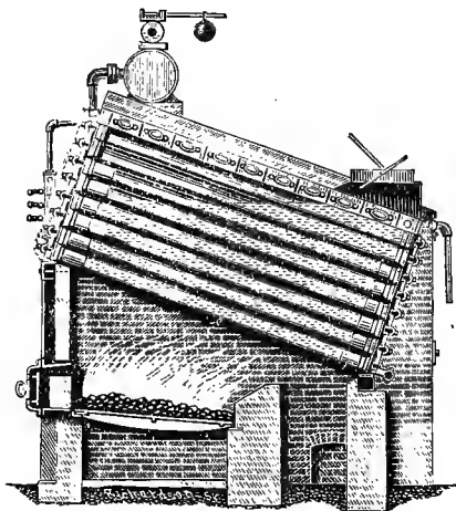
FIG. 118.—Root Sectional Boiler.
