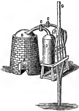
FIG. 11.—Savery's Model, 1698.
