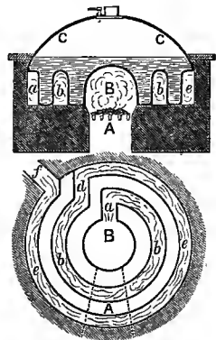
FIG. 22.—Boiler of Newcomen's Engine, 1768.
