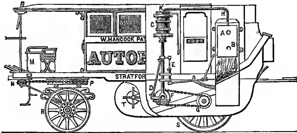
FIG. 49.—Hancock's "Autopsy," 1838.
