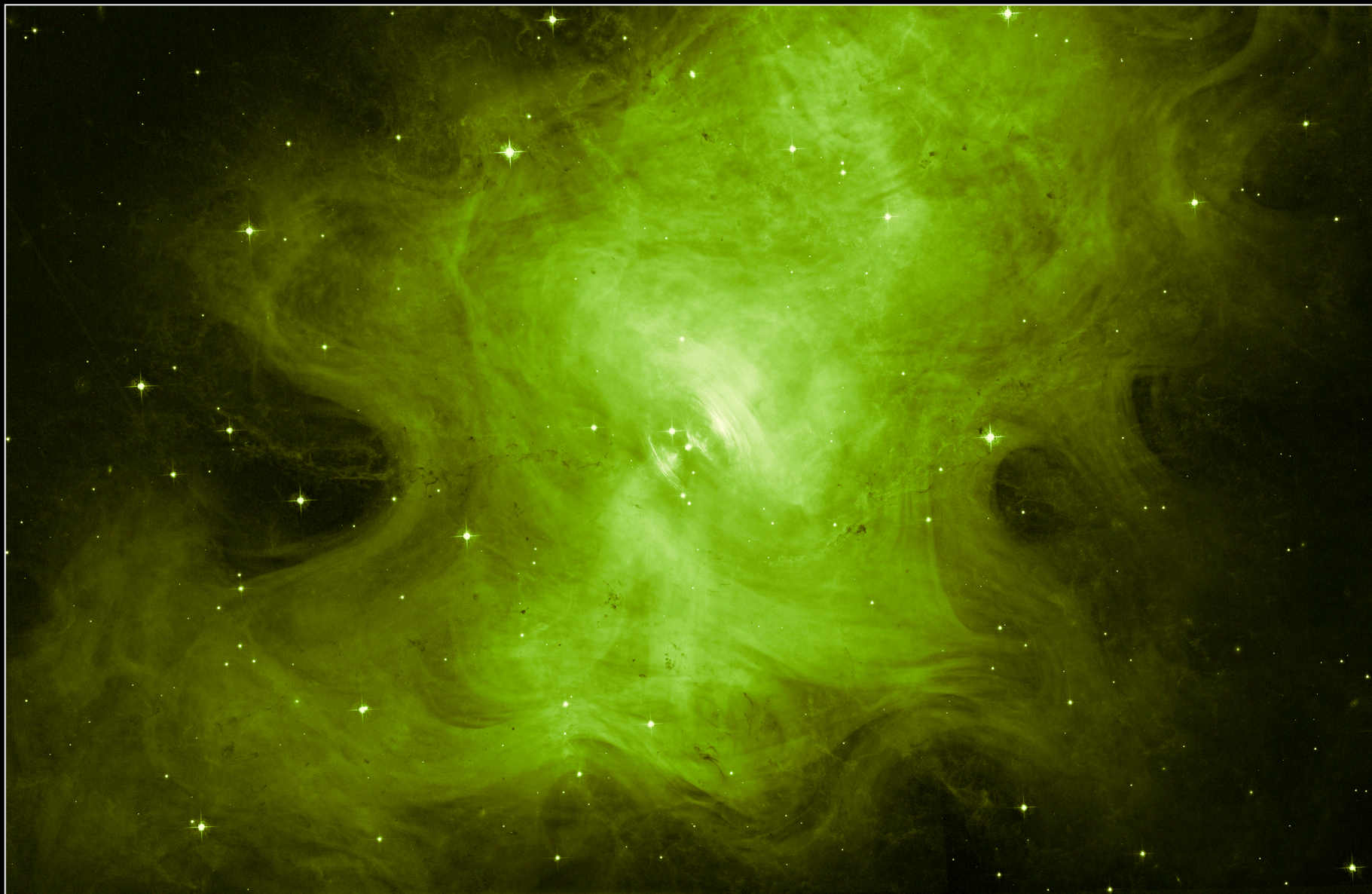
Crab Nebula ■ M1 Hubble Space Telescope ■ ACS/WFC
