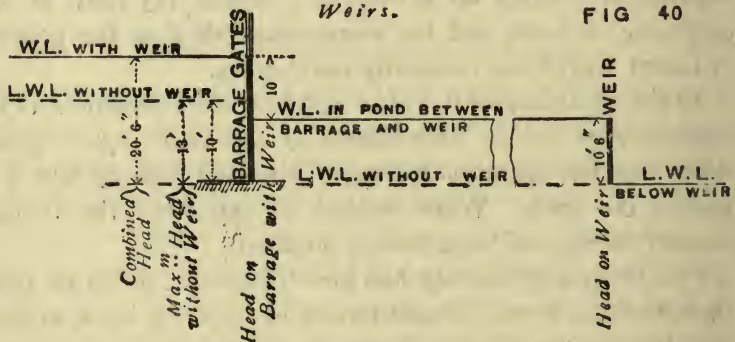
OF WATER LEVELS AT THE DELTA BARRAGE before and after construction of the Weirs.
