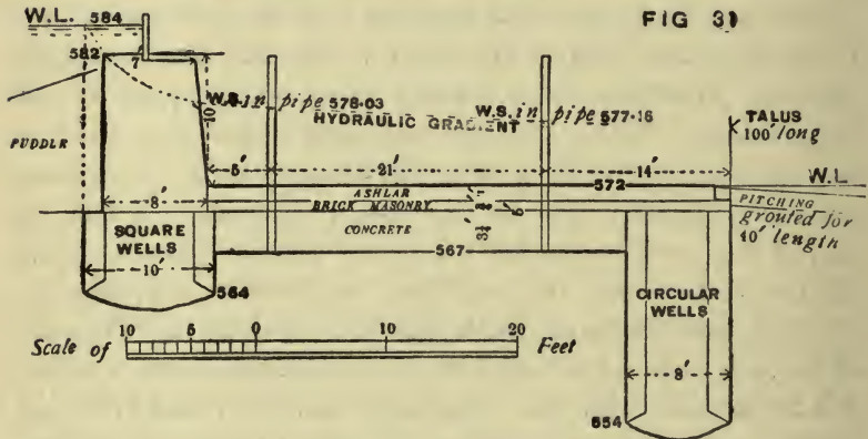
NARORA WEIR SHOWING OBSERVATION PIPES
