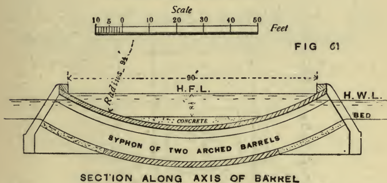
SECTION ALONG AXIS OF BARREL
