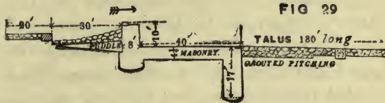
AS STRENGTHENED
