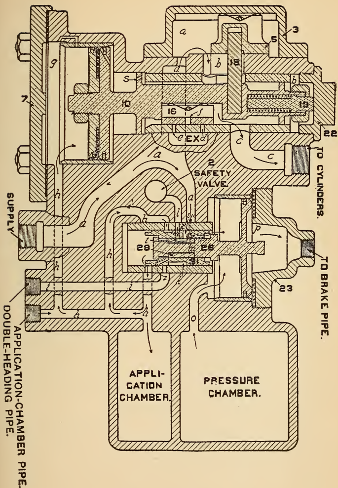
FIG. 304. EMERGENCY
