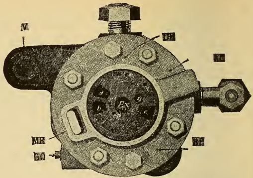
ROTARY-VALVE SEAT.
