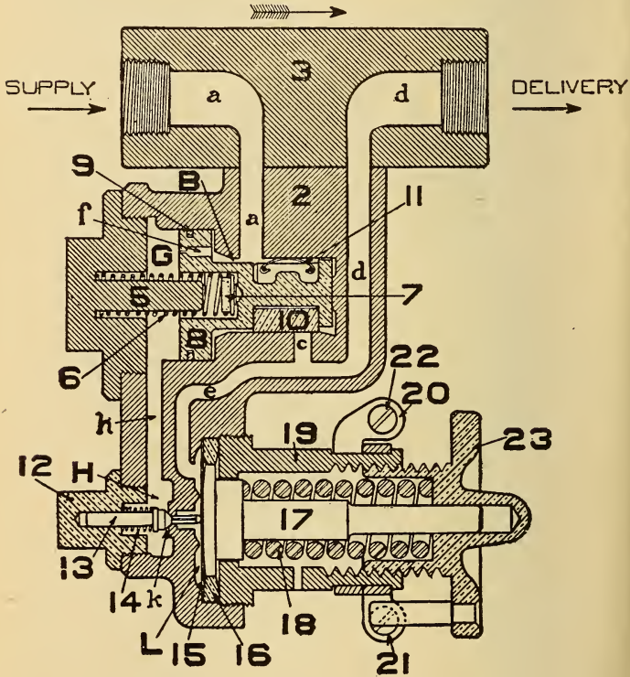
FIG. 318. DIAGRAM OF FEED VALVE, CLOSED
