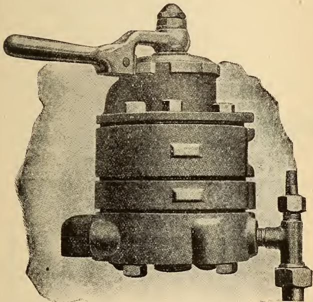
FIG. 310. TYPE H BRAKE VALVE
