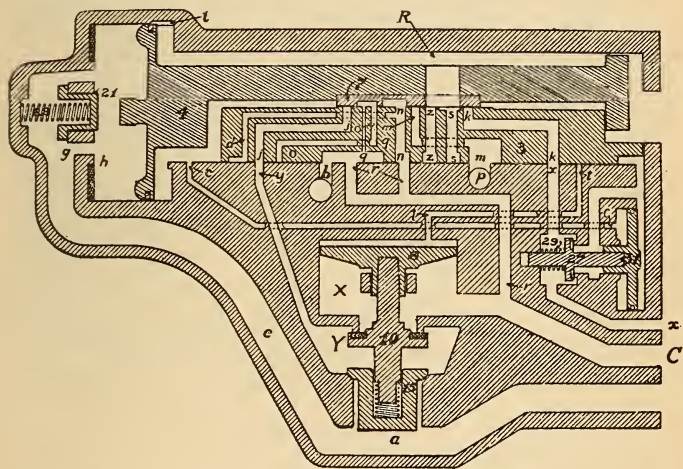
FIG. 355. GRADUATED-RELEASE-LAP POSITION
