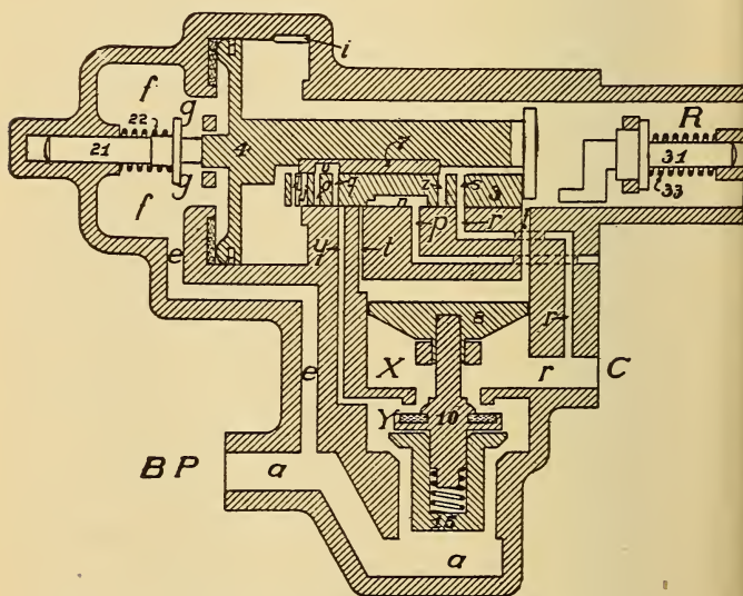
FIG. 331. EMERGENCY POSITION
