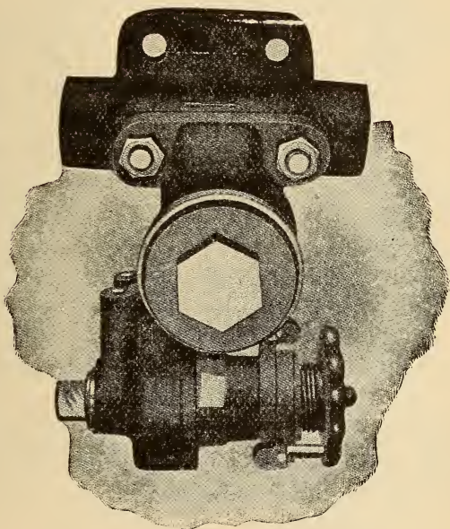
FIG. 317. FEED VALVE
