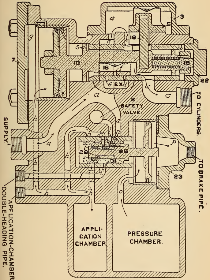
FIG. 302. AUTOMATIC SERVICE
