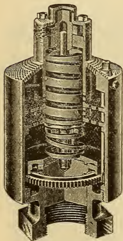
FIGURE 190 CRANE POP VALVE, SECTIONAL VIEW
