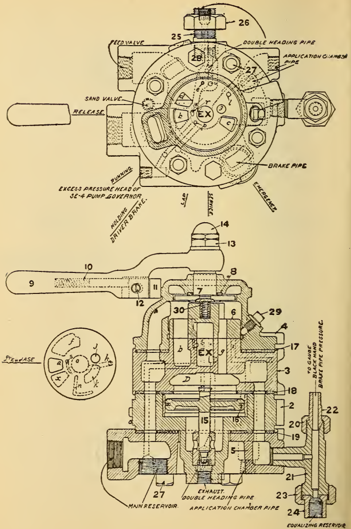
FIG. 313. AUTOMATIC BRAKE VALVE
