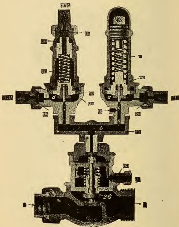
FIG. 321. PUMP GOVERNOR
