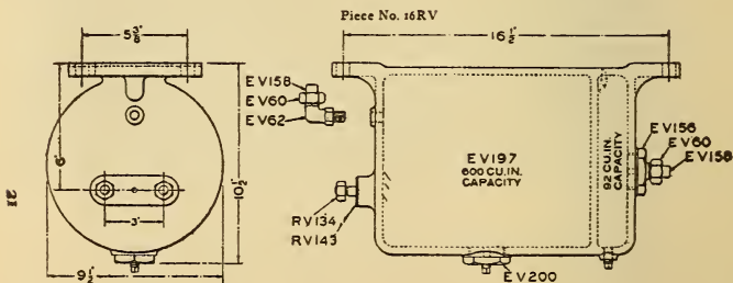
Fig. 279. Divided Reservoir.
