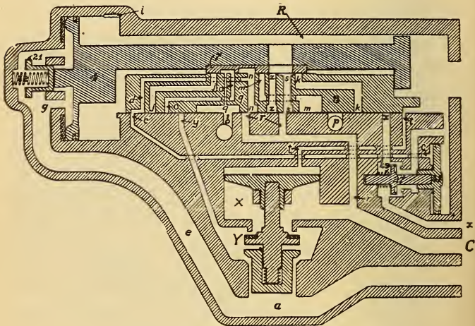
FIG. 356. EMERGENCY POSITION
