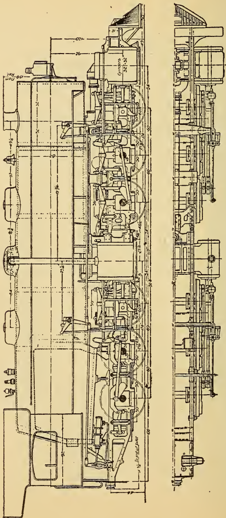
FIG. 345. WALSCHAERT VALVE GEAR—MALLET ARTICULATED COMPOUND FREIGHT LOCOMOTIVE—BALTIMORE & OHIO RAILROAD
