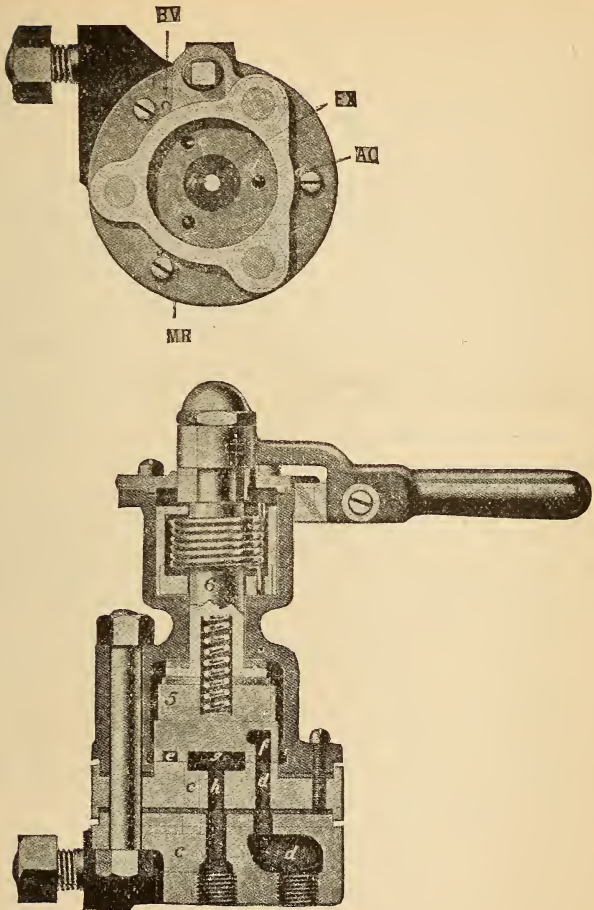
FIG. 315. INTERIOR VIEW OF THE INDEPENDENT BRAKE VALVE
