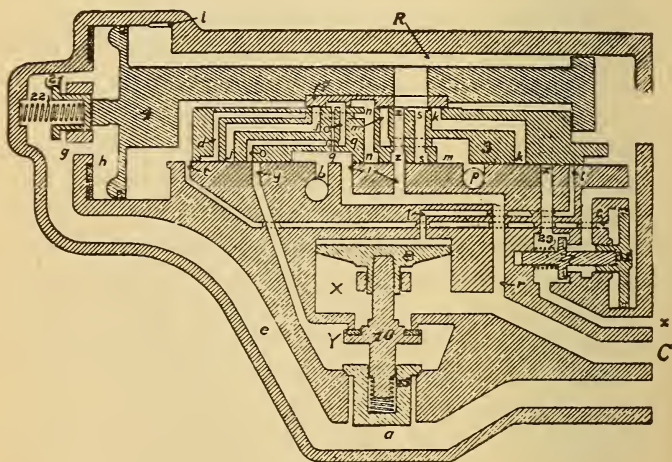
FIG. 353. FULL-SERVICE POSITION
