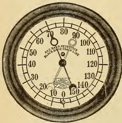
FIGURE 179 CROSBY DUPLEX GAUGE
