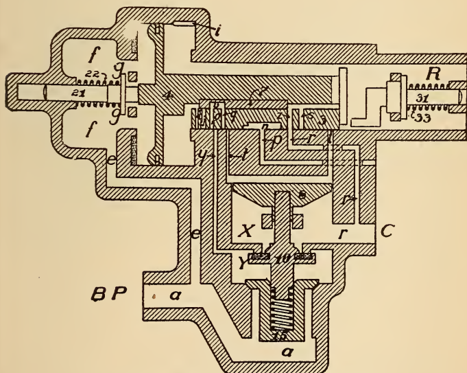
FIG. 328. FULL SERVICE POSITION
