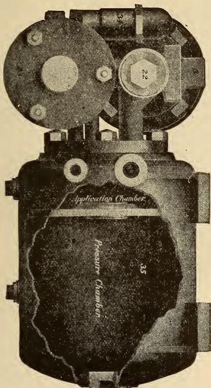
FIG. 297. DISTRIBUTING VALVE AND DOUBLE-CHAMBER RESERVOIR
