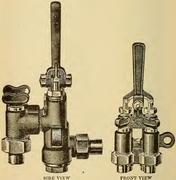
FIGURE 209 OPERATING VALVE FOR CYLINDER COCK
