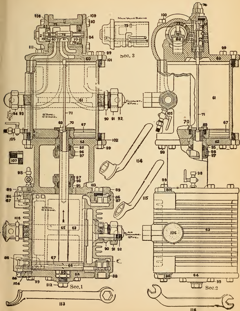
FIGURE 225 NINE AND ONE-HALF INCH PUMP — See page 520.
