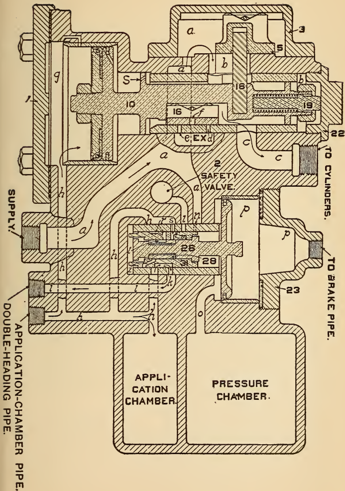
FIG. 300. INDEPENDENT APPLICATION
