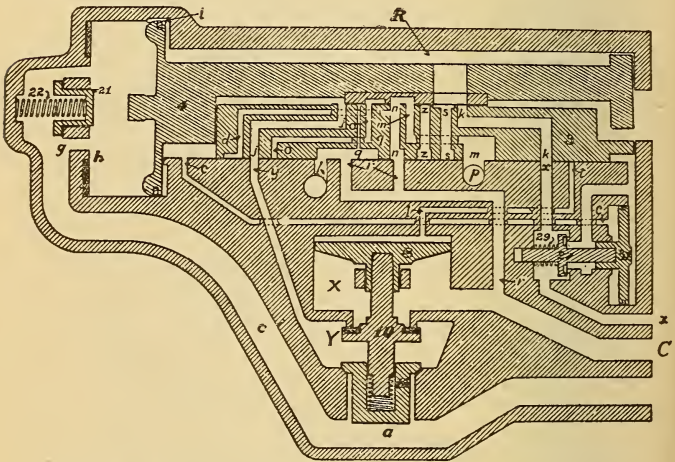
FIG. 351. FULL RELEASE AND CHARGING POSITION
