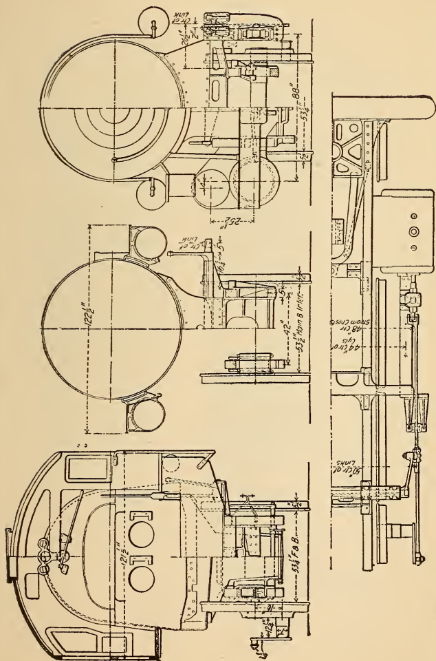
FIG. 344. WALSCHAERT VALVE GEAR—CONSOLIDATION FREIGHT LOCOMOTIVE —NEW YORK CENTRAL & HUDSON RIVER RAILROAD
