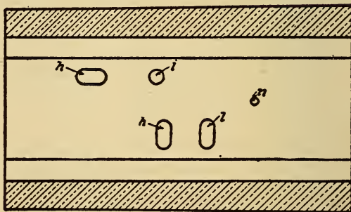
FIG. 307. GRADUATING VALVE, EQUALIZING SLIDE VALVE, AND SLIDE VALVE SEAT
