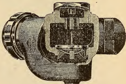
FIGURE 176 b SECTIONAL VIEW OF THE HANCOCK MAIN BOILER CHECK VALVE
