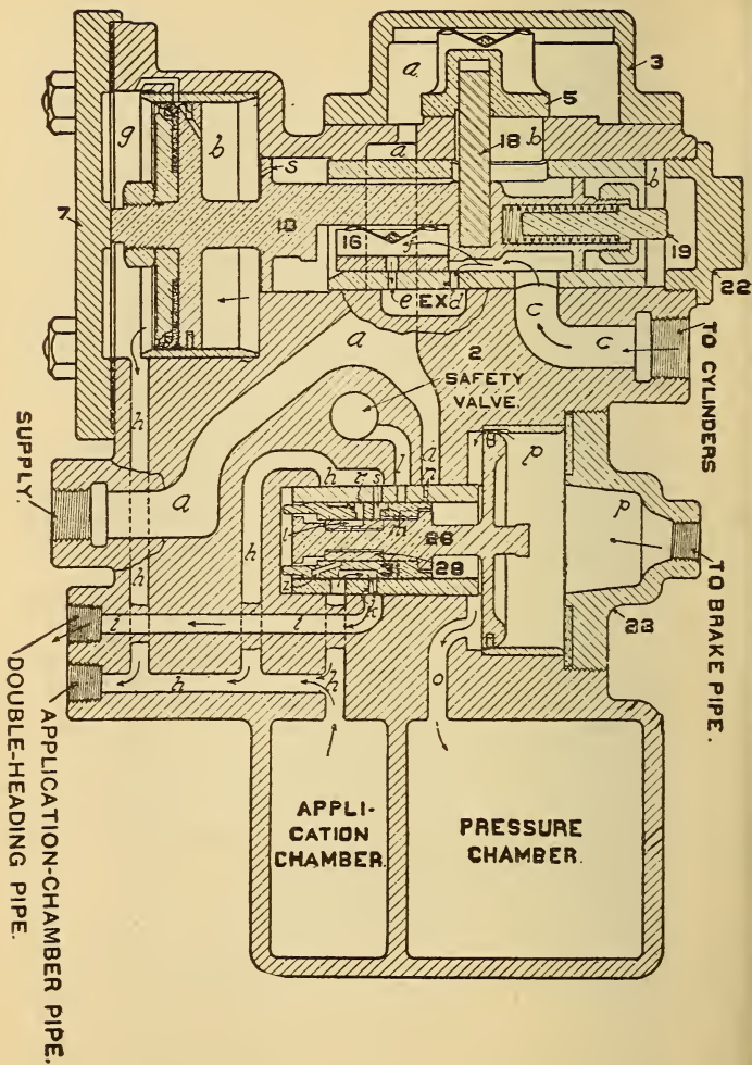
FIG. 299. RELEASE, AUTOMATIC OR INDEPENDENT
