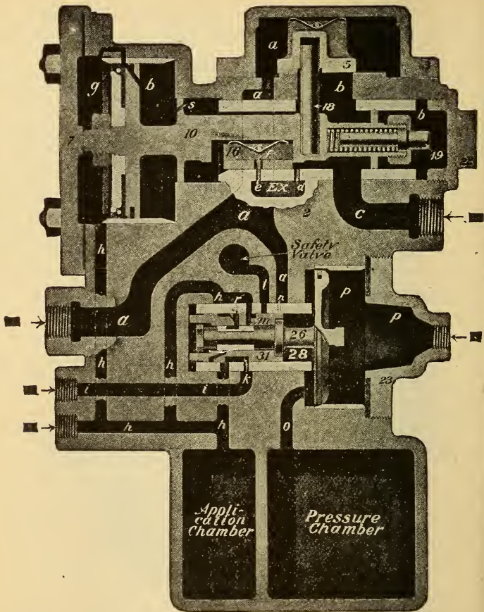
FIG. 298. THE DISTRIBUTING VALVE, DIAGRAMMATIC CONNECTIONS:
