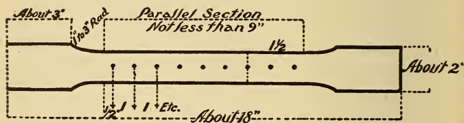
TEST PIECE
