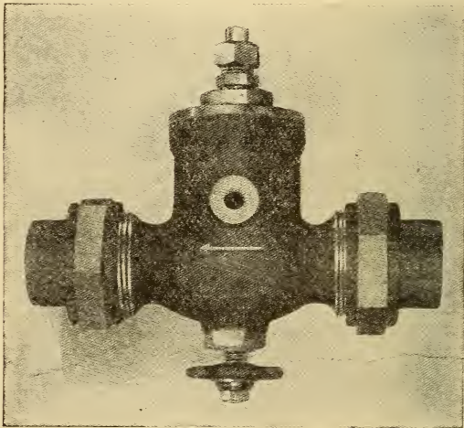
Fig. 281. Supply Portion of Pressure Controller.
