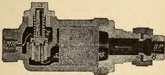
FIG. 322. COMBINED AIR STRAINER AND CHECK VALVE
