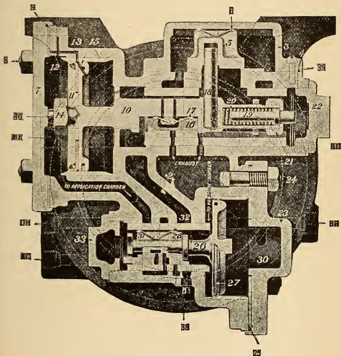
FIG. 308. DISTRIBUTING VALVE CONNECTIONS:
