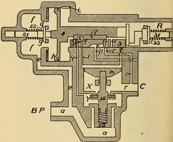
FIG. 327. QUICK SERVICE POSITION
