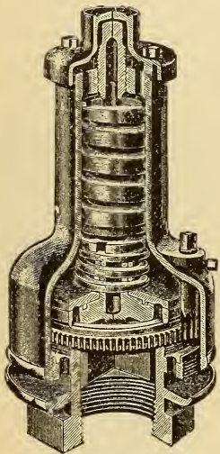
FIGURE 192 CRANE MUFFLED POP VALVE SECTIONAL VIEW
