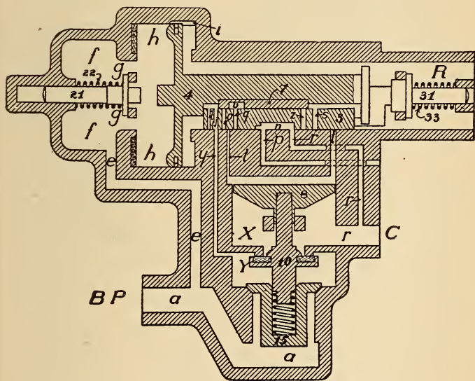
FIG. 326. FULL-RELEASE AND CHARGING POSITION
