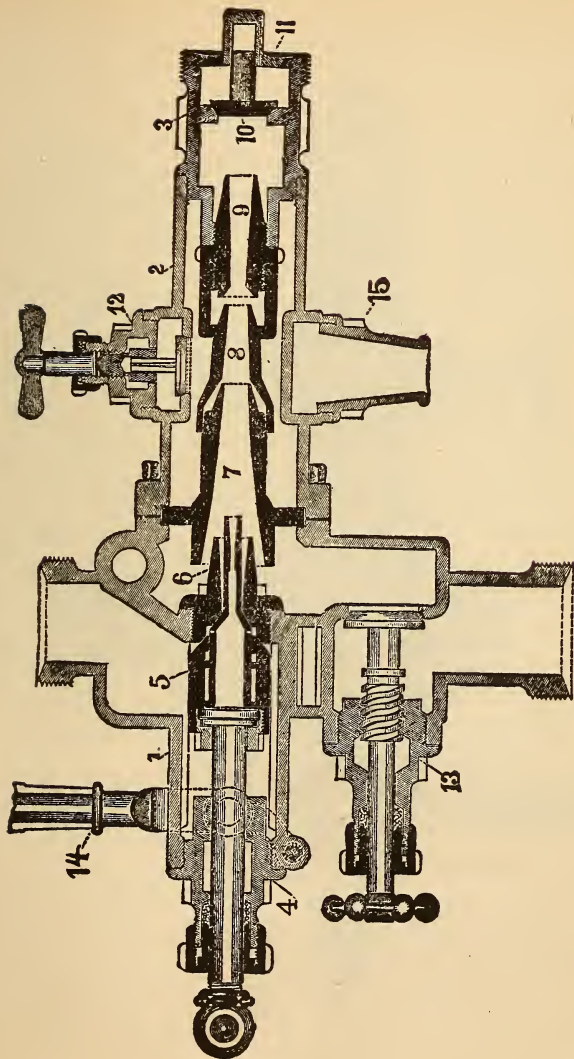
OHIO LOCOMOTIVE INJECTOR. Sectional View.
