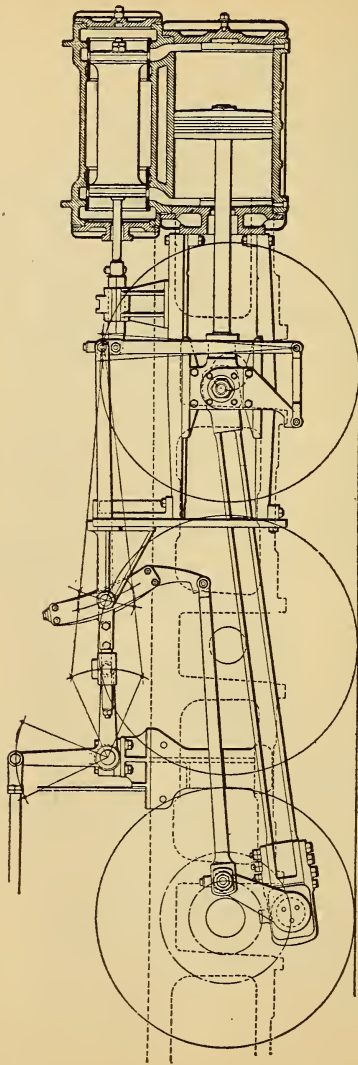
FIG. 347. WALSCHAERT VALVE GEAR AS APPLIED TO CONSOLIDATION FREIGHT LOCOMOTIVES—LAKE SHORE & MICHIGAN SOUTHERN RAILWAY
