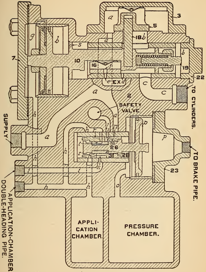
FIG. 306. RELEASE POSITION
