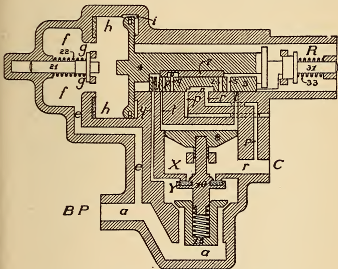
FIG. 330. RETARDED-RELEASE POSITION
