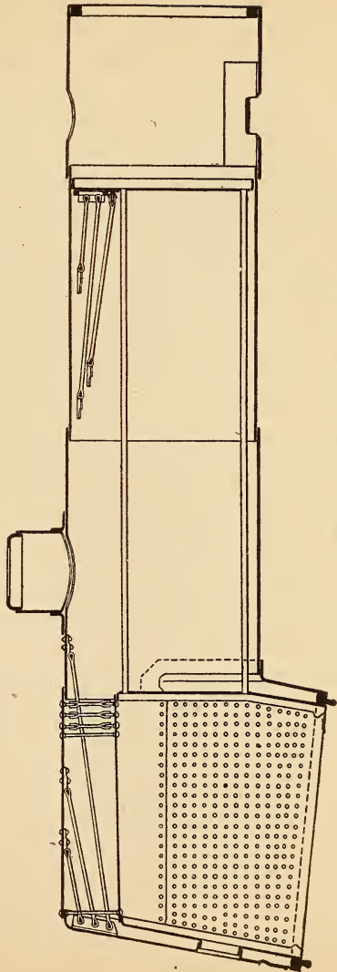
FIGURE 29. SECTION OF MODERN BOILER
