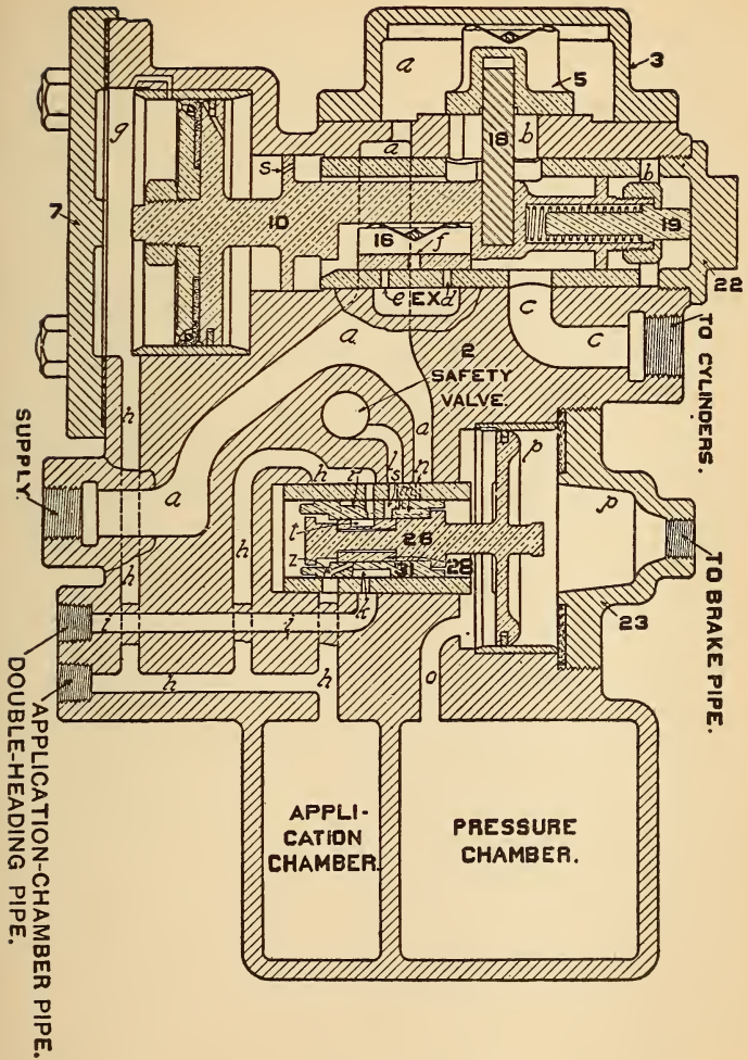
FIG. 303. SERVICE LAP
