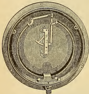
FIGURE 182 SECTIONAL VIEW AMERICAN PRESSURE GAUGE
