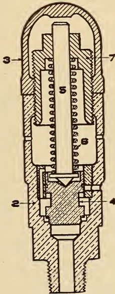
FIG. 309. SAFETY VALVE
