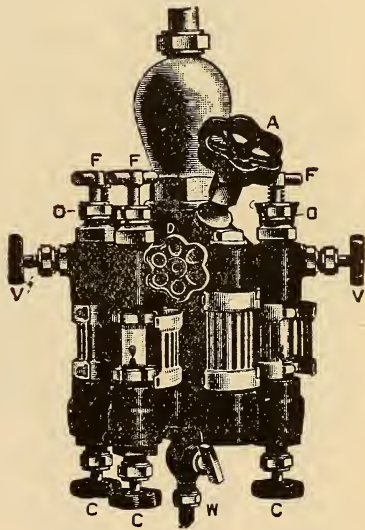
FIGURE 198 NEW NATHAN LUBRICATOR, FRONT VIEW
