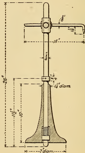
FIG. 338. A CONVENIENT GAUGE FOR SETTING THE ECCENTRIC CRANK
