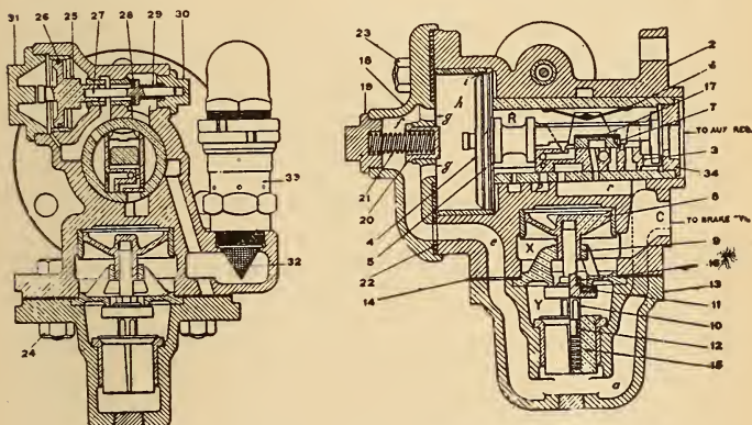
FIG. 349. THE TYPE L TRIPLE VALVE
