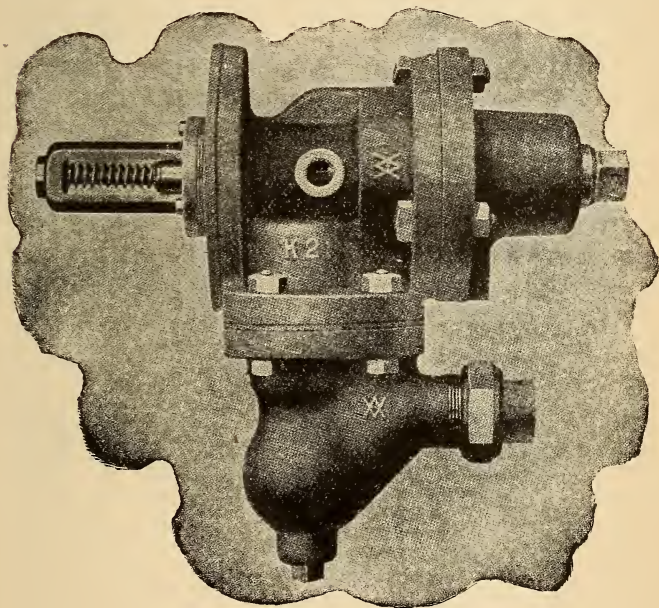
FIG. 323. THE TYPE "K" FREIGHT TRIPLE VALVE
