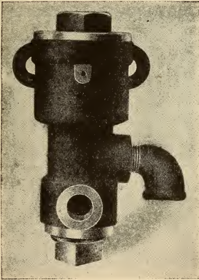
Fig. 287. Accelerator Valve.
