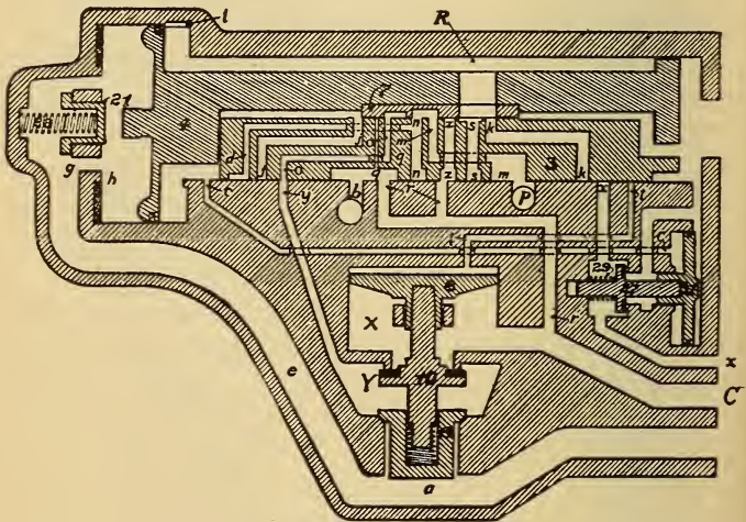
FIG. 354. SERVICE-LAP POSITION
