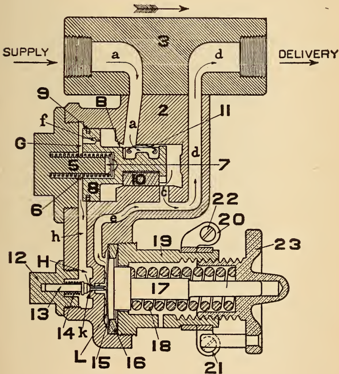
FIG. 319. DIAGRAM OF FEED VALVE, OPEN
