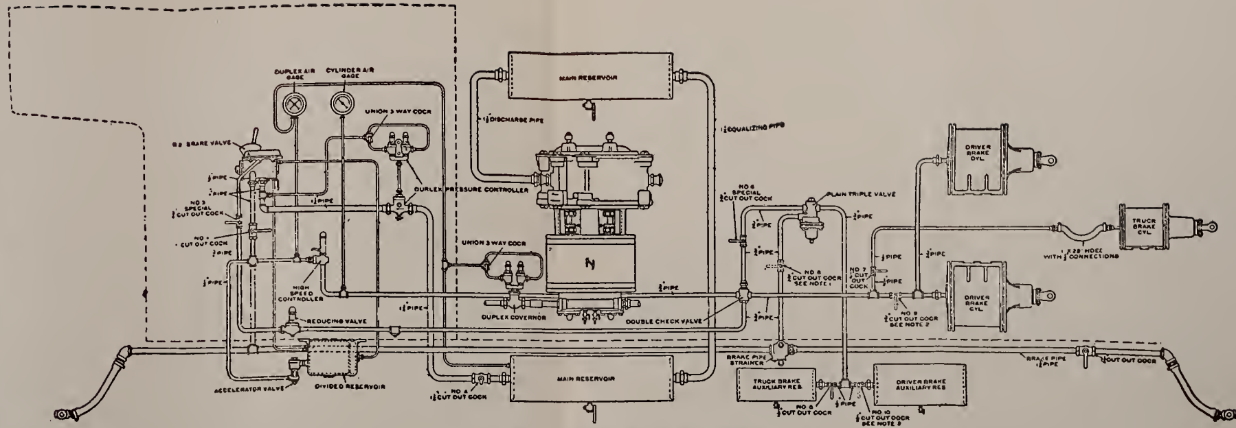
PIPING DIAGRAM B2—HS EQUIPMENT.
