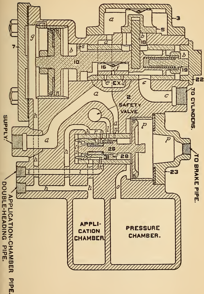
FIG. 301. INDEPENDENT LAP
