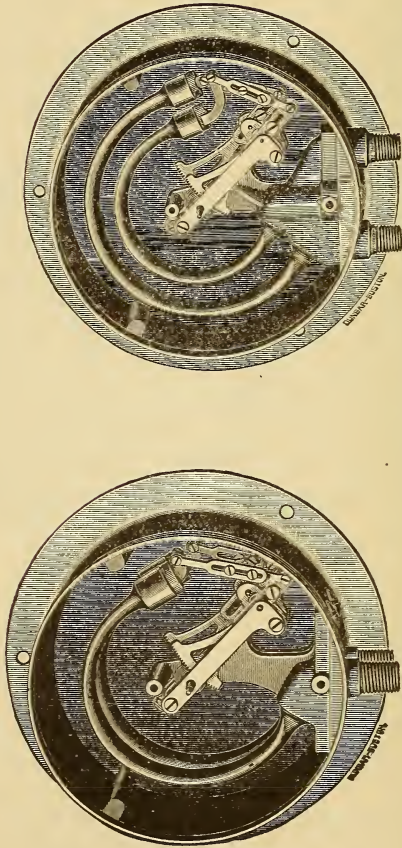
FIGURE 180 CROSBY DUPLEX GAUGE, SECTIONAL VIEW
