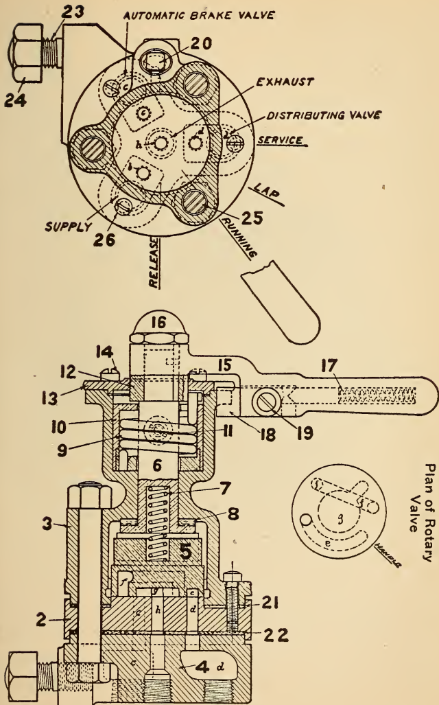
FIG. 316. INTERIOR VIEWS OF THE INDEPENDENT BRAKE VALVE
