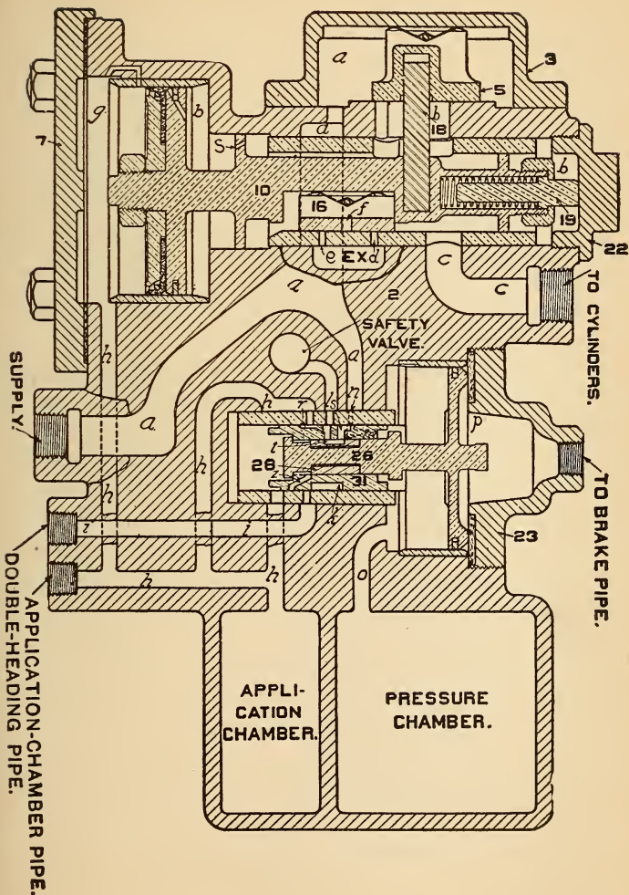
FIG. 305. EMERGENCY LAP
