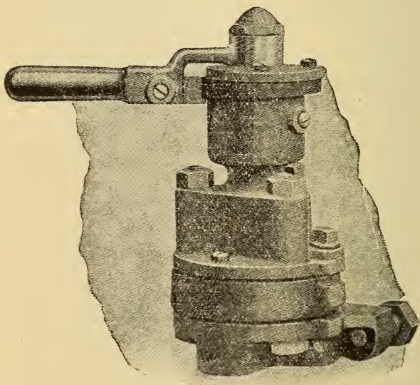
FIG. 314. THE INDEPENDENT BRAKE VALVE
