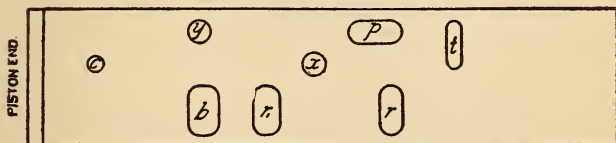
SLIDE VALVE SEAT.
