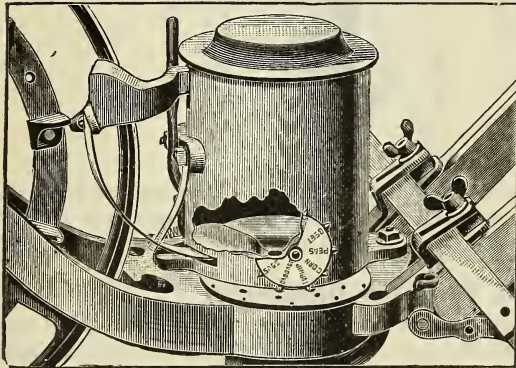
MATTHEW HILL AND DRILL SEEDER.
