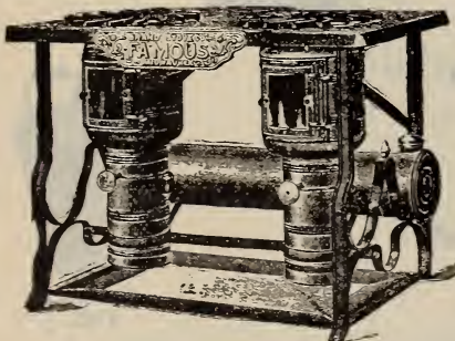
One, Two, Three and Four-Hole Oil Stoves; also, Electric Blue-Flame Naphtha Stoves, for Heating and Cooking.
