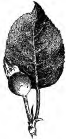
FIG. 140. Almost too late to spray for codling moth
