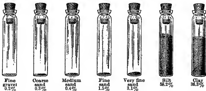
FIG. 42. Composition of a clay loam
