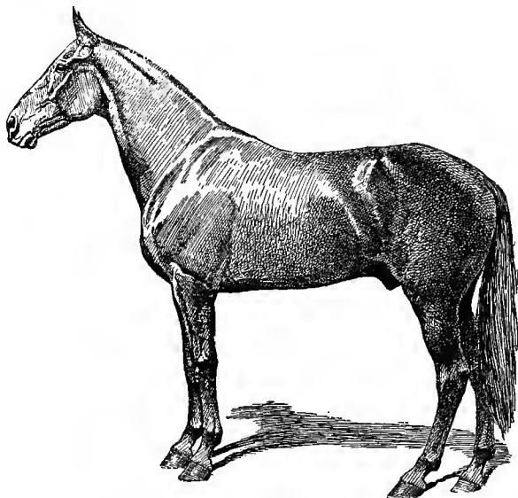
FIG. 146. The speed type. Dan Patch, 1:55 \frac{1}{4}
