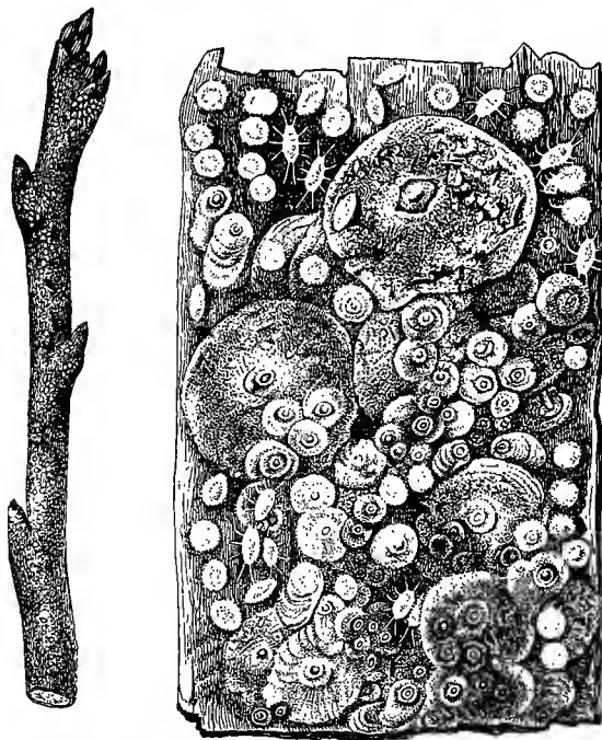
FIG. 141. San José scale. Natural size on the left; much enlarged on the right. A sucking insect. (After Howard and Morlatt)
