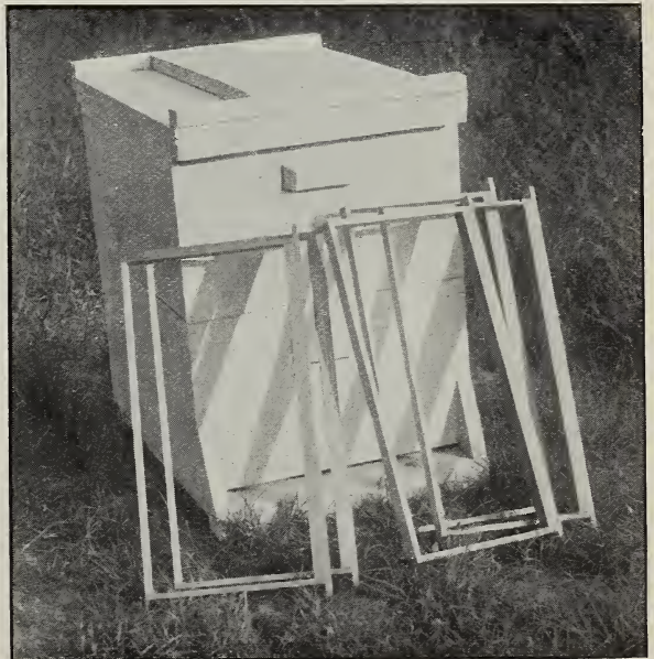
TEN-FRAME HIVE COMPLETE, MADE WITH ROBINSON'S WIND-POWER BUZZ-SAW.
