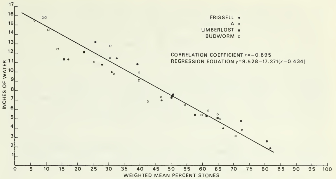
Figure 3.--Retention storage capacity in the surface 48 inches of 40 soil profiles representing four soil series as a function of average stone content.
