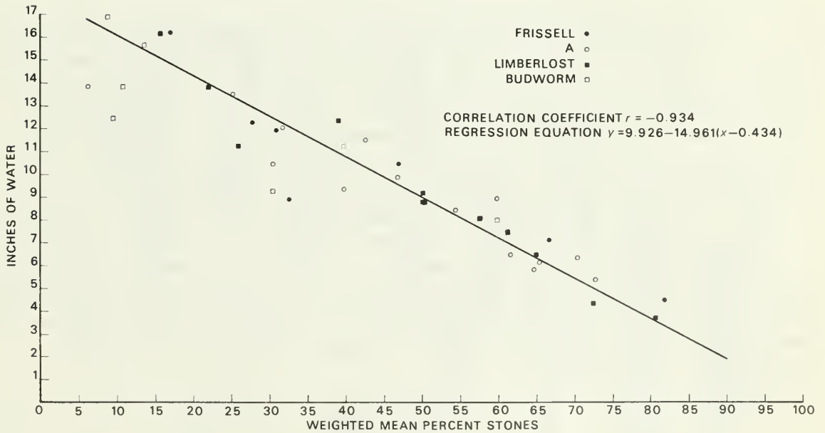
Figure 4.--Detention storage capacity in the surface 48 inches of 40 soil profiles representing four soil series as a function of average stone content.
