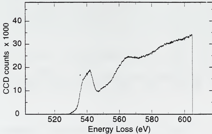
Figure 4.68 PEELS analysis of inclusion JWV1 Region A - O K spectrum
