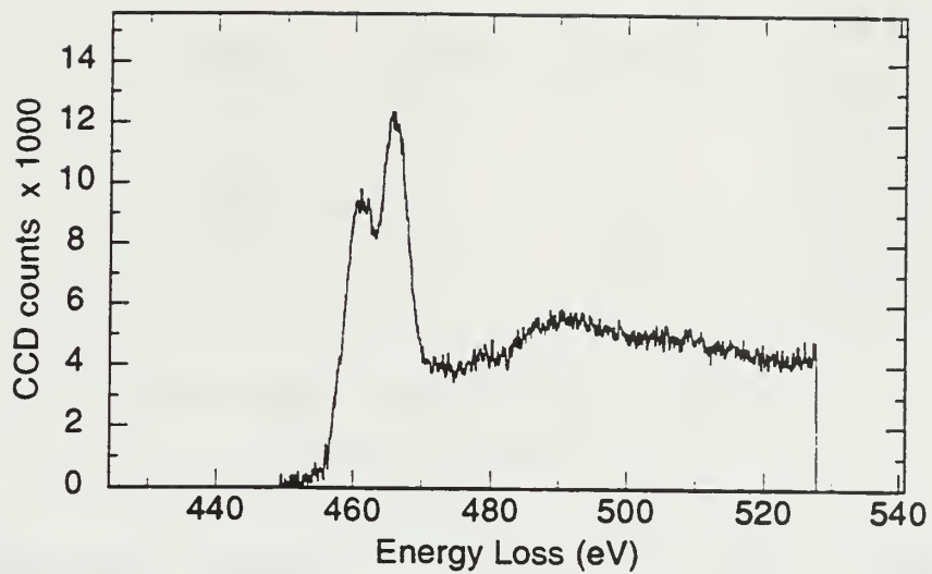
Figure 4.82 PEELS analysis of inclusion J WV2 Region B - Ti_{L_{2,3}} spectrum
