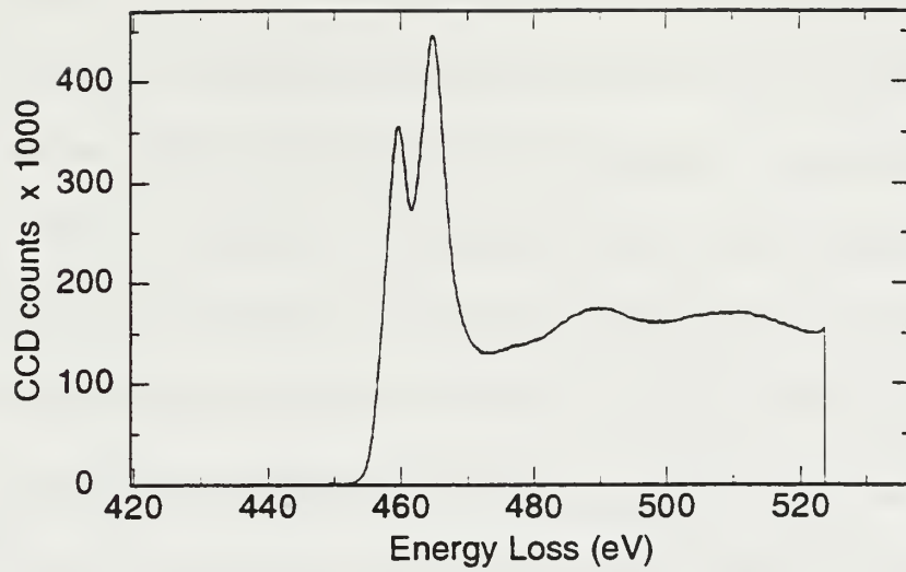
Figure 4.26 PEELS analysis of inclusion JWY2 - Ti L2,3 spectrum
