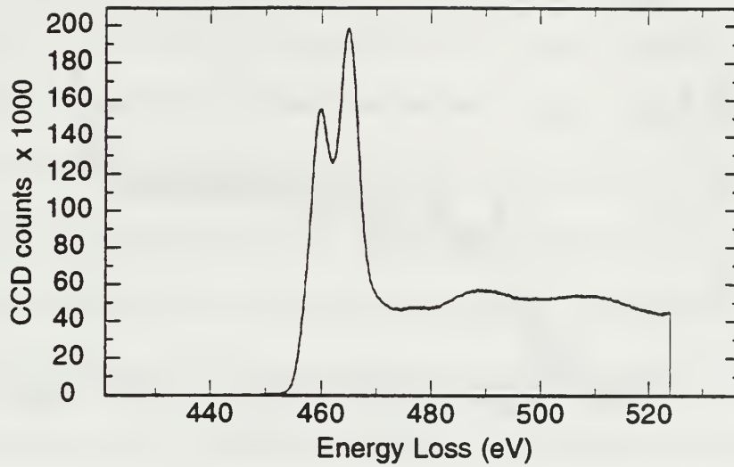
Figure 4.43 PEELS analysis of inclusion JWZ1 - Ti_{L2,3} spectrum
