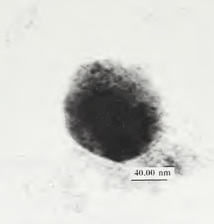
Figure 4.58 TEM microrgraph of inclusion JWZ3
