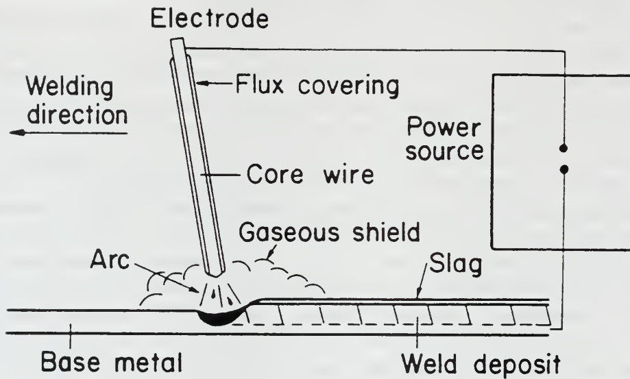
Figure 2.1 SMA welding process [From Ref. 2]
