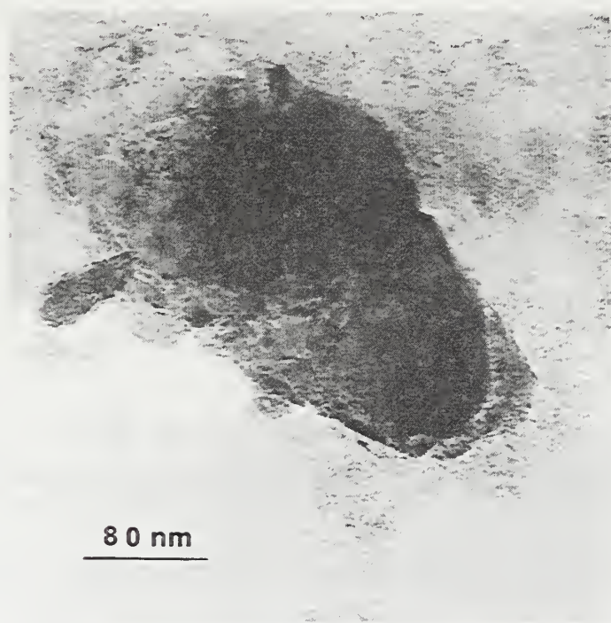
Figure 4.24 TEM micrograph of inclusion JWY2
