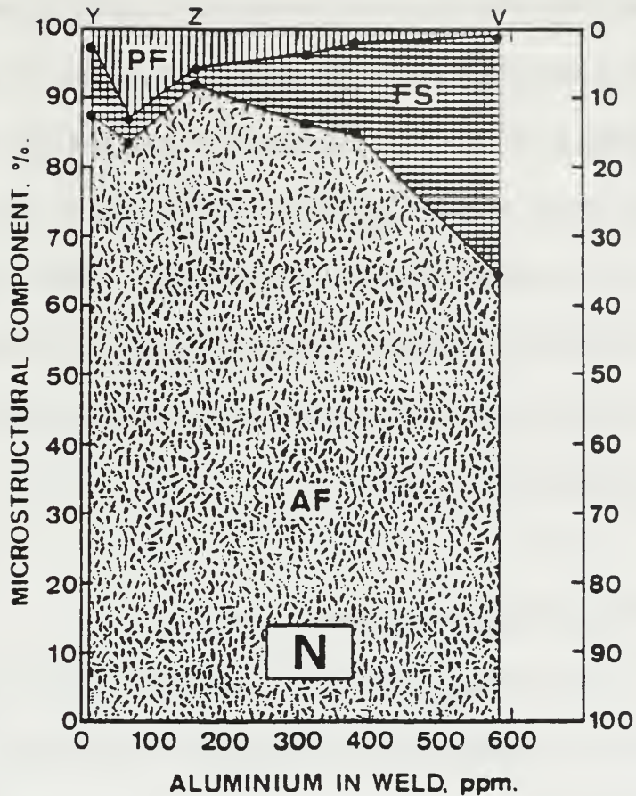
Figure 4.11 Effect of aluminum on weld metal microstructure of samples Y, Z and V [From Ref. 32]
