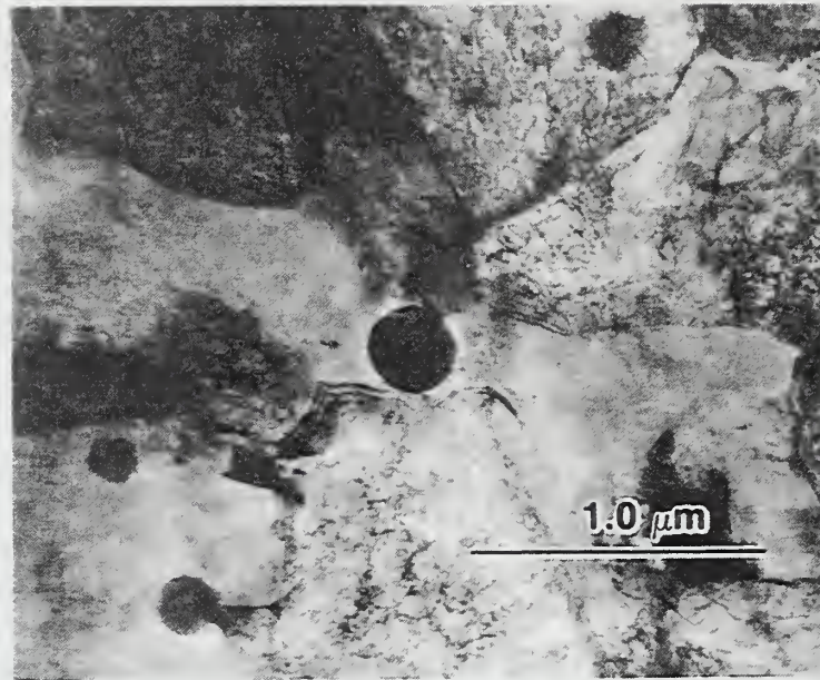
Figure 2.12 Multiple nucleation of acicular ferrite on an inclusion in a C-Mn steel weld metal containing 28 ppm titanium [From Ref. 30]
