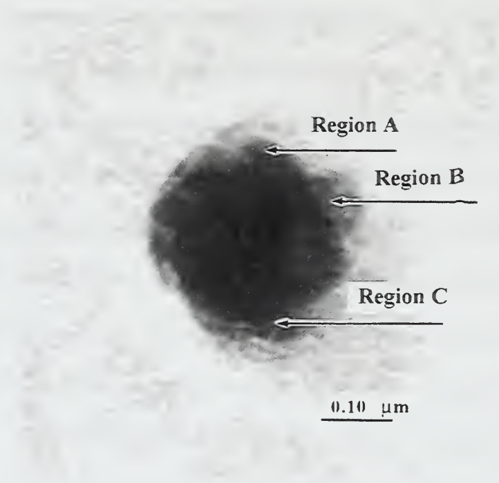
Figure 4.92 TEM micrograph of inclusion JWV3
