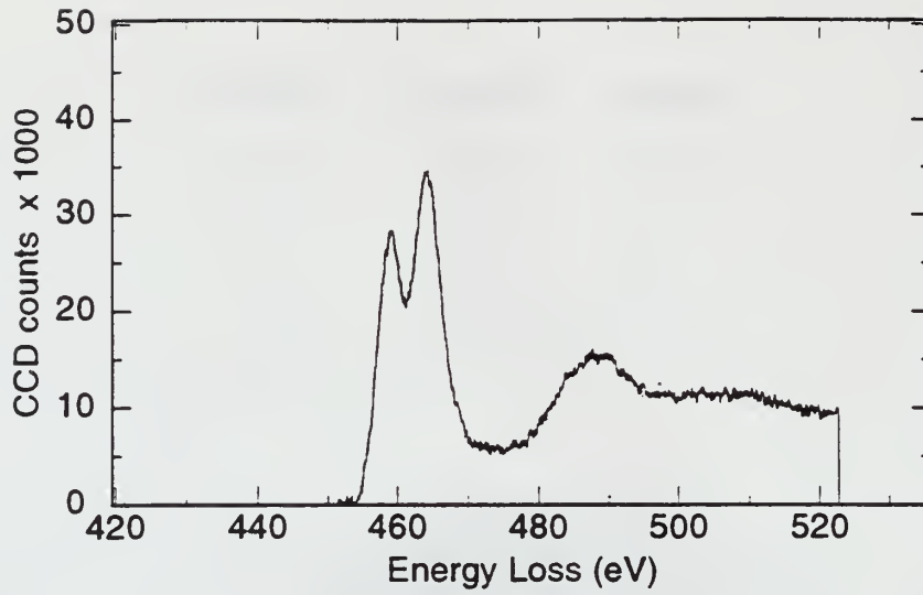
Figure 4.94 PEELS analysis of inclusion JWV3 Region A - Ti L2,3 spectrum
