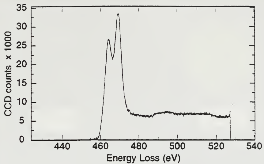
Figure 4.60 PEELS analysis of inclusion JWZ3 - Ti L2,3 spectrum
