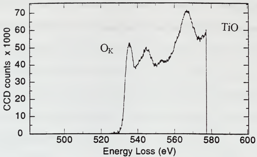
Figure 4.13 Energy loss spectra for oxygen - TiO
