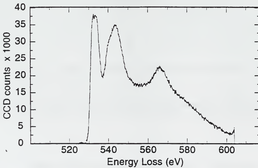
Figure 4.32 PEELS analysis of inclusion JWY3 Region A - O_K spectrum
