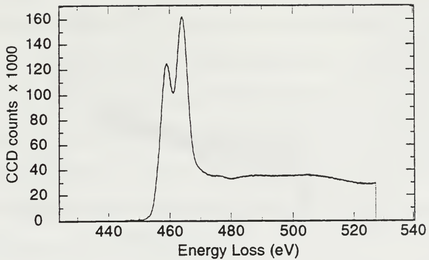
Figure 4.54 PEELS analysis of inclusion JWZ2 Region B - Ti_{L_{2,3}} spectrum
