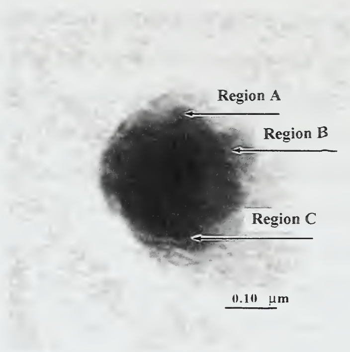
Figure 4.75 TEM micrograph of inclusion JWV2
