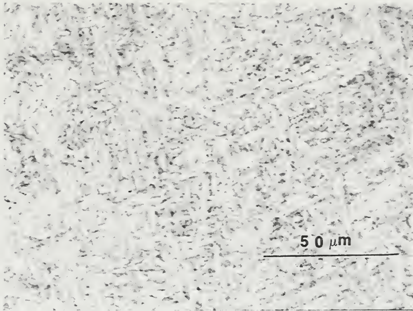
Figure 4.4 Optical micrographs of final weld pass of sample Z
