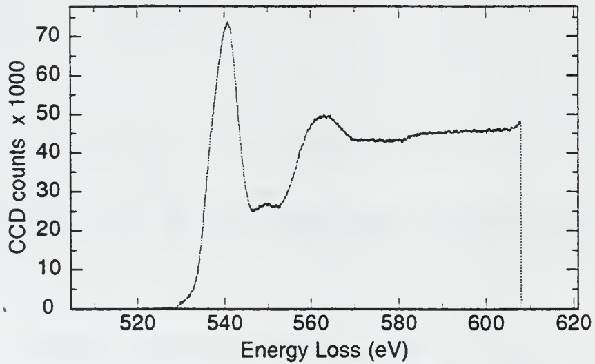
Figure 4.50 PEELS analysis of inclusion JWZ2 Region A - O K spectrum
