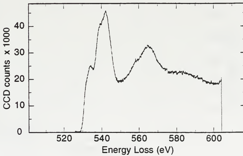
Figure 4.44 PEELS analysis of inclusion JWZ1 - O_K spectrum
