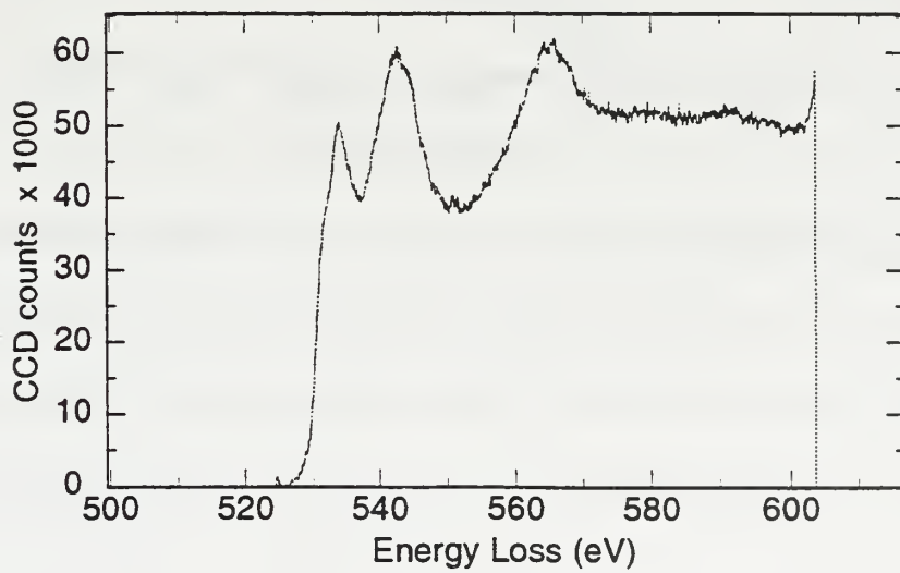
Figure 4.27 PEELS analysis of inclusion JWY2 - O K spectrum
