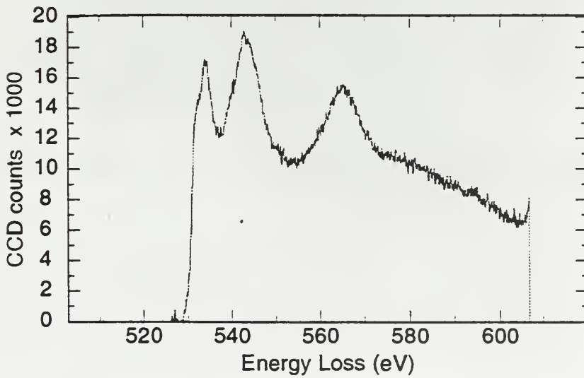
Figure 4.22 PEELS analysis of inclusion JWY1 - O K spectrum
