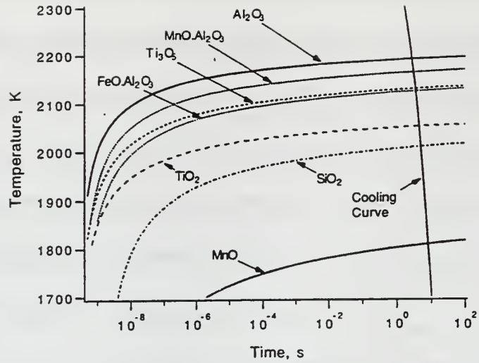
Figure 2.8 TTT curve generated using extent of reaction equations [From Ref. 14]
