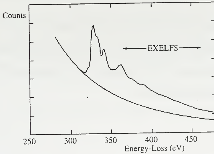
Figure 3.14 EXELFS Features of an inner-shell ionization edge [From Ref. 35]
