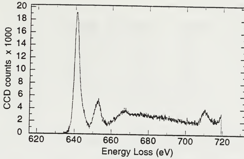
Figure 4.51 PEELS analysis of inclusion JWZ2 Region A - Mn_{L_{2,3}} spectrum
