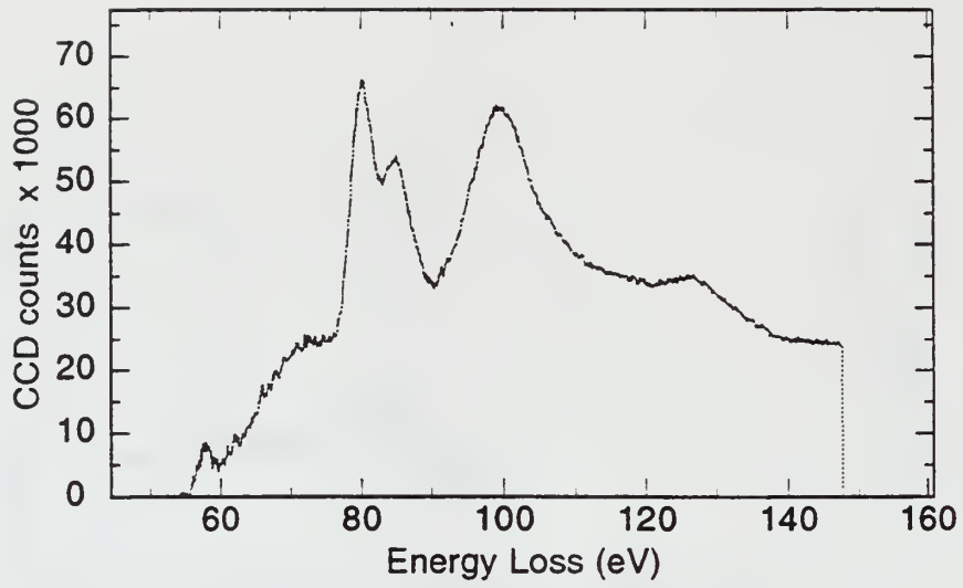
Figure 4.84 PEELS analysis of inclusion JWV2 Region B - Al_{L_{2,3}} spectrum
