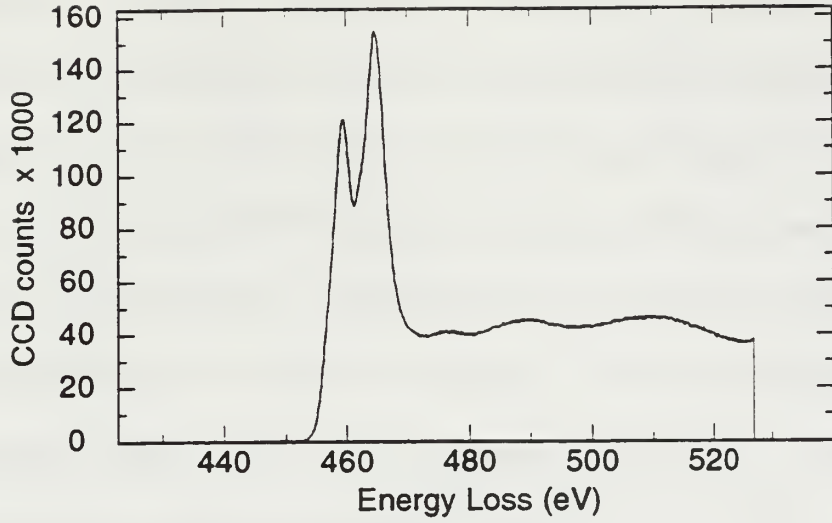
Figure 4.21 PEELS analysis of inclusion JWY1 - Ti L2,3 spectrum
