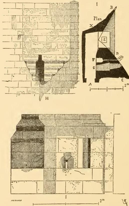
Fig. 378. Latrines in the Palace of Courci, France. 13th Century.*
