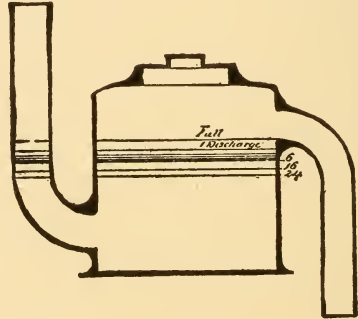
Fig. 249. 8 in. Pot.
