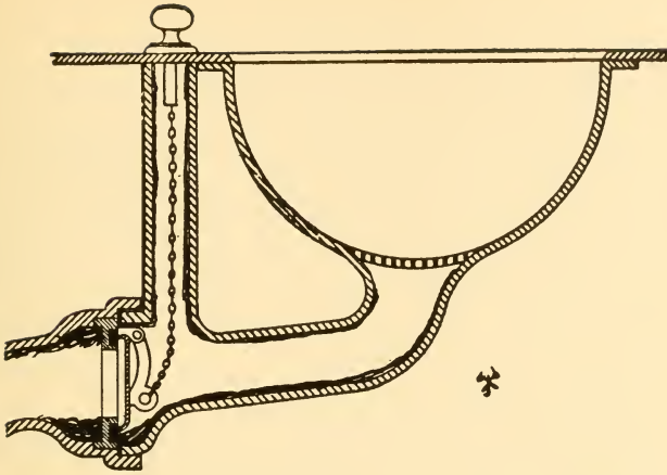
Fig. 312. Valve-Outlet Basin with Chain Movement.
