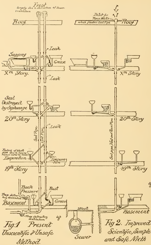
Figs. 264 and 265. Two Diagrams comparing together the Complex and Simple Systems in a Modern Tall Office Building. From the "Inland Architect and News Record" for Oct., 1905, article by J. P. Putnam.
