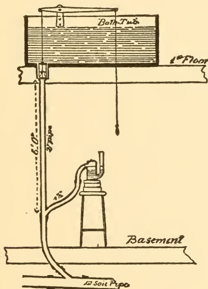
Fig. 243. Simple Apparatus for Trap Testing.
