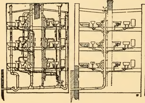
Fig. 2. Complexity and Danger. Type of system of extreme complication to which we are tending.
