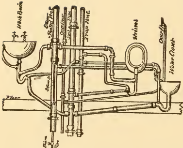
Fig. 30. Complexity with Inse-urity.
