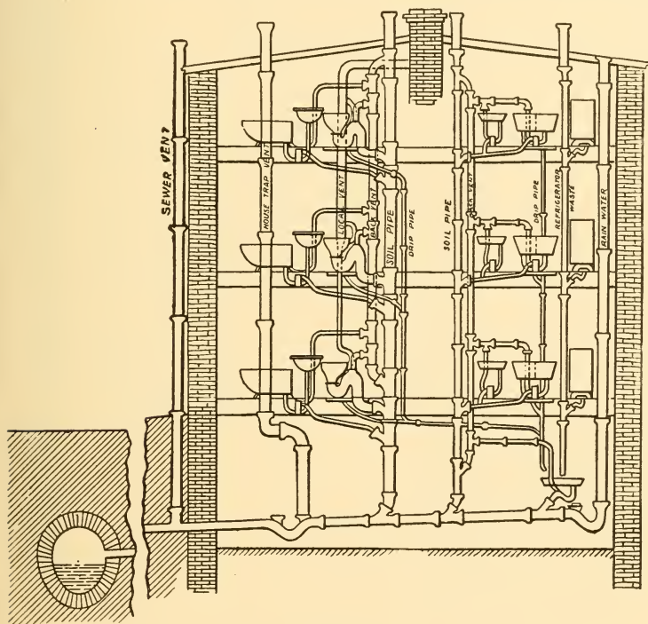
Fig. 32. Complicated plumbing, showing the modern tendency.
