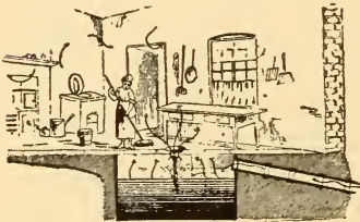
Fig. 633. Dish stone in scullery untrapped, and opening direct into a rain water tank, with overflow into drain.
