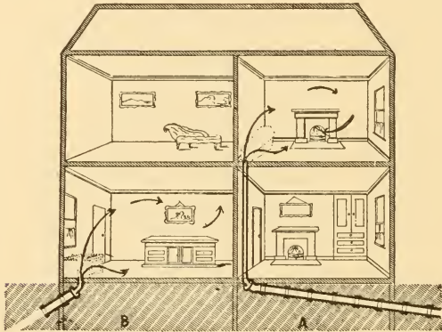
Fig. 618. "A" Bath waste pipe cut off and left open to the drain, "B," Sink waste pipe ditto.
