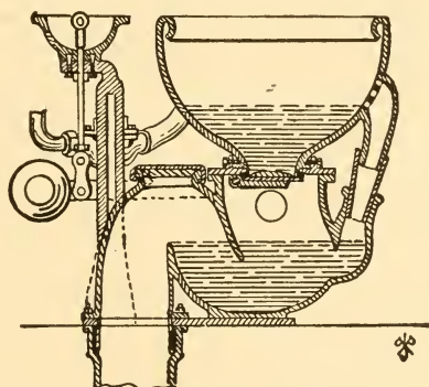
Fig. 386. Valve Closet.
