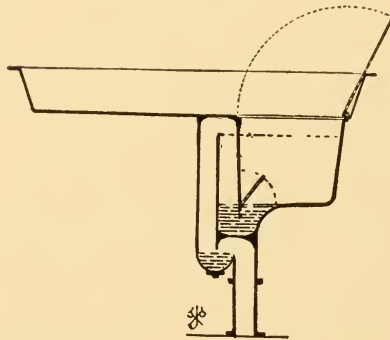
Trap 366h. Section of "Securitas" Sink.
