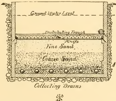
Fig. 640. Transverse Section of Filter Bed.
