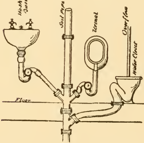
Fig. 31. Simplicity with Security.
