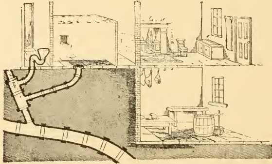
Fig. 606. Six-inch pipe between two four-inch pipes.
