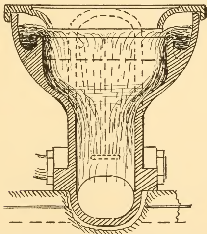
Fig. 430. Transverse Section of Final Improvement.
