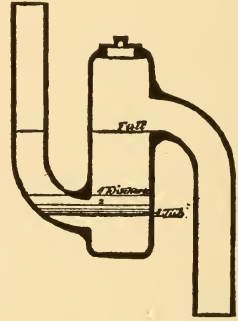
Fig. 247. 2½ in. Pot.
