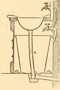
Fig. 316. French "Perfected" Bath Room Apparatus.*
