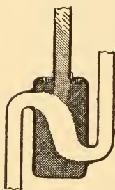
Fig. 38. Vented Pot becoming an Unvented S Trap.
