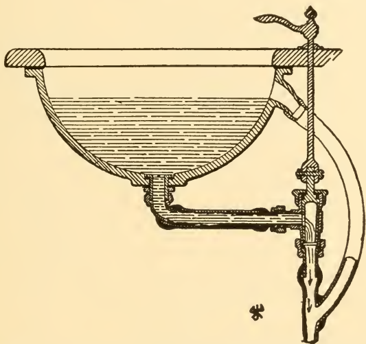
Fig. 308. Waste-Cock Outlet Basin, the "Boston Waste."
