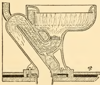
Fig. 422. Section of the Sanitas W. C. Outfit.
