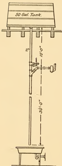
Fig. 549. Trap Testing Apparatus.
