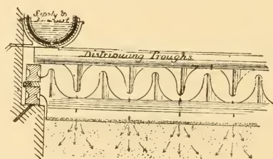
Fig. 642. Detail of Knife and Troughs.
