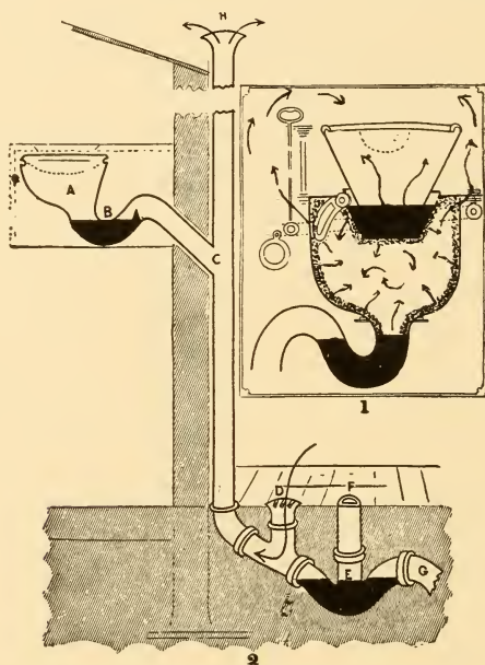
Fig. 332. Pan and Hopper Closets.*
