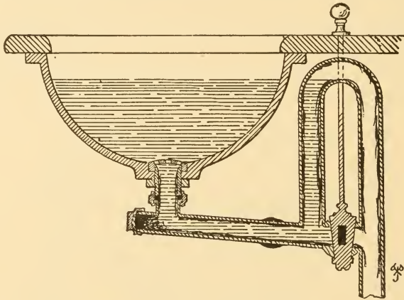
Fig. 309. The Waste-Cock Outlet Basin with Syphon Overflow.
