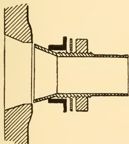
Fig. 439. Sanitas Coupling, ready to be connected.
