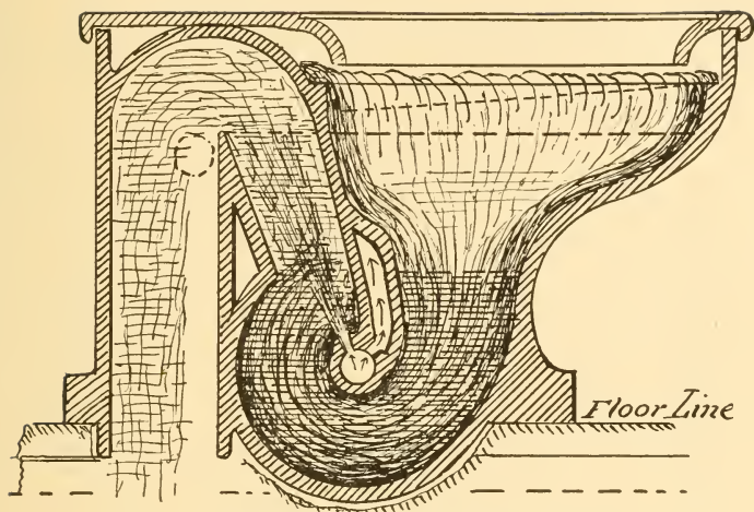
Fig. 429. Longitudinal Section of Final Improvement.
