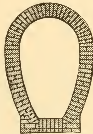
Fig. 50. Section of Egg-Shaped Sewer.
