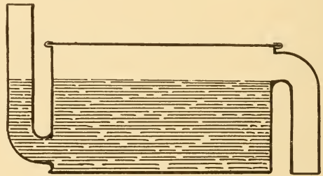
Fig. 146. Pot trap nine inches in diameter.
