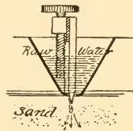
Fig. 647. Detail of Distributor.
