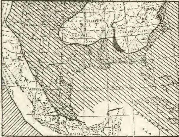
FIG. 2. THE TURONIAN SEA (LINED AREA) OF SOUTHERN NORTH AMERICA.
