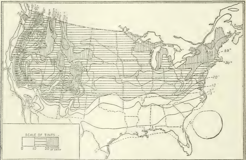
MEAN ANNUAL SNOWFALL MAP OF THE UNITED STATES. (C. F. Brooks.)
