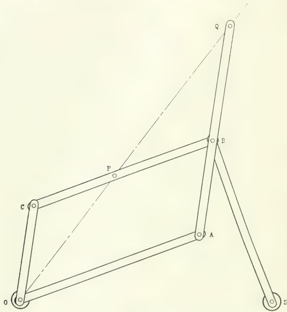
FIG. 5. PANTAGRAPH.
