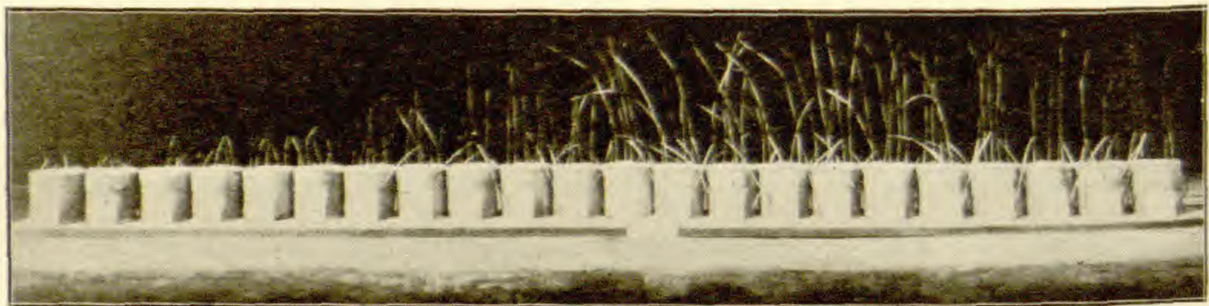
FIG. 6.—Lead nitrate series in soil. Sept. 2-14. 1905.
