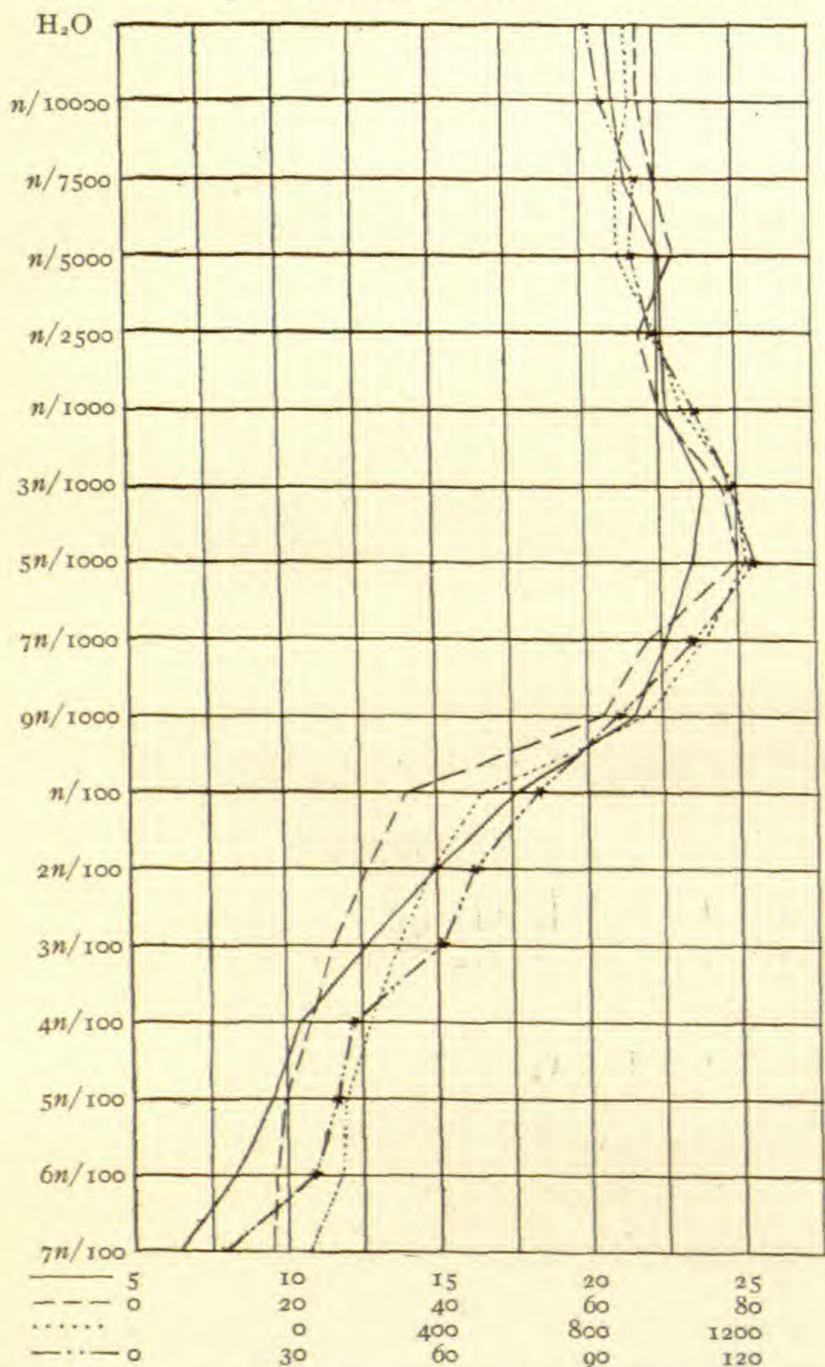
FIG. 26.—Iron nitrate series in soil with nutritive solution. Oct. 14-Nov. 8. 1905.
