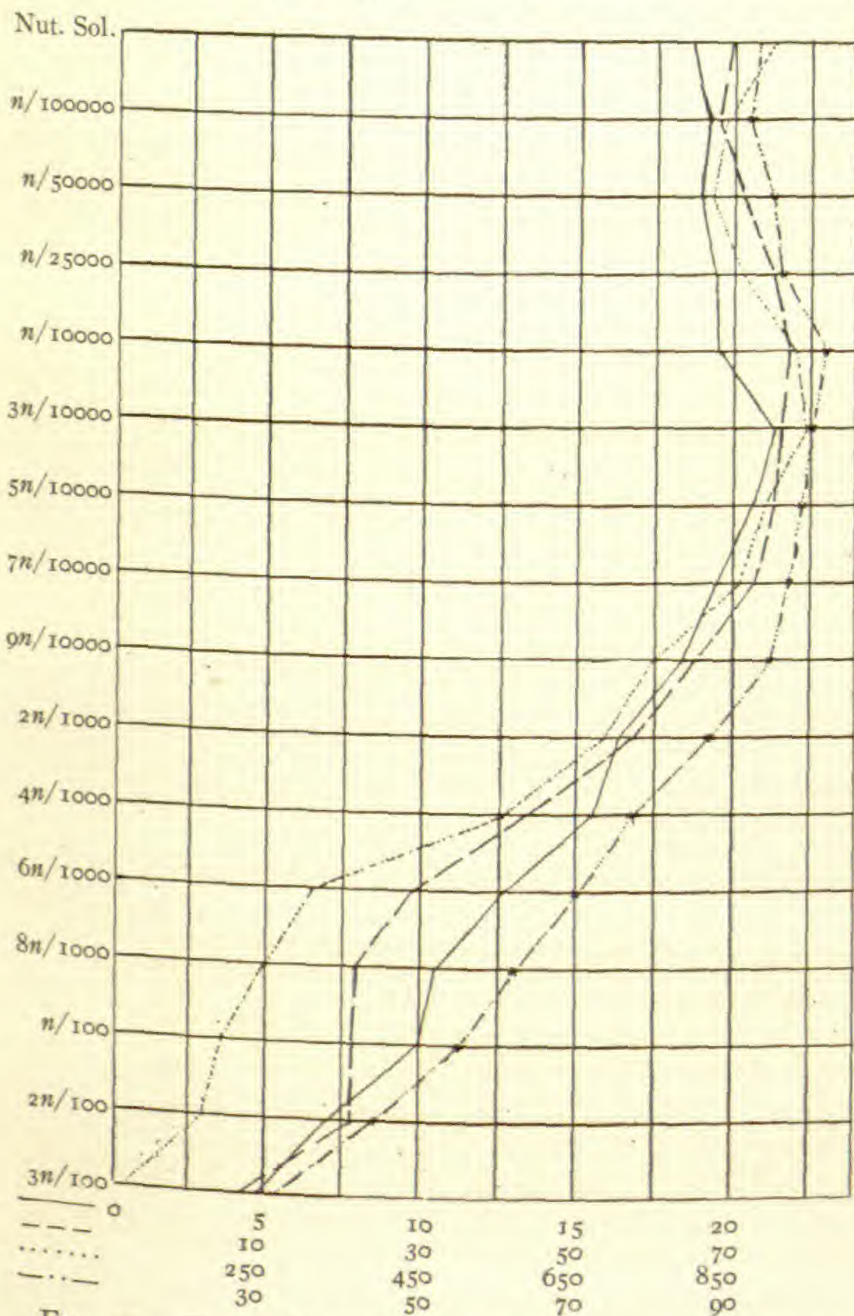
FIG. 20.—Zinc sulfate series in soil. Oct. 21-Nov. 18. 1905.
