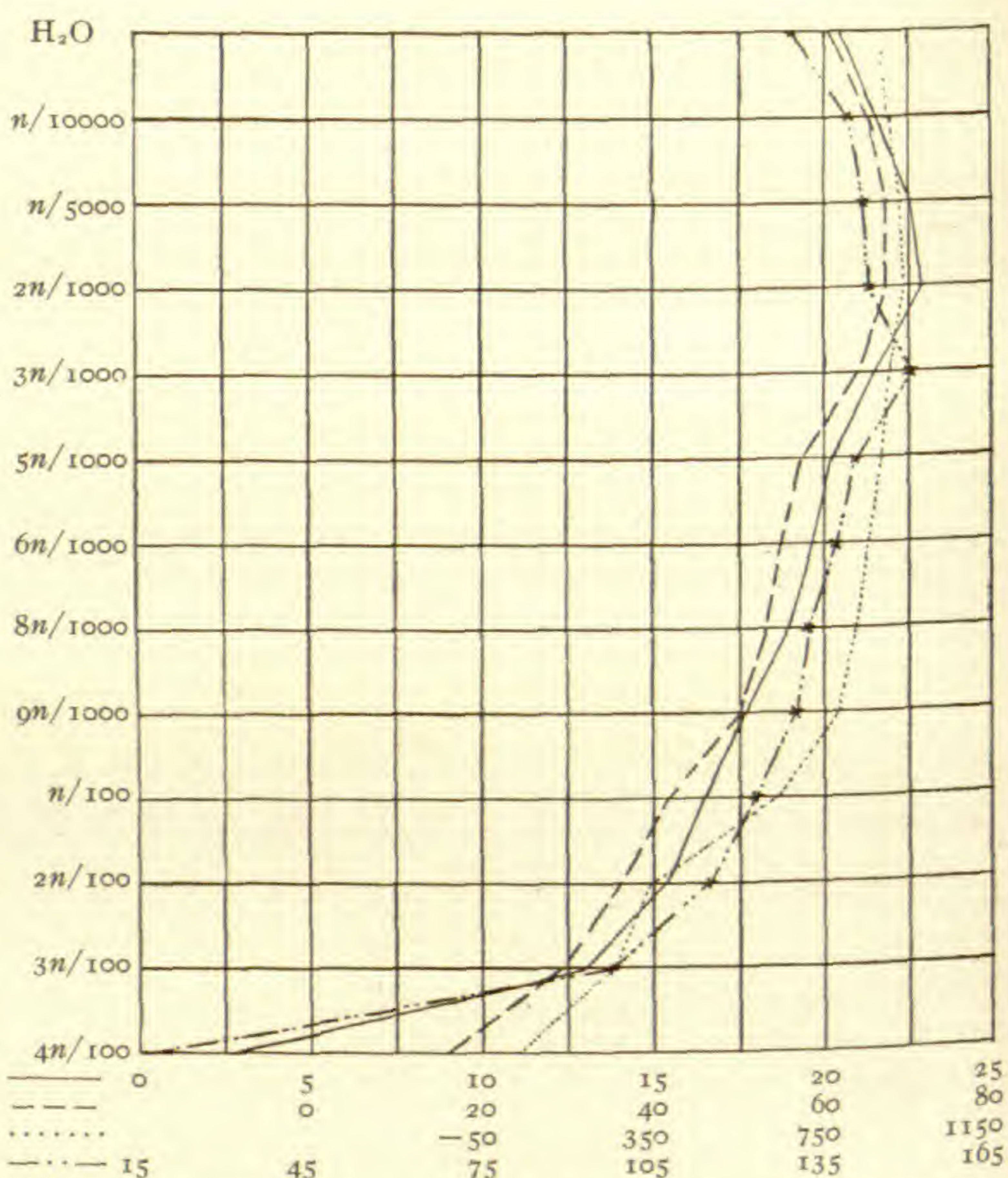
FIG. 13.—Silver nitrate series in soil. Average of results.
