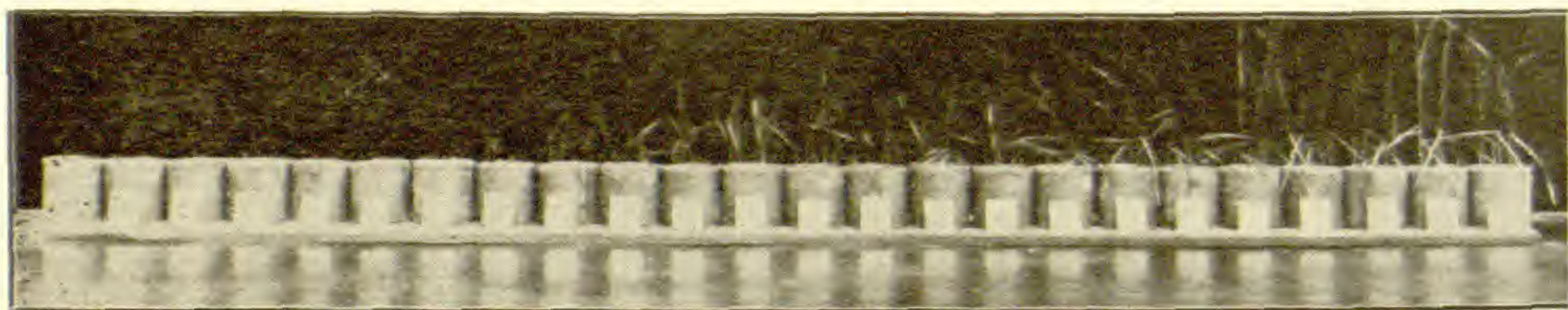
FIG. 2.—Copper sulfate series in soil. Aug. 24–Sept. 26. 1905.
