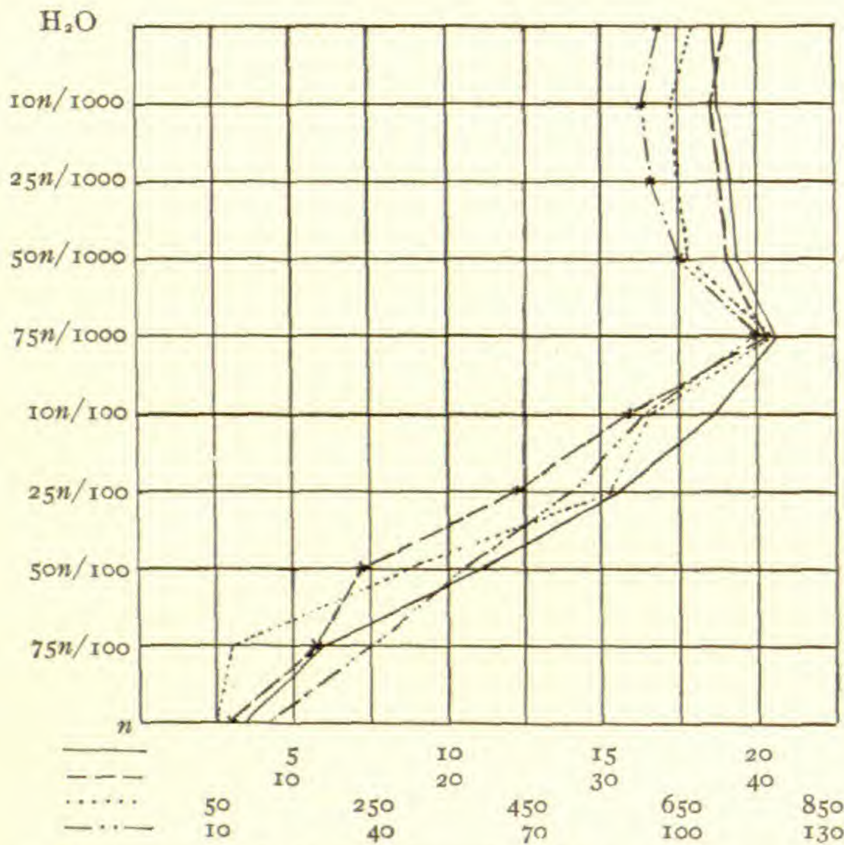
FIG. 33.—Alcohol series in soil. Mar. 2-22. 1906.
