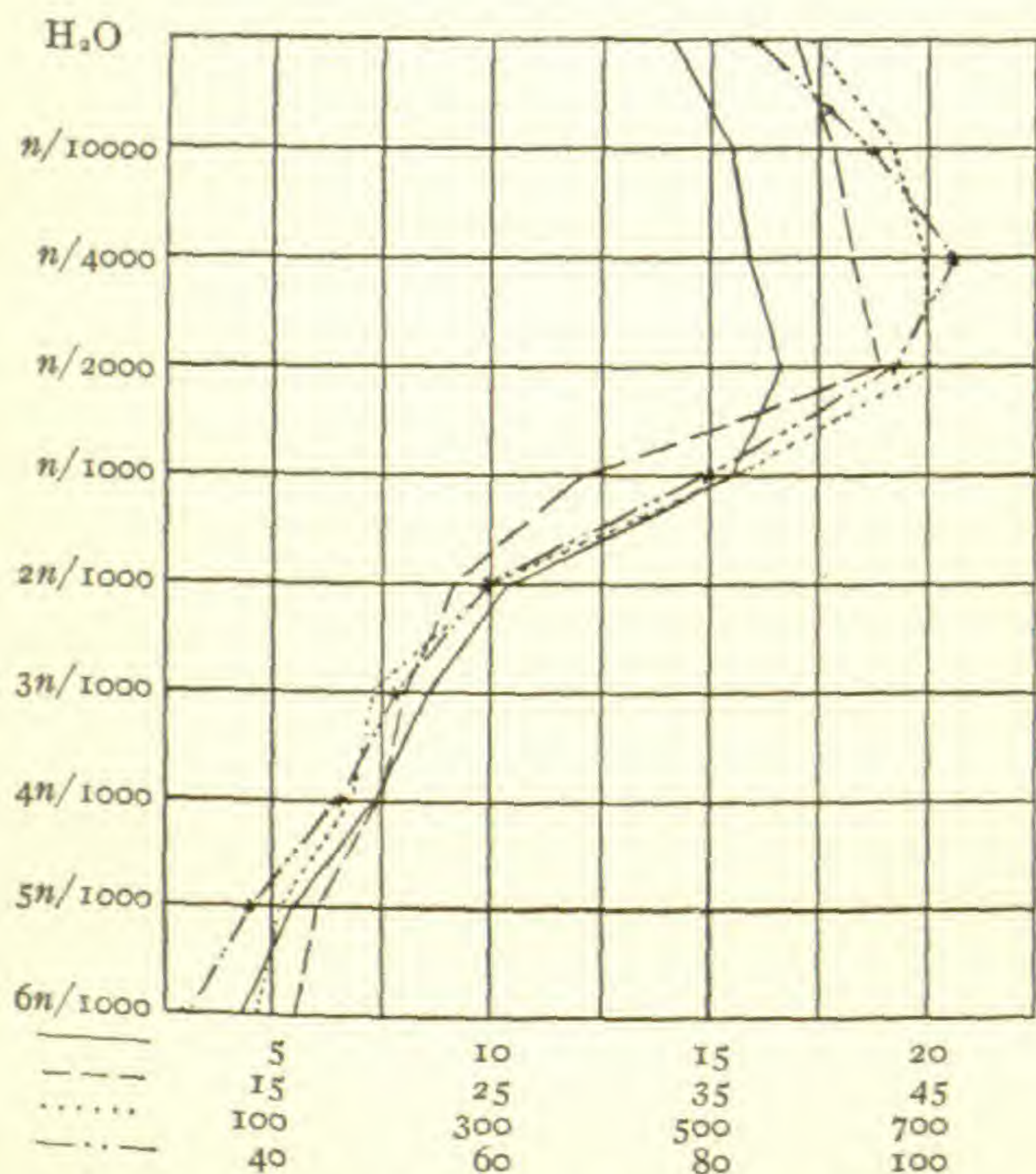
FIG. 29.—Nickel nitrate series in soil. Mar. 17-Apr. 2. 1906.
