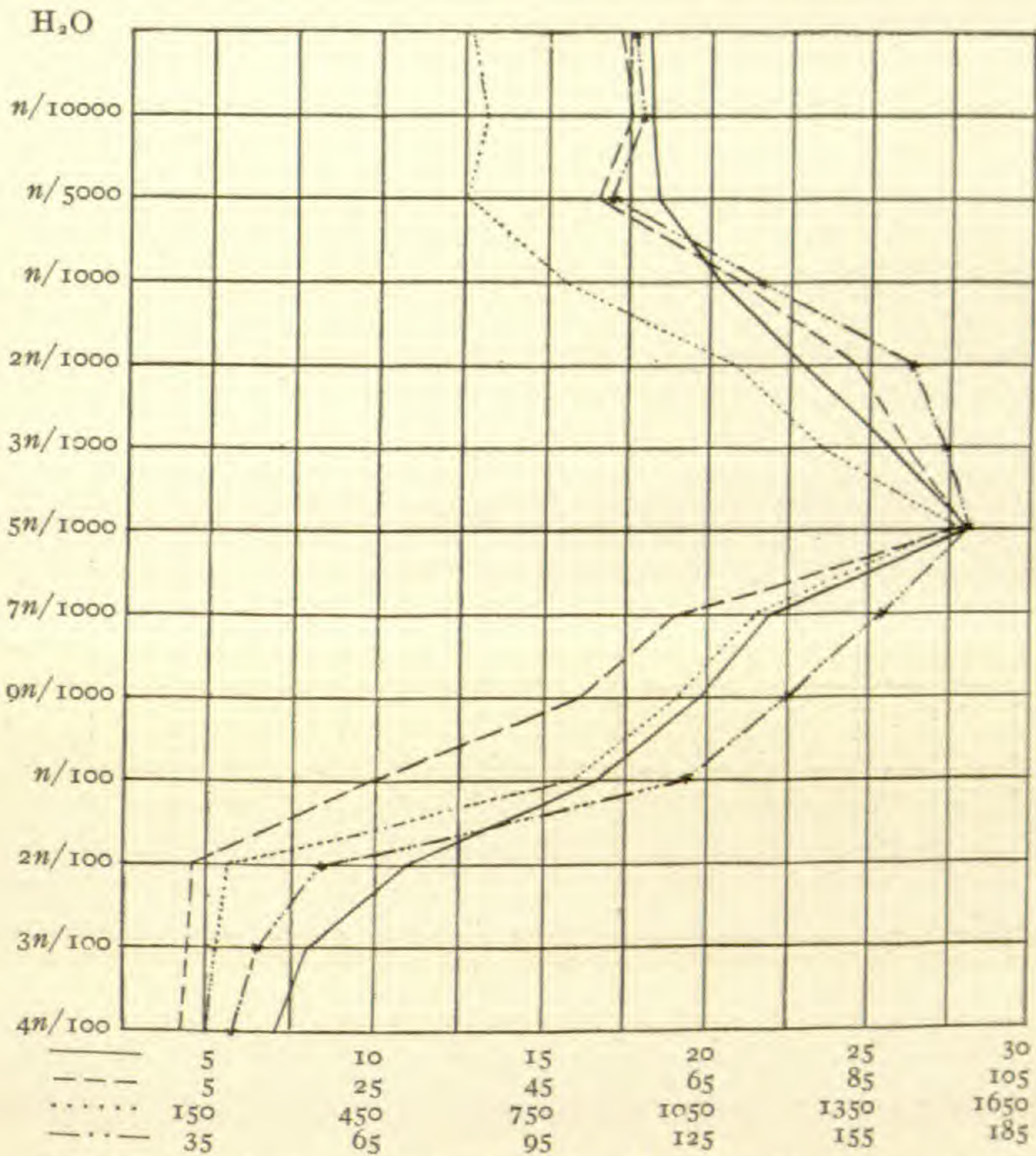
FIG. 8.—Lead nitrate series in soil. Nov. 19–Dec. 20. 1905.
