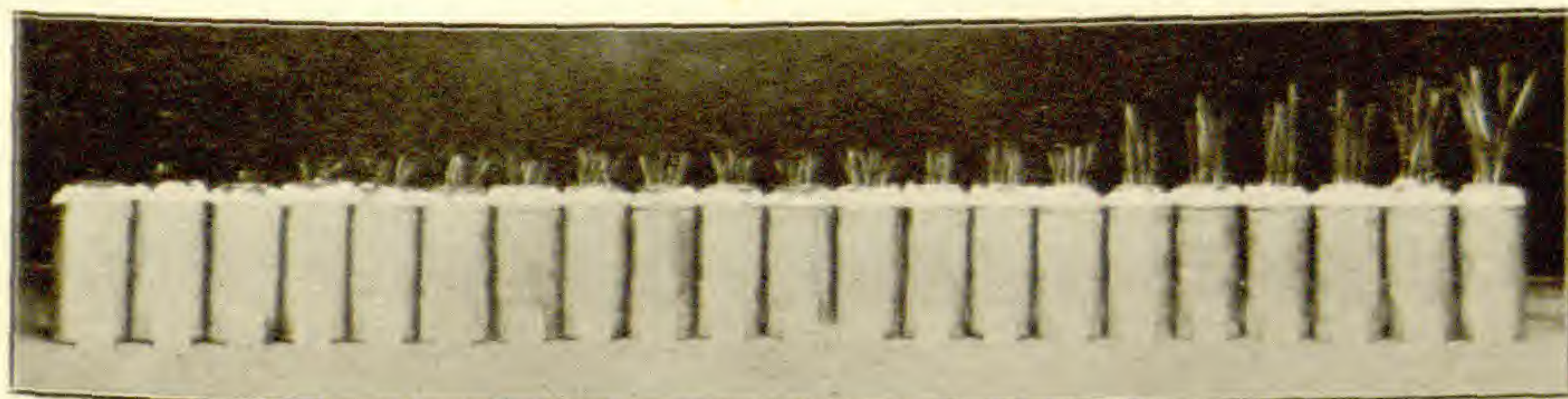
FIG. 16.—Silver nitrate series in solution. Sept. 10–15. 1905.
