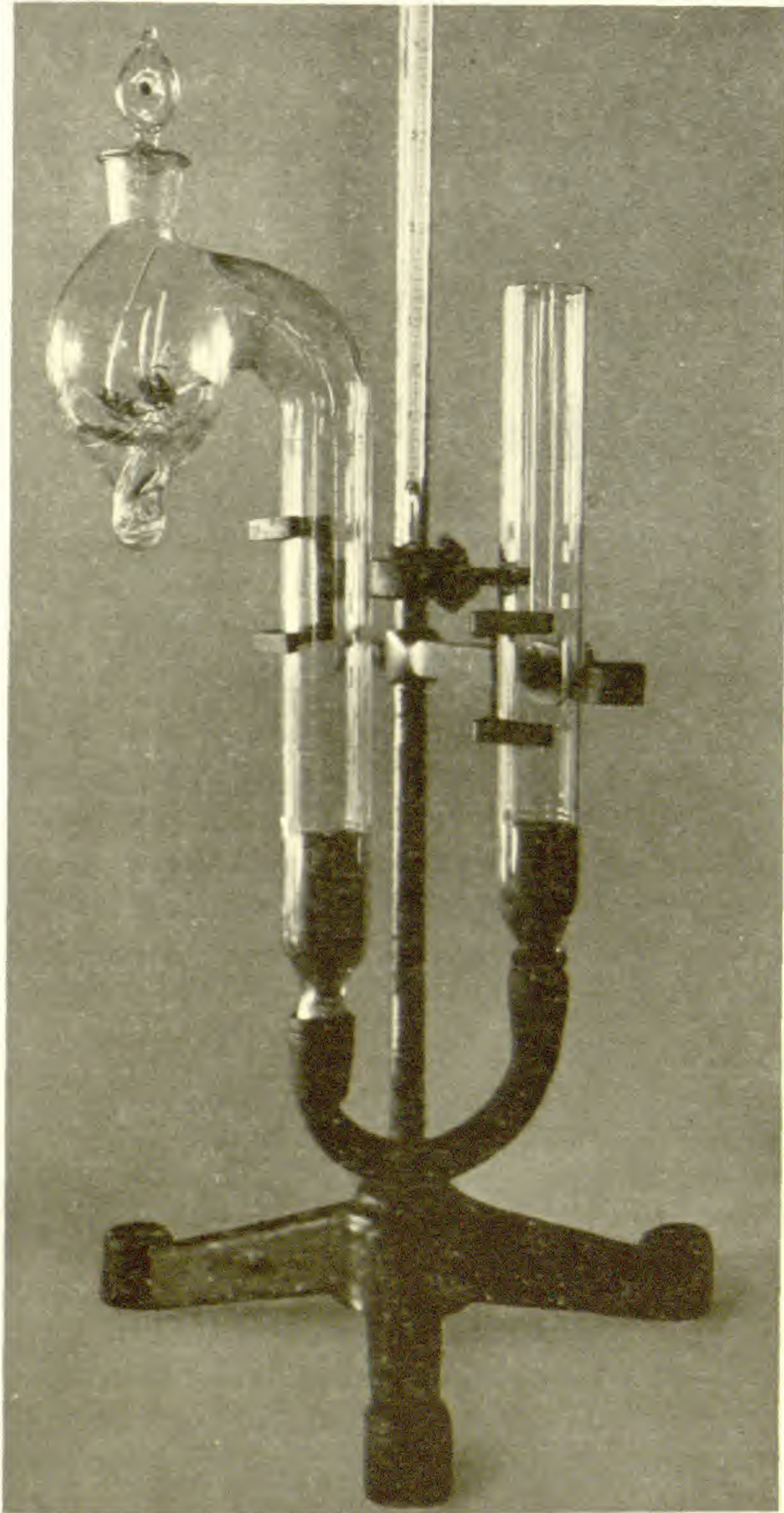
FIG. 1.—Respirometer.
