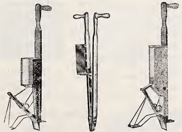
Rotary Planter No. 309 Acme Planter No. 306 One Hand Segment No. 311
