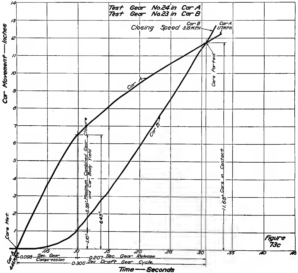
FIGS. 73B AND 73C—CAR-MOVEMENT CURVES, SUPERIMPOSED. MINER A-18-S GEARS THESE CURVES DRAWN BY CARS IN TEST
