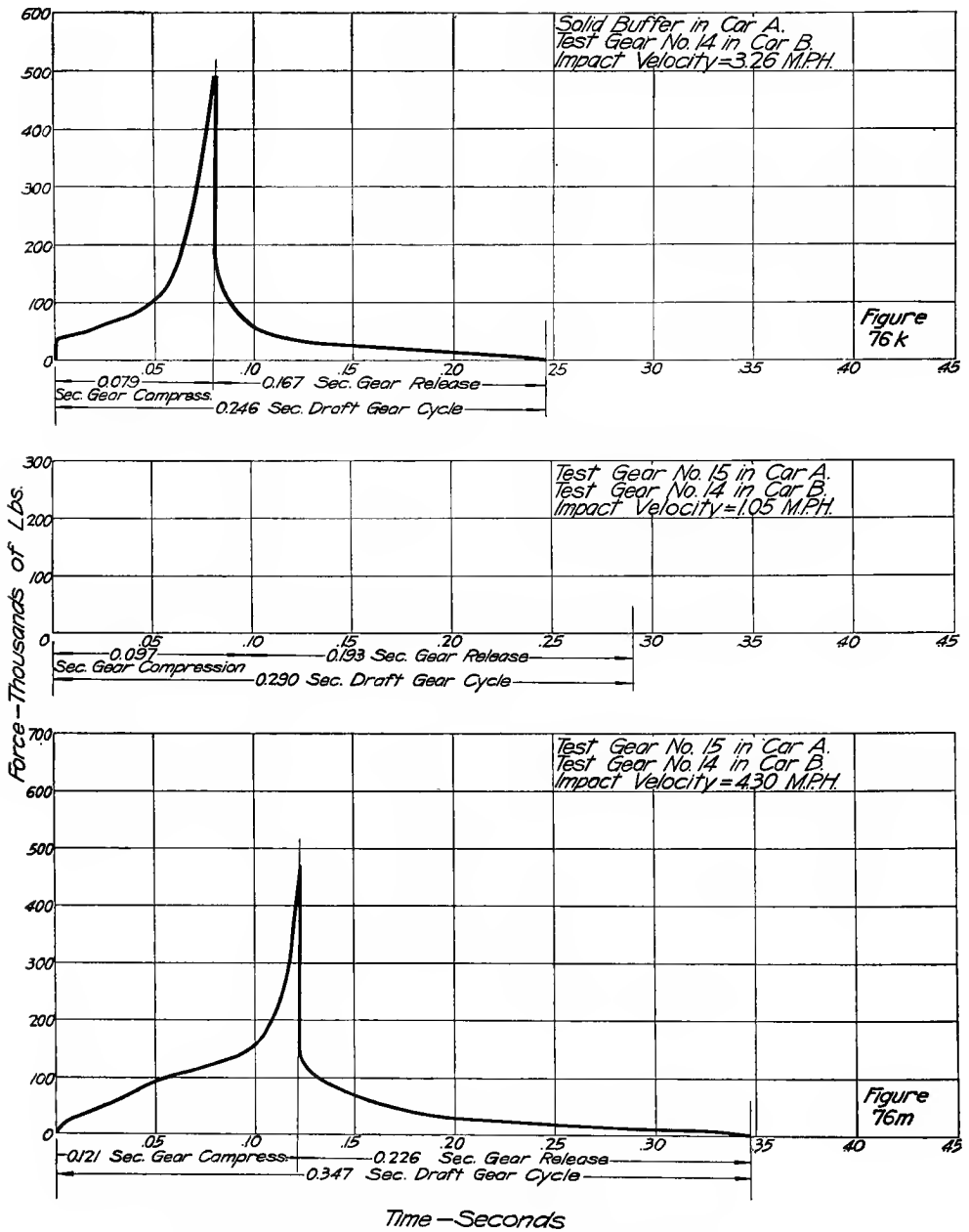
FIGS. 76K AND 76M—TIME-FORCE CURVES, SESSIONS JUMBO GEARS
