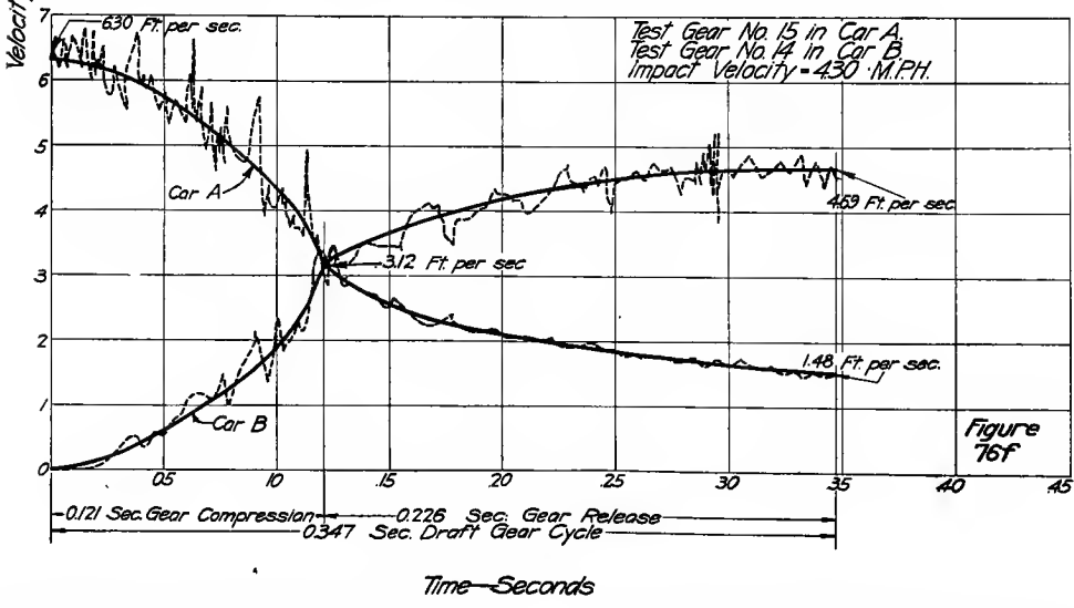
FIGS. 76D, 76E AND 76F—VELOCITY CURVES, SESSIONS JUMBO GEARS
