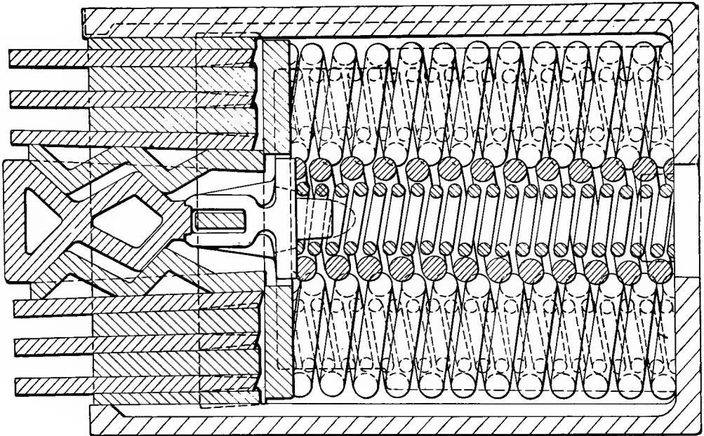
FIG. 3—WESTINGHOUSE NA-1 GEAR
