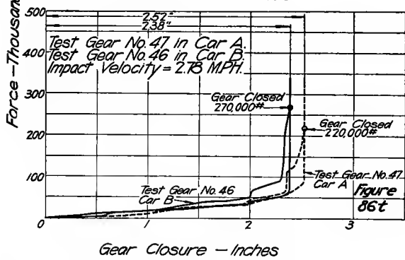
FIGS. 86r AND 86t—FORCE-CLOSURE DIAGRAMS, BRADFORD K GEARS
