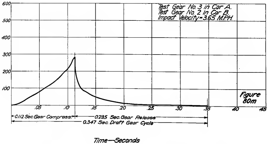
FIGS. 80K, 80L AND 80M—TIME-FORCE CURVES, WESTINGHOUSE D-3 GEARS
