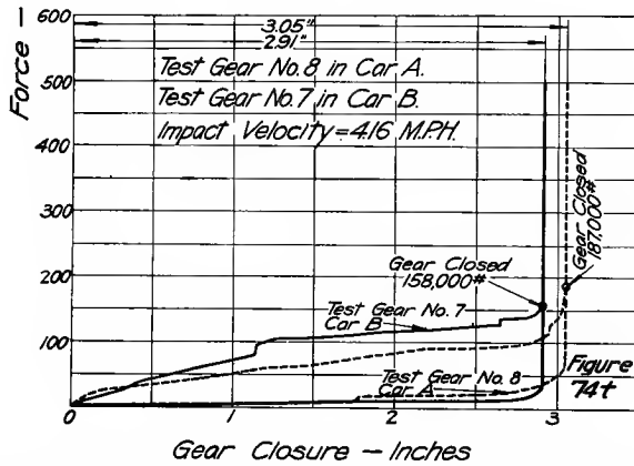
FIGS. 74R AND 74T—FORCE-CLOSURE DIAGRAMS, WESTINGHOUSE NA-1 GEARS
