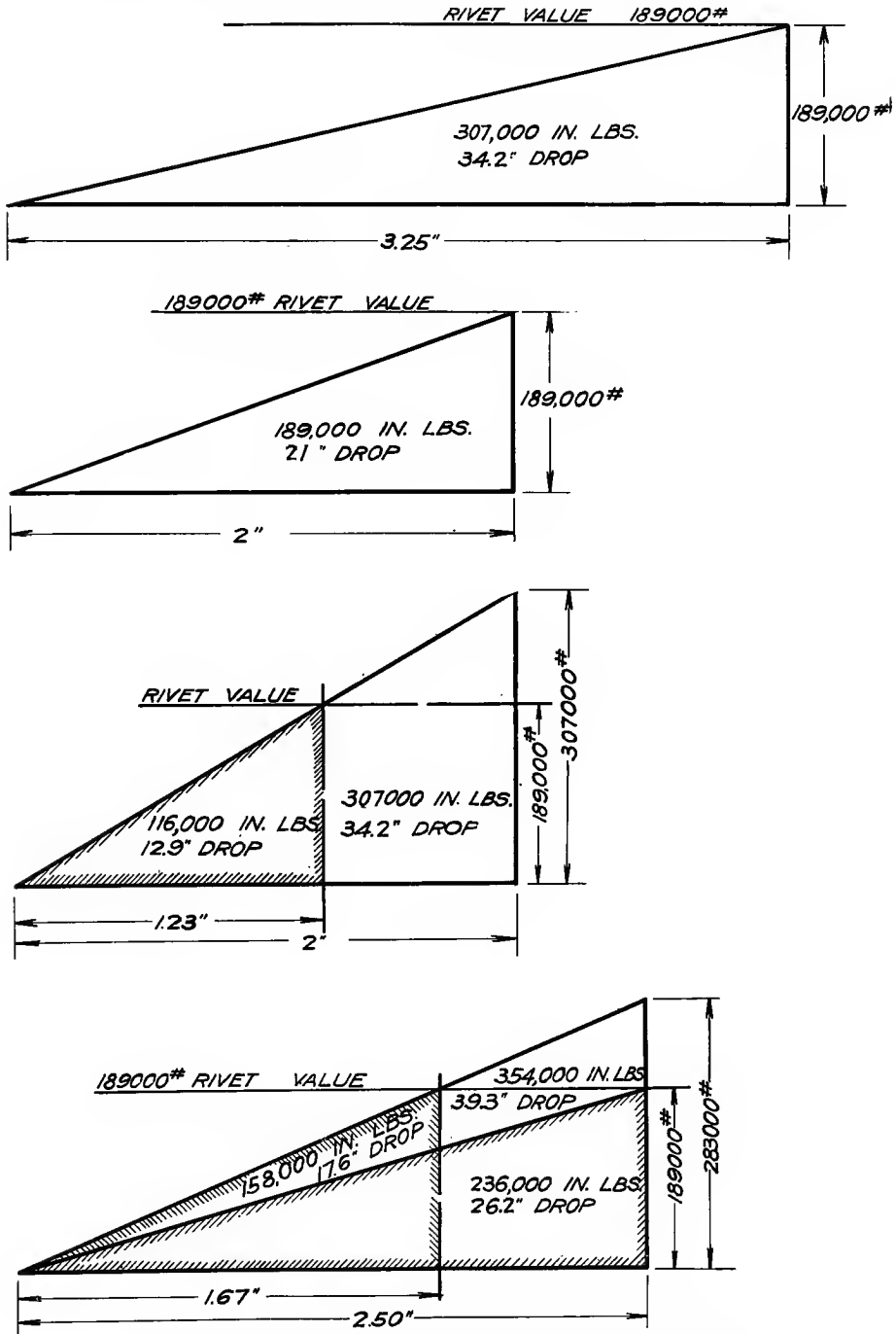
FIG. 41—DIAGRAMS OF RIVET SHEARING ACTION OF DRAFT GEARS
