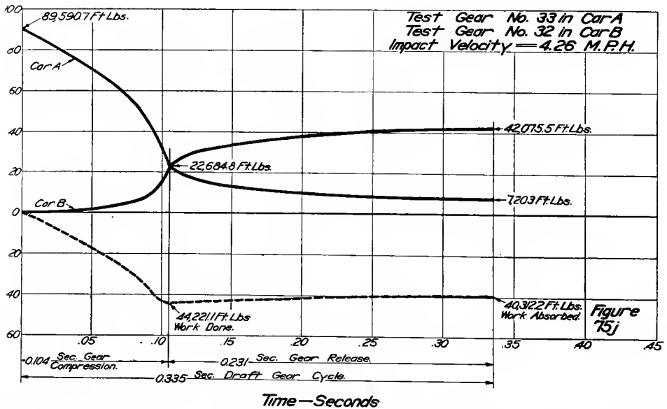
FIGS. 75C AND 75J—ENERGY CURVES, NATIONAL M-1 GEARS
