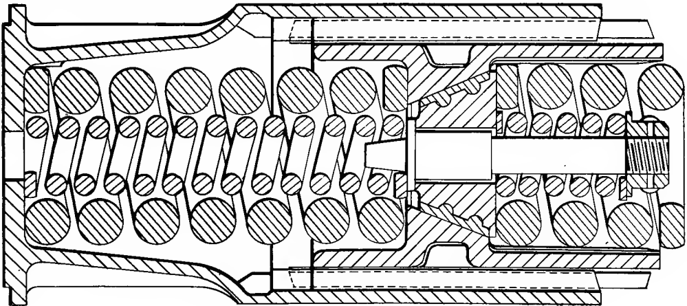
FIG. 2—WESTINGHOUSE D-3 GEAR
