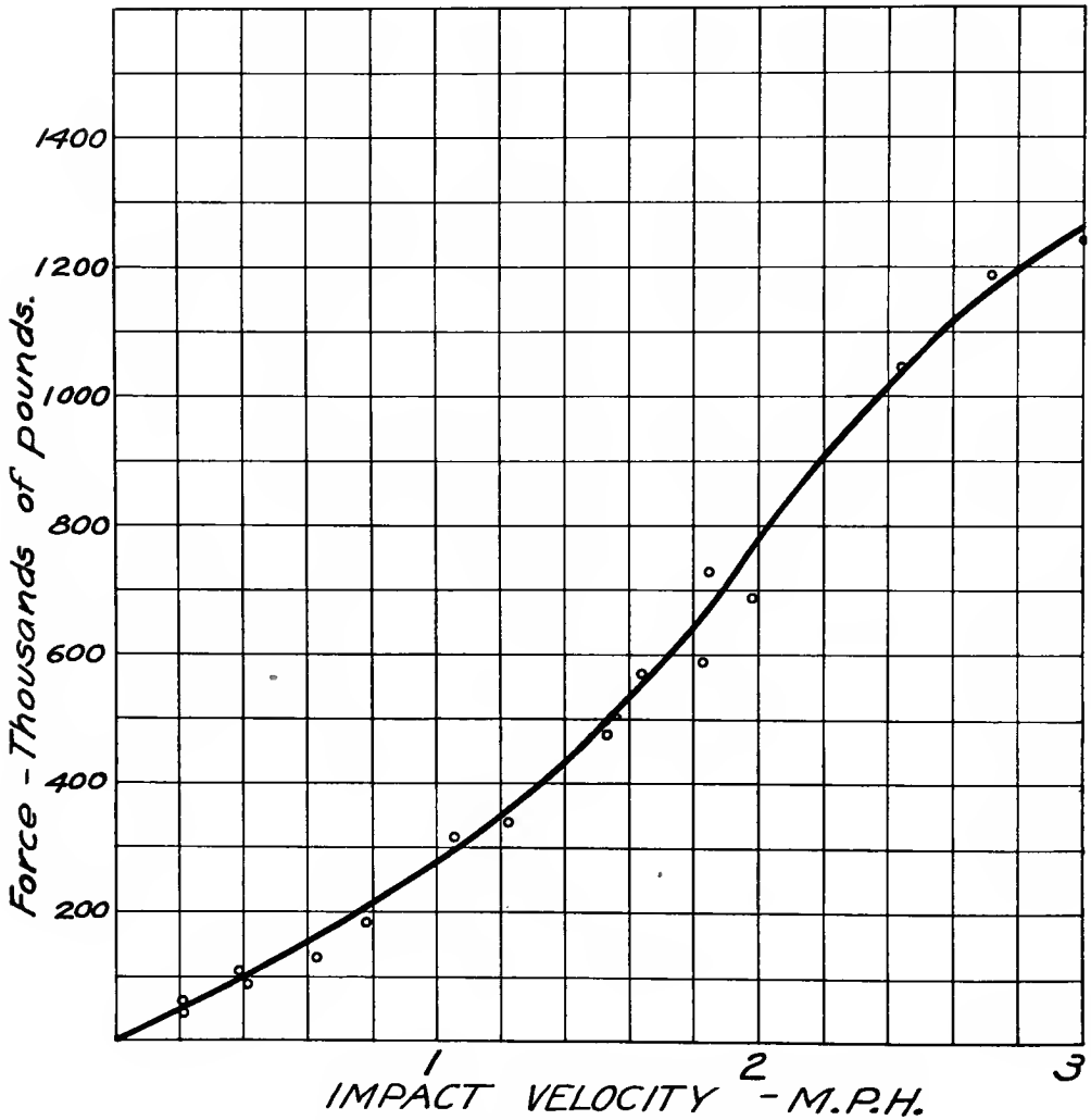
FIG. 60—PLOT OF FORCE AT VARYING IMPACT VELOCITIES
