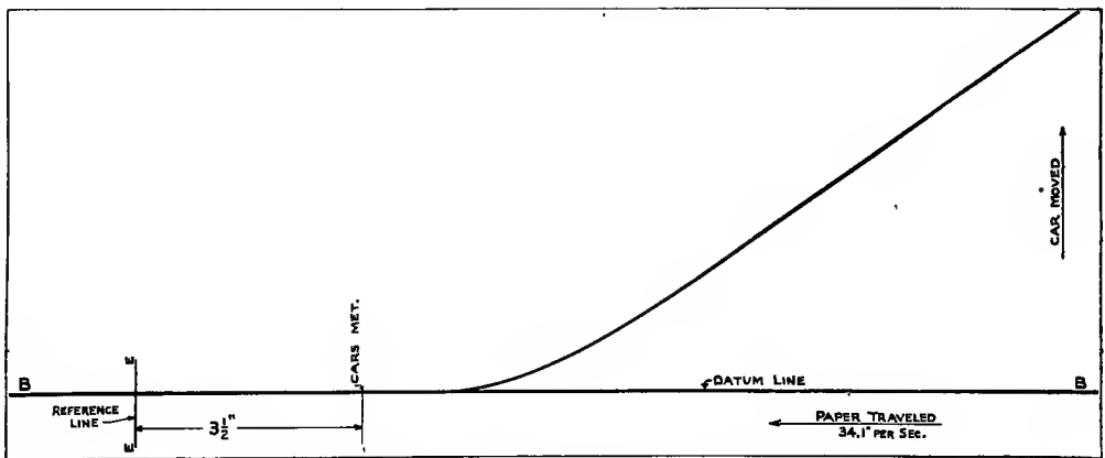
FIG. 55—SPECIMEN CAR-MOVEMENT CARD FROM DRUM B
