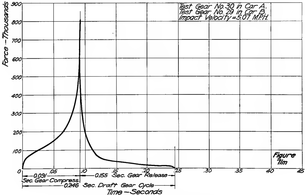
FIGS. 71K AND 71M—TIME-FORCE CURVES, NATIONAL H-1 GEARS
