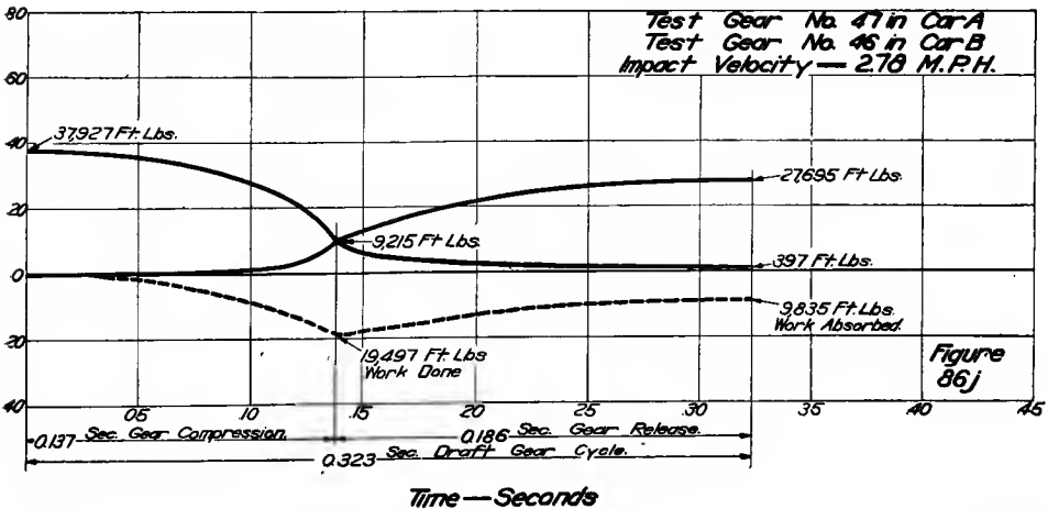
FIGS. 86G AND 86J—ENERGY CURVES, BRADFORD K GEARS
