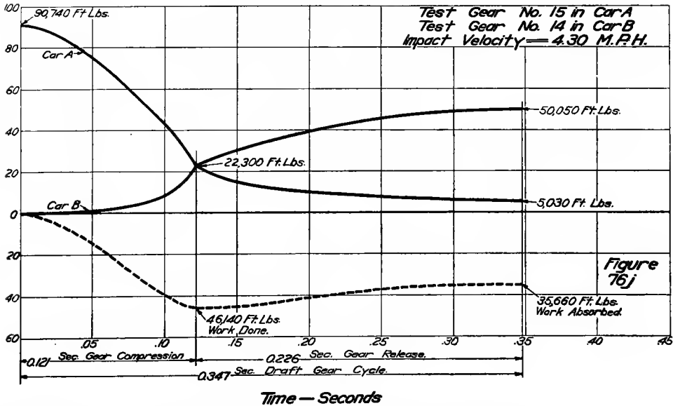
FIGS. 76C AND 76J—ENERGY CURVES, SESSIONS JUMBO GEARS
