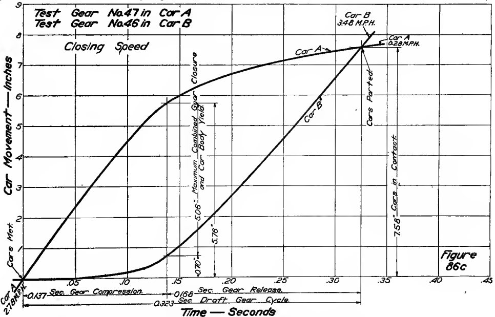
FIGS., 86A, 86B AND 86C—CAR-MOVEMENT CURVES, SUPERIMPOSED. BRADFORD K GEARS THESE CURVES DRAWN BY CARS IN TESTS
