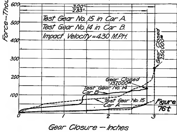
FIGS. 76R AND 76T—FORCE-CLOSURE DIAGRAMS SESSIONS JUMBO GEARS
