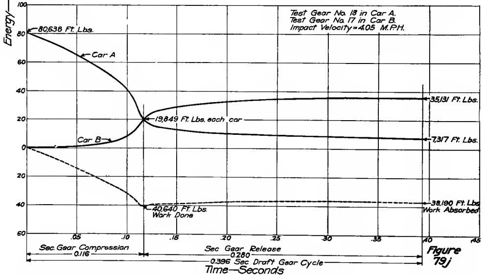
FIGS. 79C, 79H AND 79J—ENERGY CURVES, CARDWELL G-25-A GEARS
