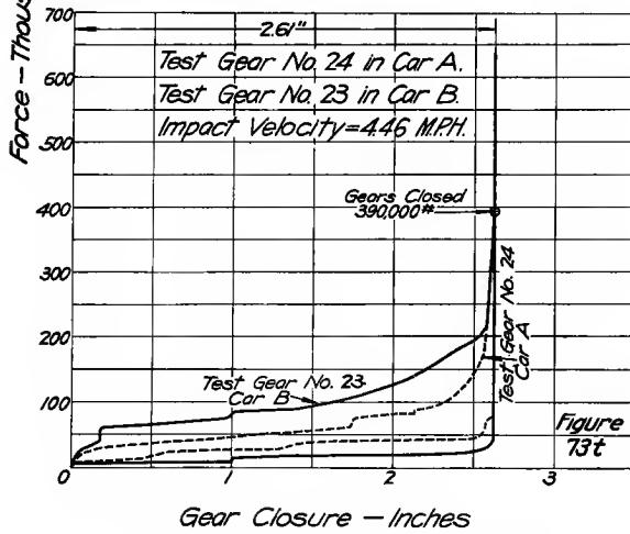
FIGS. 73R AND 73T—FORCE-CLOSURE DIAGRAMS MINER A-18-S GEARS
