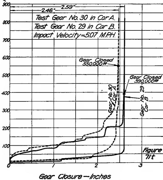
FIGS. 71R AND 71T—FORCE-CLOSURE DIAGRAMS, NATIONAL H-1 GEARS
