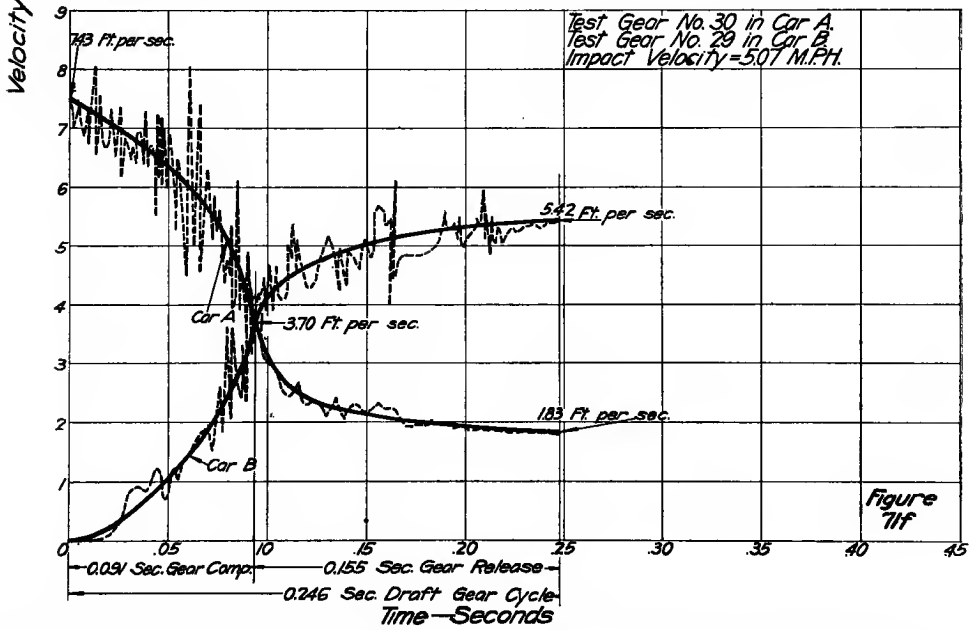
FIGS. 7Id, 7Ie AND 7If--VELOCITY CURVES, NATIONAL H-1 GEARS
