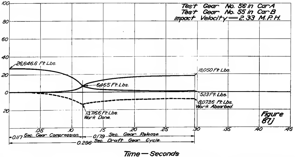
FIGS. 87C AND 87J—ENERGY CURVES, HARVEY SPRINGS
