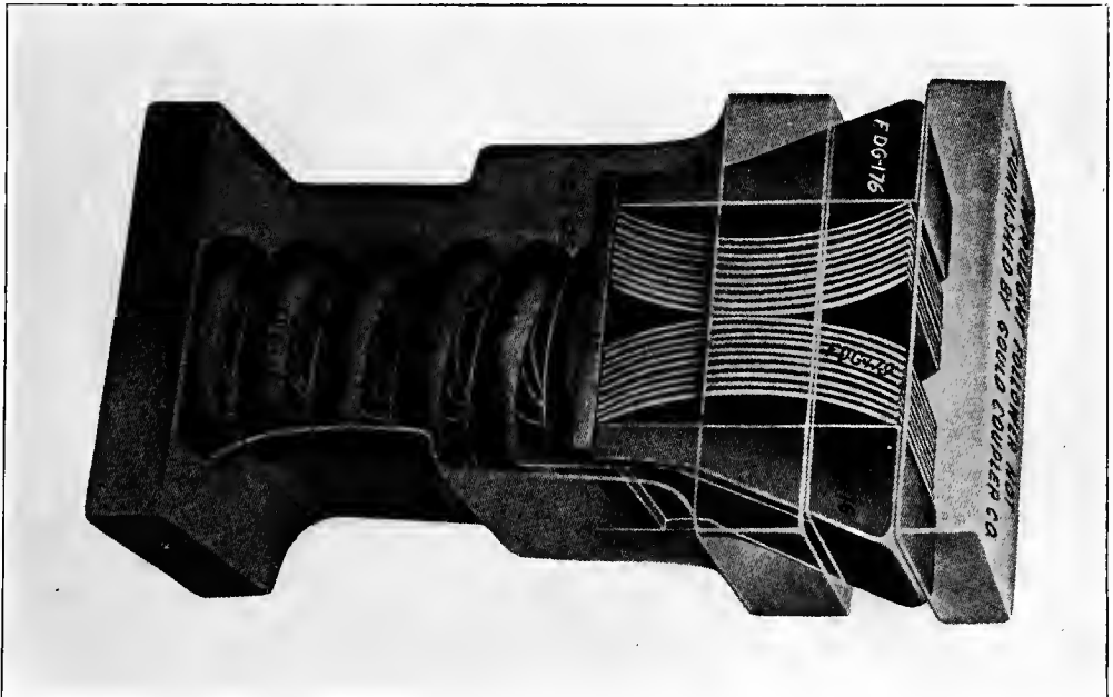
FIG. 11—GOULD TYPE 175 GEAR
