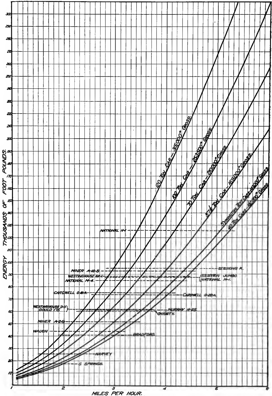
FIG. 68—ENERGY CURVES FOR CARS OF VARIOUS WEIGHTS, WITH COMMERCIAL GEAR CAPACITIES INDICATED
