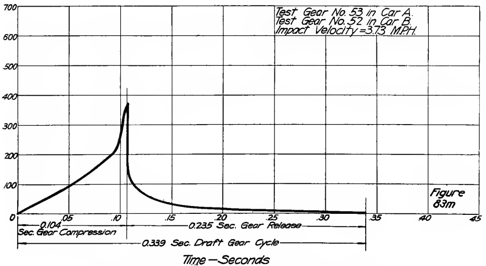
FIGS. 83K AND 83M—TIME-FORCE CURVES, CHRISTY GEARS
