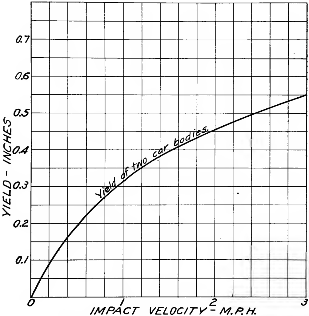
FIG. 59—PLOT OF CAR BODY YIELD AT VARYING IMPACT VELOCITIES
