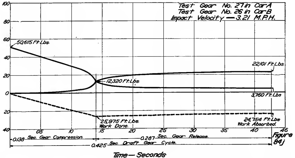
FIGS. 84G AND 84J—ENERGY CURVES, MINER A-2-S GEARS
