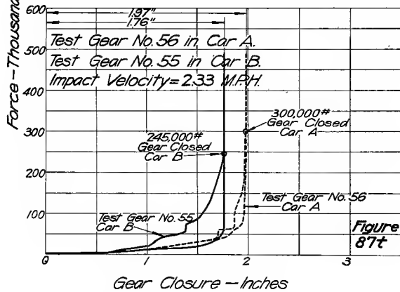
FIGS. 87R AND 87T—FORCE-CLOSURE DIAGRAMS, HARVEY SPRINGS
