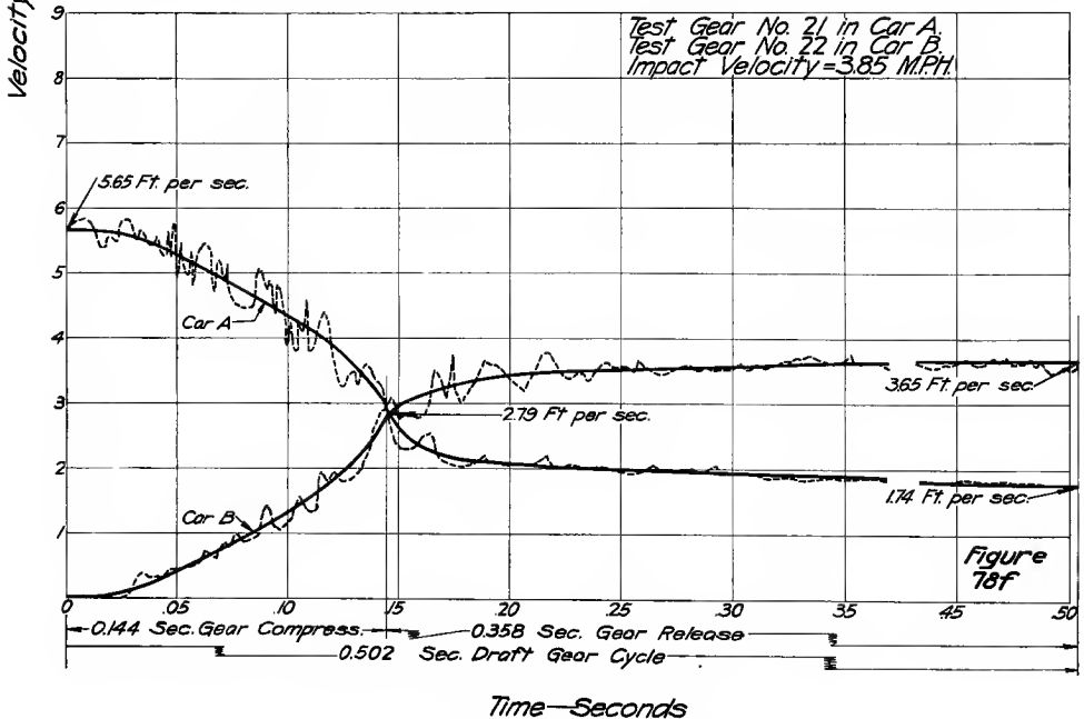
FIGS. 78D, 78E AND 78F—VELOCITY CURVES, CARDWELL G-18-A GEARS
