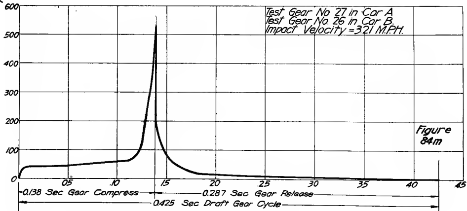
FIGS 84K AND 84M—TIME-FORCE CURVES, MINER A-2-S GEARS
