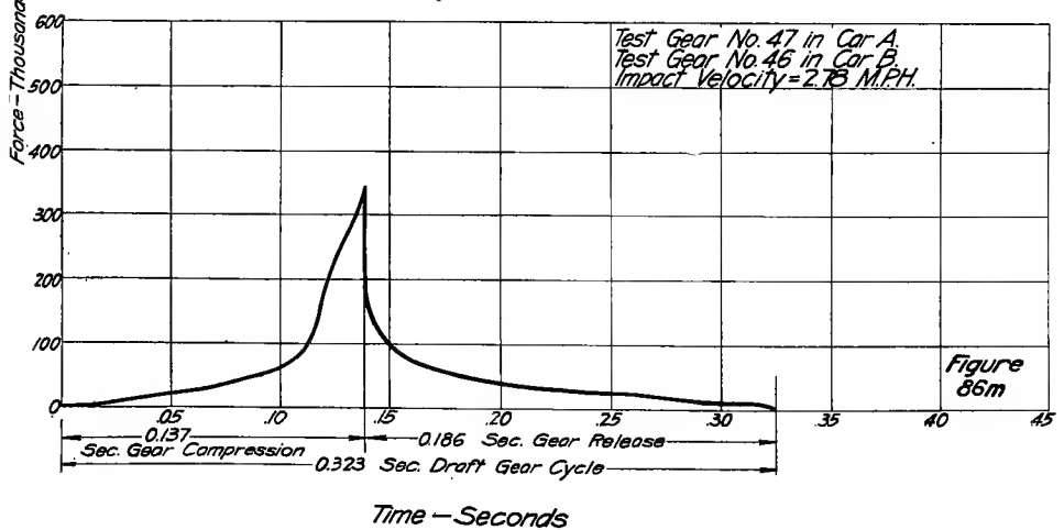
FIGS. 86K AND 86M—TIME-FORCE CURVES, BRADFORD K GEARS
