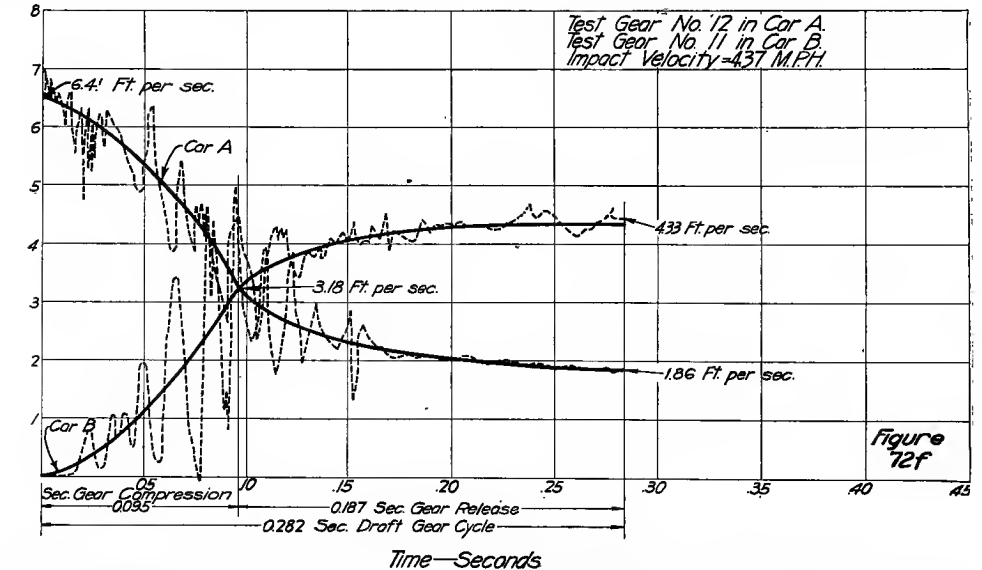
FIGS. 72D, 72E AND 72F—VELOCITY CURVES, SESSIONS K GEARS
