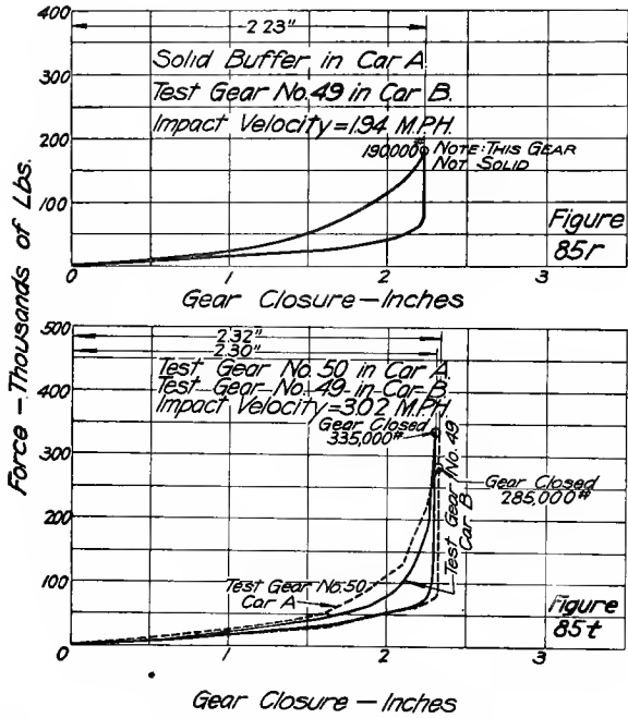
FIGS. 85R AND 85T—FORCE-CLOSURE DIAGRAMS, WAUCH PLATE GEARS
