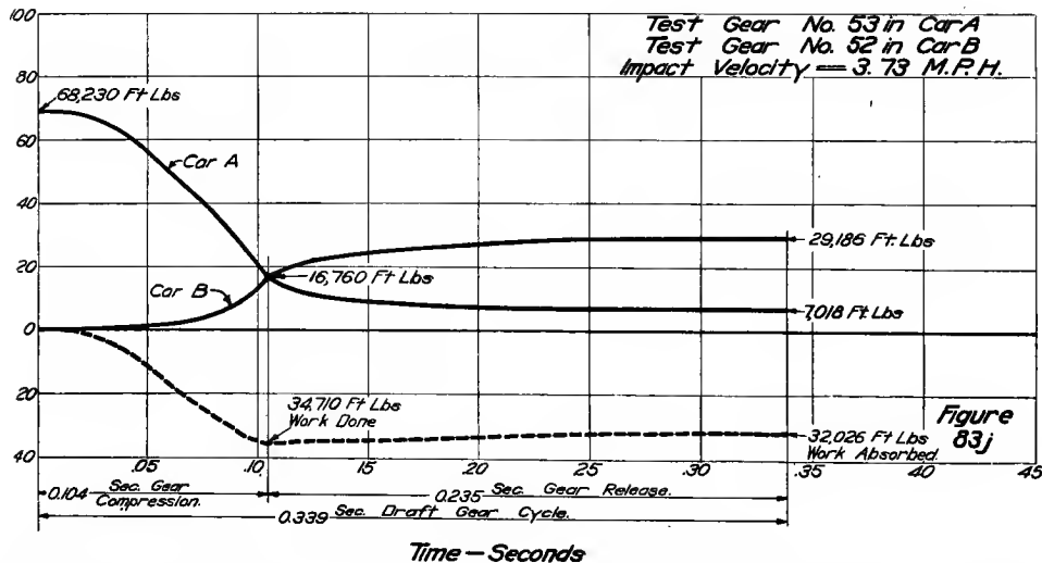
FIGS. 83C AND 83J—ENERGY CURVES, CHRISTY GEARS
