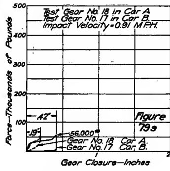
FIGS. 79R, 79S AND 79T—FORCE-CLOSURE DIAGRAMS, CARDWELL G-25-A GEARS
