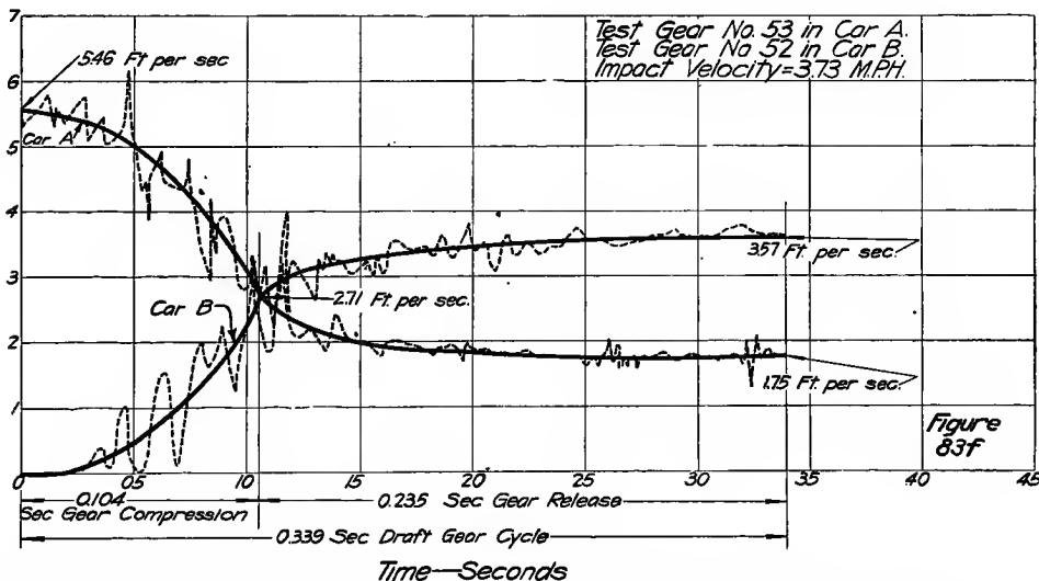
FIGS. 83D, 83E AND 83F—VELOCITY CURVES, CHRISTY GEARS
