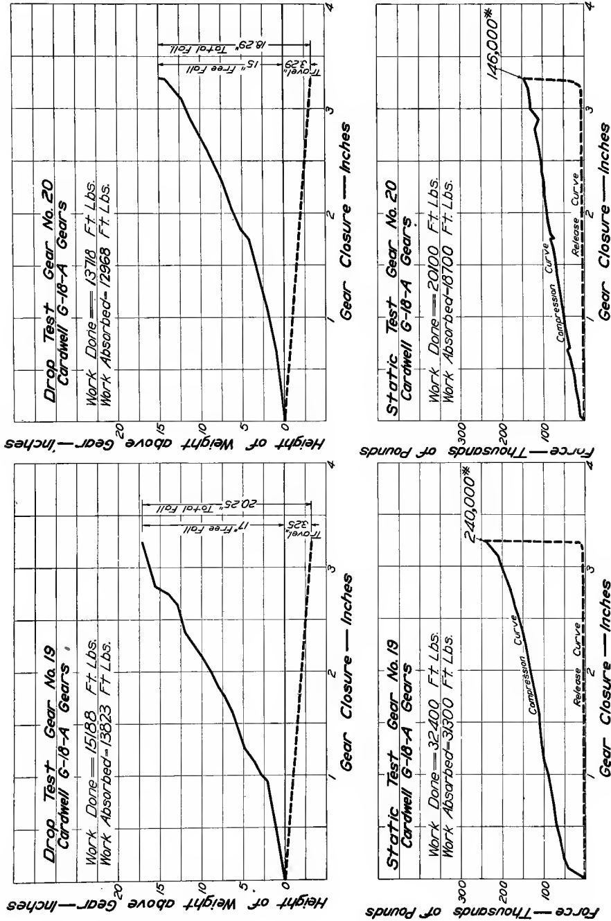
FIG. 23—DROP TEST AND STATIC TEST DIAGRAMS, CARDWELL TYPE C-18-A
