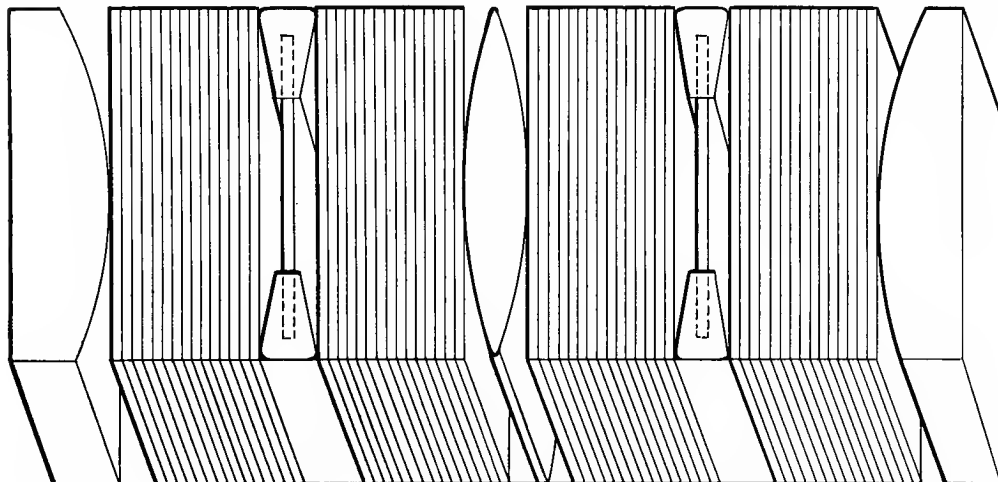
FIG. 13—WAUGH PLATE GEAR
