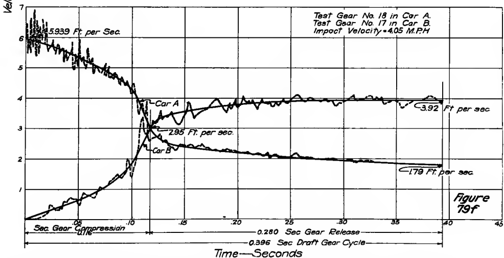
FIGS. 79D, 79E AND 79F—VELOCITY CURVES, CARDWELL G-25-A GEARS
