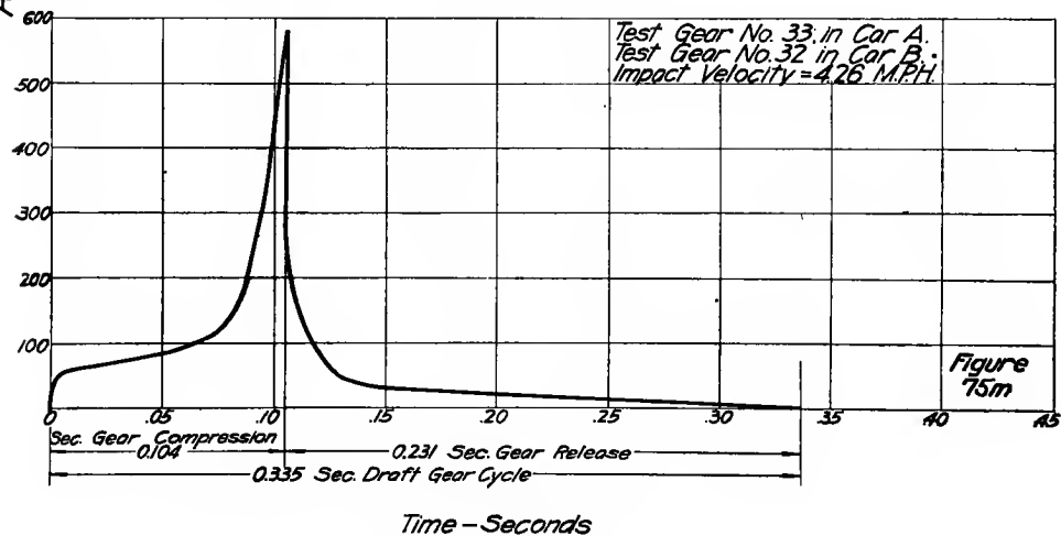
FIGS. 75K AND 75M—TIME-FORCE CURVES, NATIONAL M-1 GEARS
