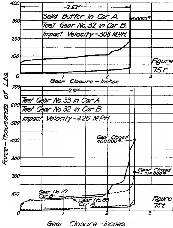
FIGS. 75R AND 75T—FORCE-CLOSURE DIAGRAMS, NATIONAL M-1 GEARS
