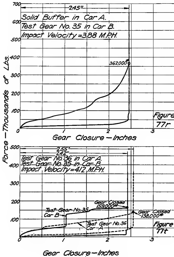
FIGS. 77R AND 77T—FORCE-CLOSURE DIAGRAMS NATIONAL M-4 GEARS
