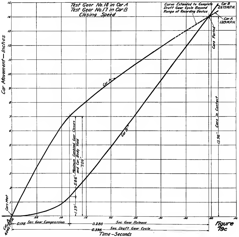
FIGS. 79B AND 79C—CAR-MOVEMENT CURVES, SUPERIMPOSED. CARDWELL G-25-A GEARS THESE CURVES DRAWN BY CARS IN TESTS
