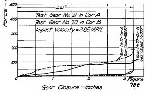
FIGS. 78R AND 78T—FORCE-CLOSURE DIAGRAMS CARDWELL G-18-A GEARS
