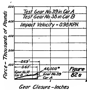
FIGS. 82r, 82s AND 82t—FORCE-CLOSURE DIAGRAMS, MURRAY H-25 GEARS
