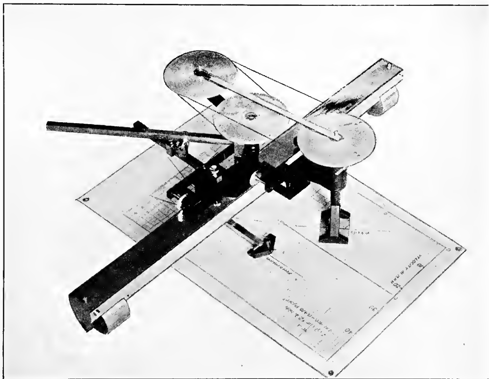
FIG. 57—MECHANICAL DIFFERENTIATING MACHINE
