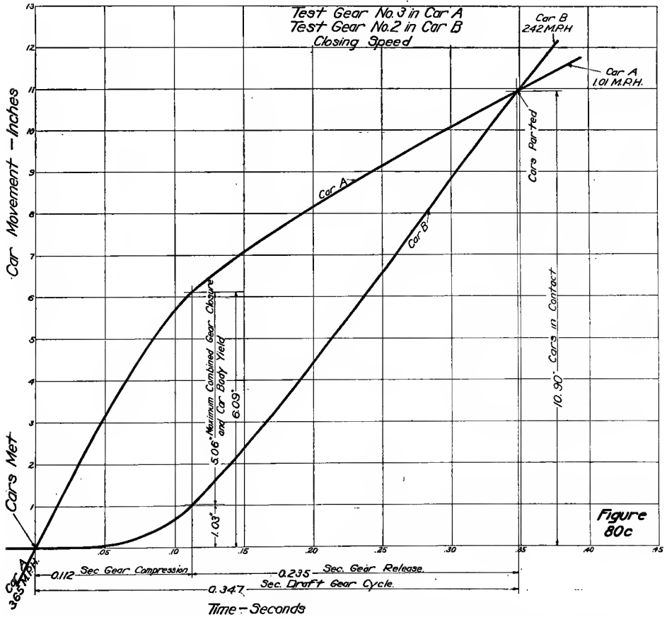
FIGS. 80B AND 80C—CAR-MOVEMENT CURVES, SUPERIMPOSED. WESTINGHOUSE D-3 GEARS THESE CURVES DRAWN BY CARS IN TESTS
