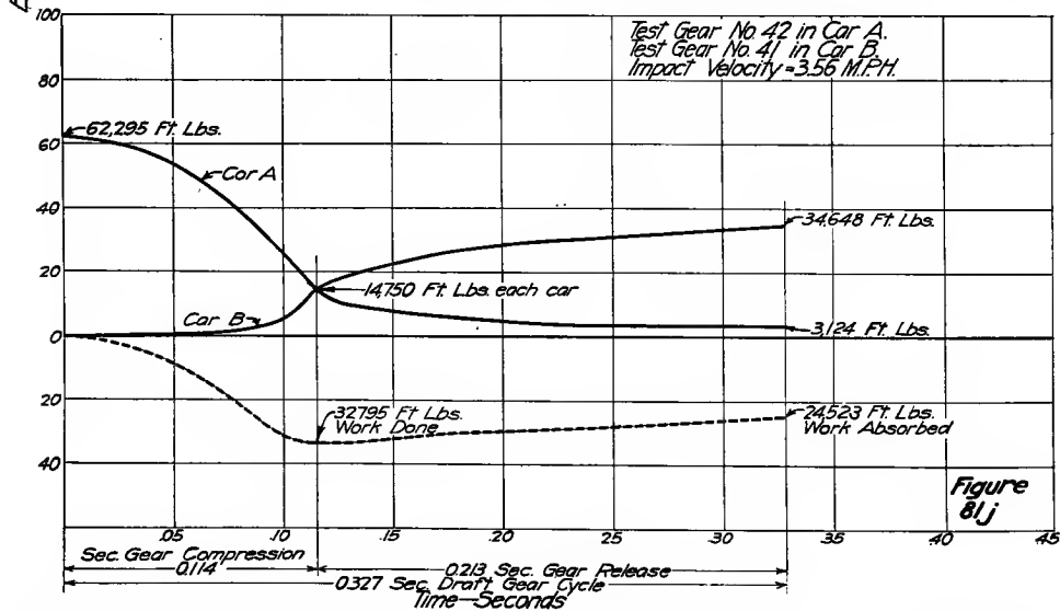
FIGS. 81G, 81H AND 81J--ENERGY CURVES, GOULD NO. 175 GEARS
