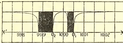
FIG. 5. m = \cdot003 .
