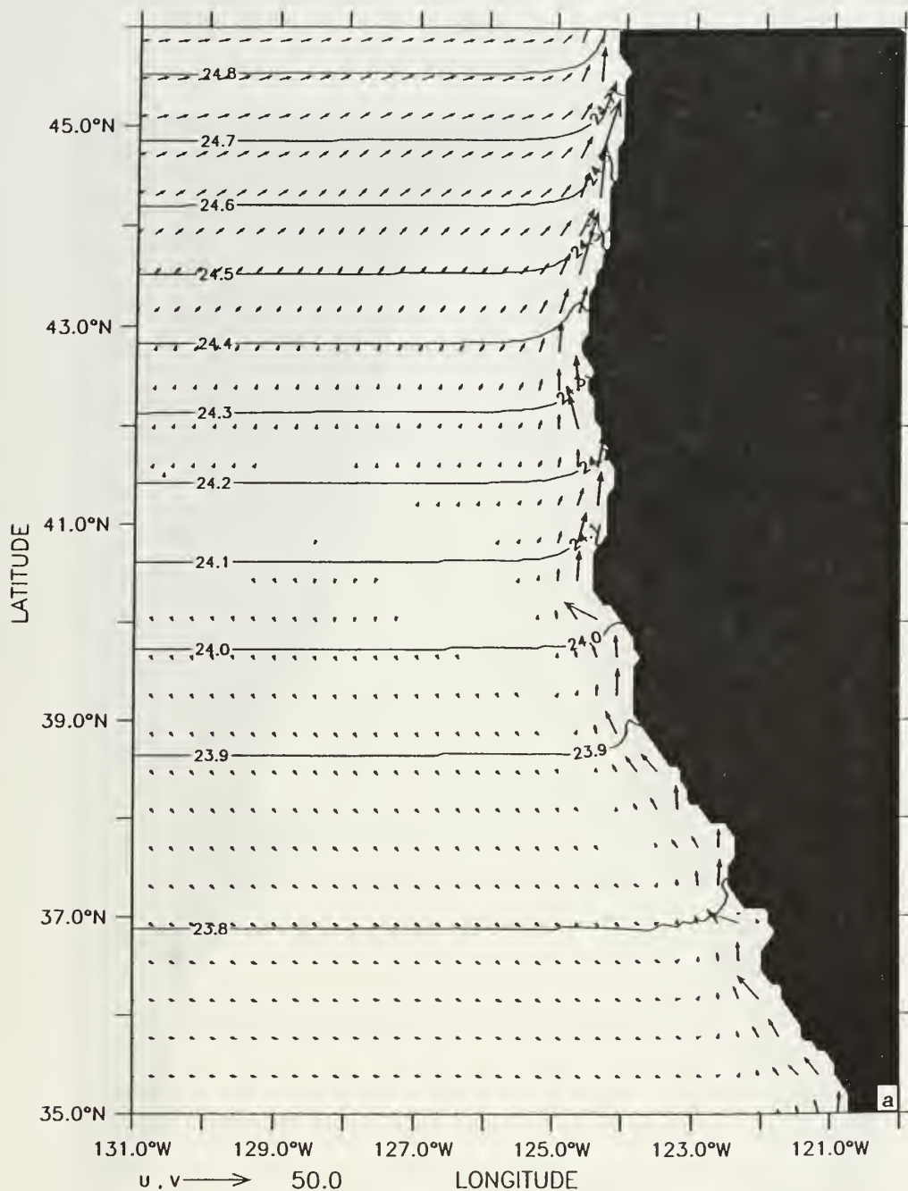
Figure 5. Day 3 density contours and velocity vectors at 13 m depth for (a) the northern half and (b) the southern half of the model domain. Contour interval is 0.1 g/cm 3 ; maximum velocity vector is 50 cm/s. In this and the following figures, to avoid clutter, vectors are plotted at every third or fourth grid point in the cross-shore and alongshore directions, and velocities less than 5 cm/s are not plotted.
