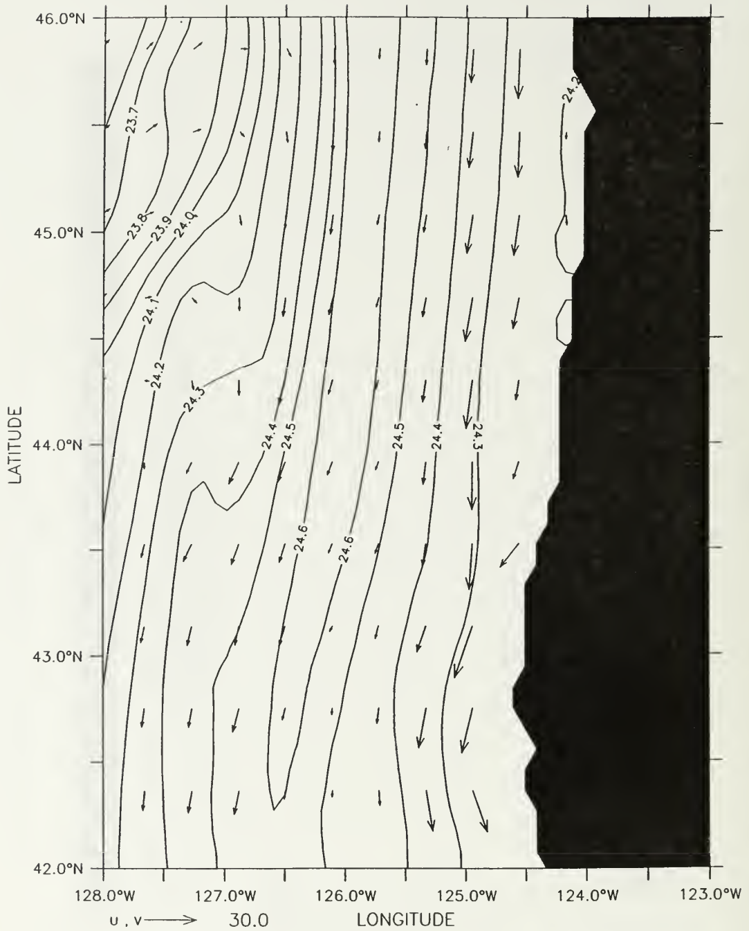
Figure 13. Day 300 density contours and velocity vectors at 13 m depth for the northern portion of the domain from 42° N to 46° N. Contour interval is 0.1 g/cm 3 ; maximum velocity vector is 30 cm/s.
