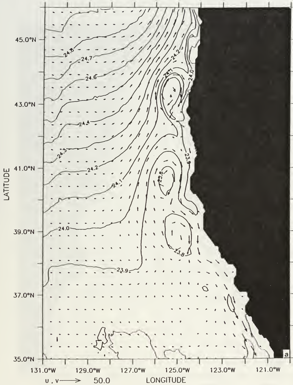
Figure 9. Day 105 density contours and velocity vectors for the northern (a,c) and southern (b,d) portions of the model domain at depths 13 m (a,b) and 316 m (c,d). Contour interval is 0.1 \text{ g/cm}^3 ; maximum velocity vector is 50 \text{ cm/s} in (a) and (b), and 20 \text{ cm/s} in (c) and (d).
