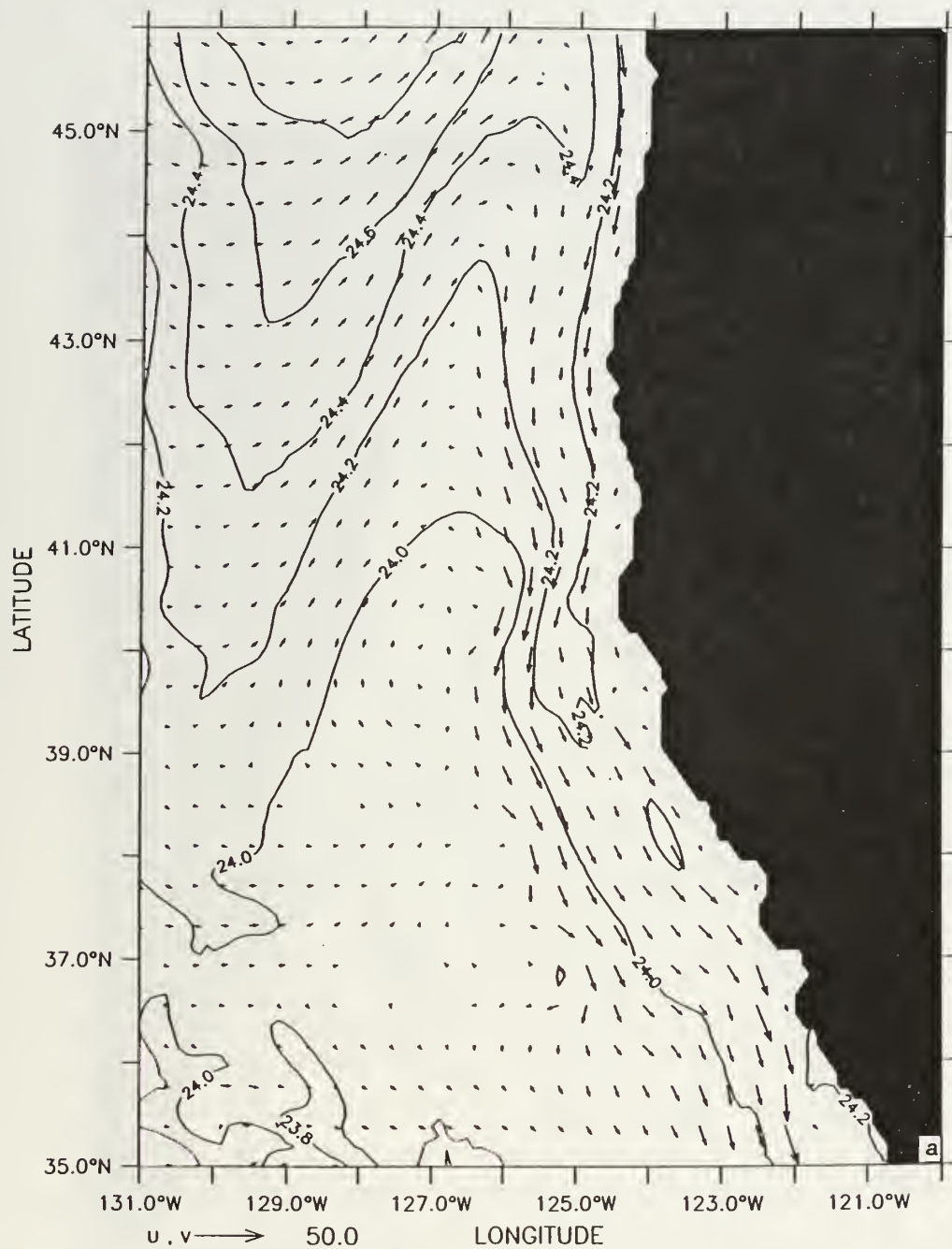
Figure 10. Day 195 density contours and velocity vectors for the northern (a,c) and southern (b,d) portions of the model domain at depths 13 m (a,b) and 316 m (c,d). Contour interval is 0.2 \text{ g/cm}^3 in (a) and (b), and 0.1 \text{ g/cm}^3 in (c) and (d); maximum velocity vector is 50 \text{ cm/s} in (a) and (b) and 20 \text{ cm/s} in (c) and (d).
