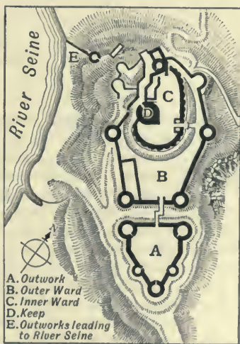
PLAN OF CHÂTEAU GAILLARD.
