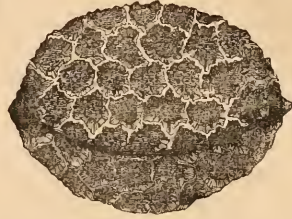
Fig. 9. Seed of Eschscholtzia Californica , \times 40 .
