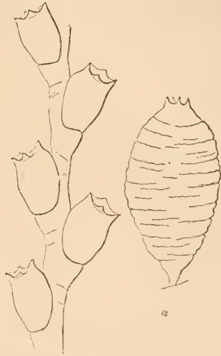
Fig. 149. Sertulariella polyzonias , magnified. a. capsule.
