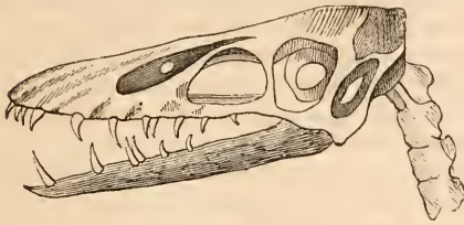
Fig. 226. Head of Pterodactyle.
