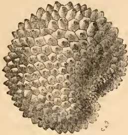
Fig. 102. Seed of Saponaria Calabrica , x 40.
