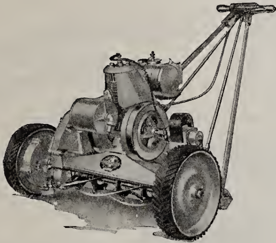
4-Acre Power Lawn Mower
