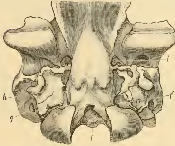
FIGURE 195.—Skull of Uintatherium robustum , Leidy (type specimen); bottom view of back part of skull. f , foramen unguam; f , occipital foramen; g , stylo-mastoid foramen; h , foramen lacernum; i , vascular foramen in basisphenoid.
