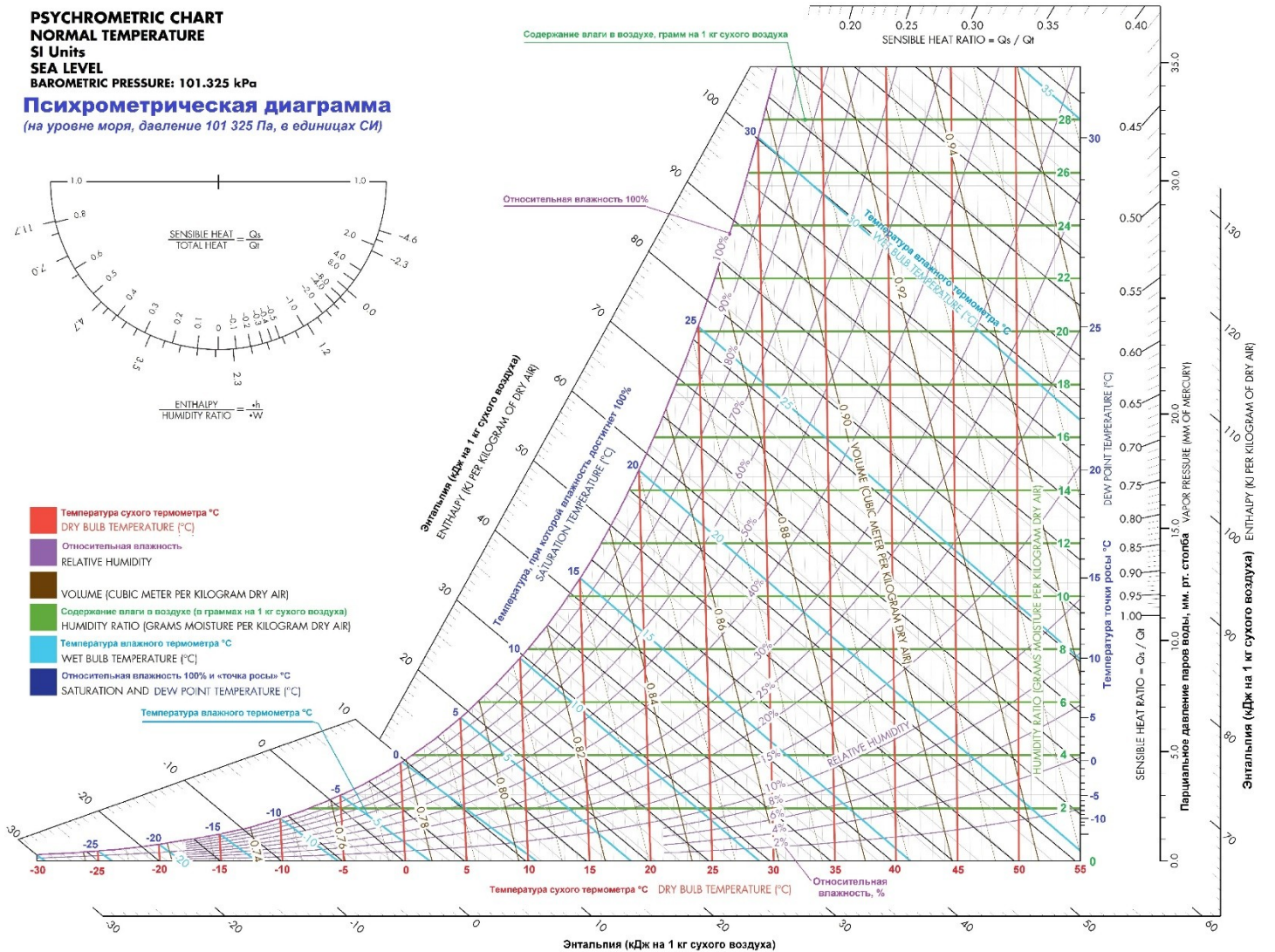
Figure 5-1. The psychrometric chart (adapted from ISO [1993] and Coolerado [2012])
