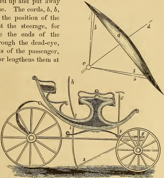
VINEY AND POCOCK'S CHARVOLANT.
