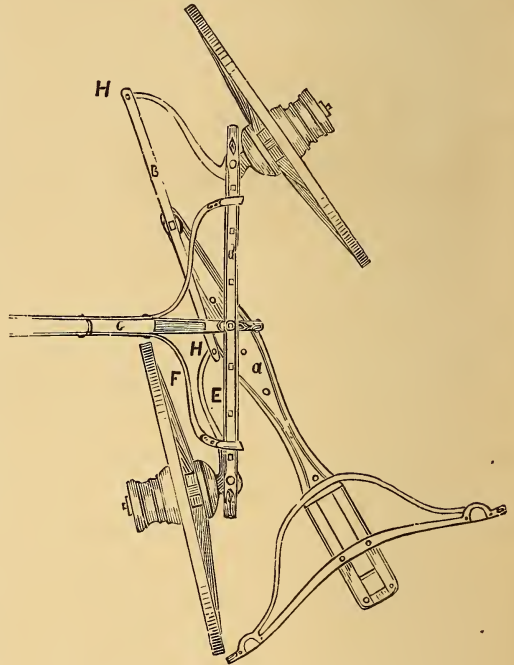
ACKERMAN'S MOVABLE AXLE.
