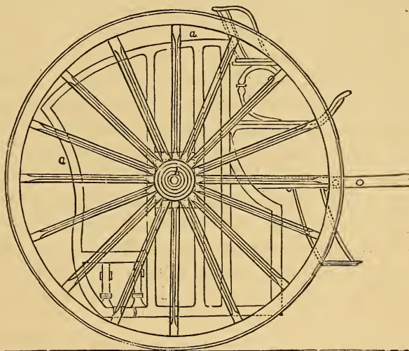
HANSOM'S CAB. 1
