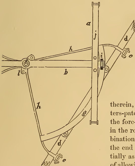
EVERETTS' PERCH-COUPLING.
