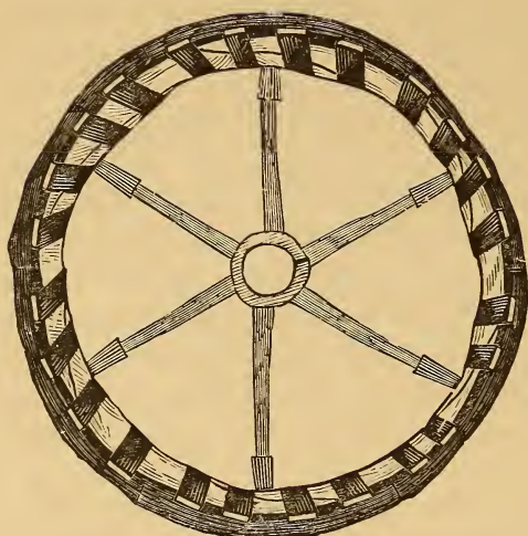
COMPLETED CHARIOT WHEEL.
