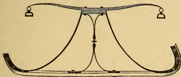
TILBURY SPRING.—REAR VIEW.
