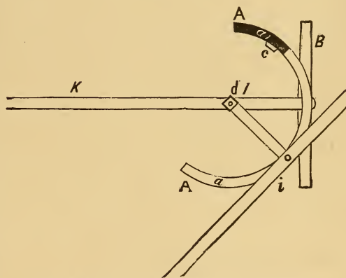
ANOTHER HAUSSKNECHT COUPLING.
