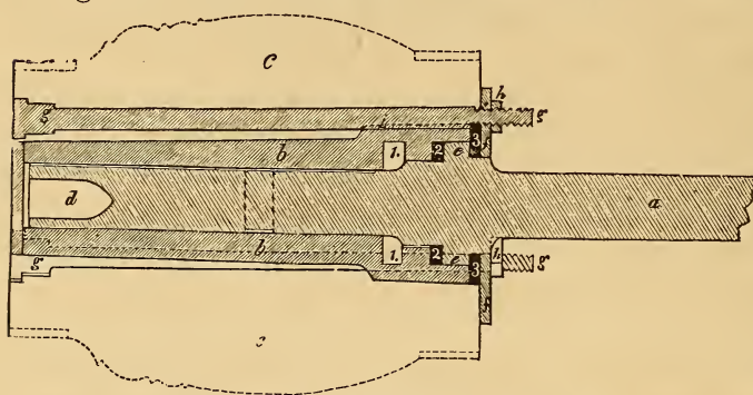
STRATTON'S PATENT MAIL-AXLE.
