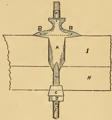
PHELPS'S KING-BOLT.
