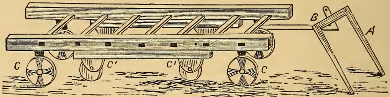
CART AND WAGON COMBINED, 1797.
