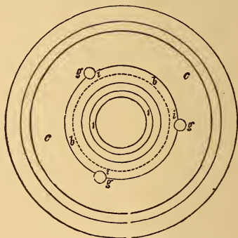
MAIL-AXLE COLLAR-PLATE.
