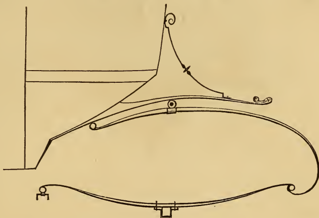
IMPROVED SCROLL-SPRING.
