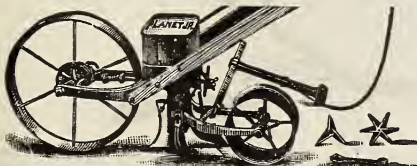
No. 3 Planet Jr. Hill and Drill Seeder, Holds 3 Quarts, Weight 43 lbs., $17.50.
