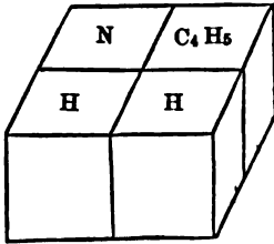
Ethylamine.
