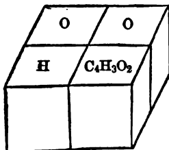
Acetic Acid.
