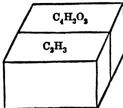
Acetone.
