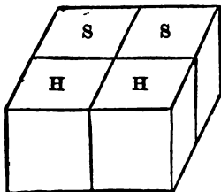
Acetic Acid.
