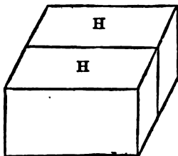
HYDROGEN TYPE.
