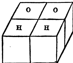
THE TYPE—WATER.
