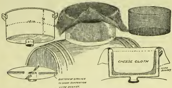
FIG. 123. — Honey strainer.
