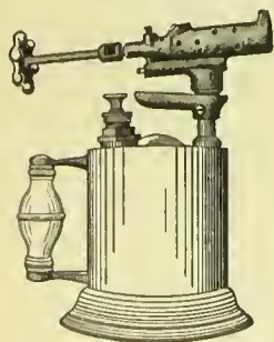
FIG. 169.—Gasoline torch.
