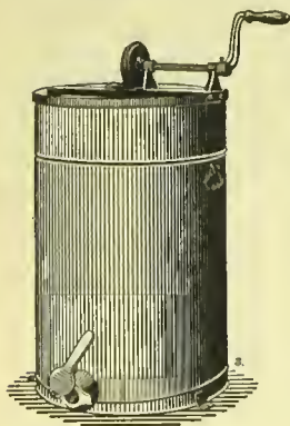
FIG. 121. — Extractor with stationary can.
