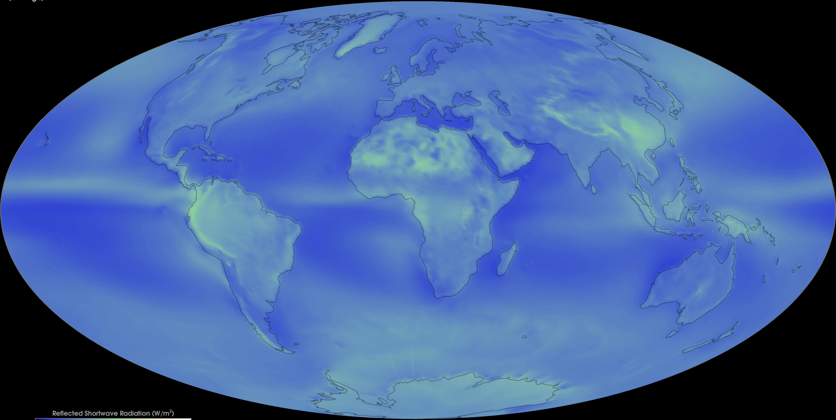
Reflected Shortwave Radiation (average)
