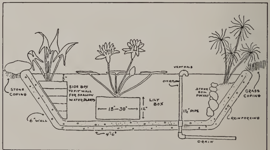
Section showing construction and planting. This type of pool is easy to build and will give satisfaction.
