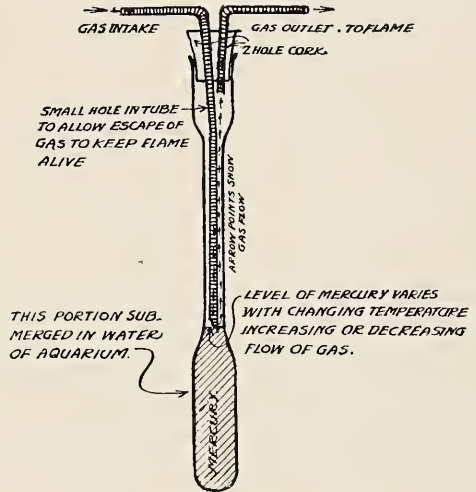
Aquarium Thermostat
