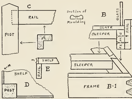
Construction Details
