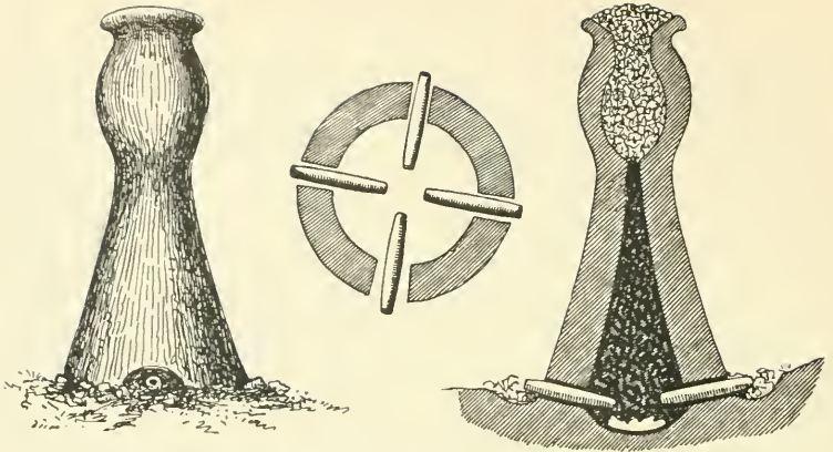
FIG. 12.—Primitive smelting furnace with four blast-pipes. Jur of the Upper Nile (after Schurtz).
