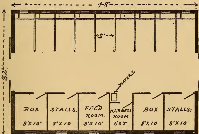
GROUND PLAN OF HORSE BARN
