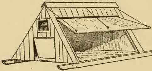
MOVABLE HOG SHELTER
