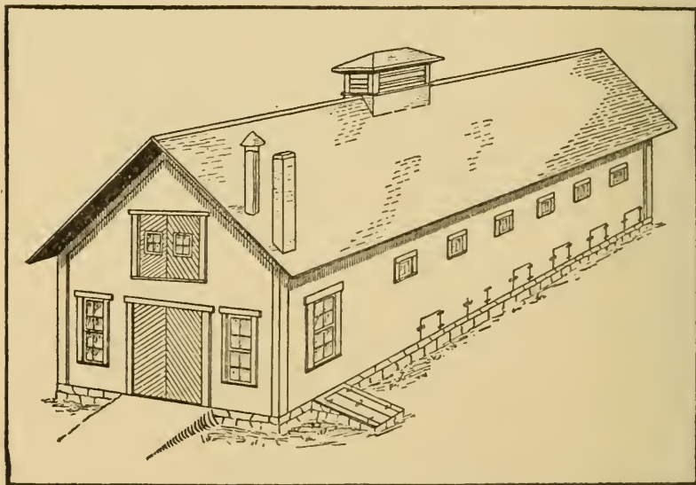
ELEVATION OF HOG HOUSE
