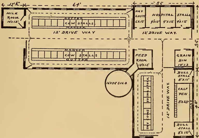
GROUND PLAN OF DAIRY BARN
