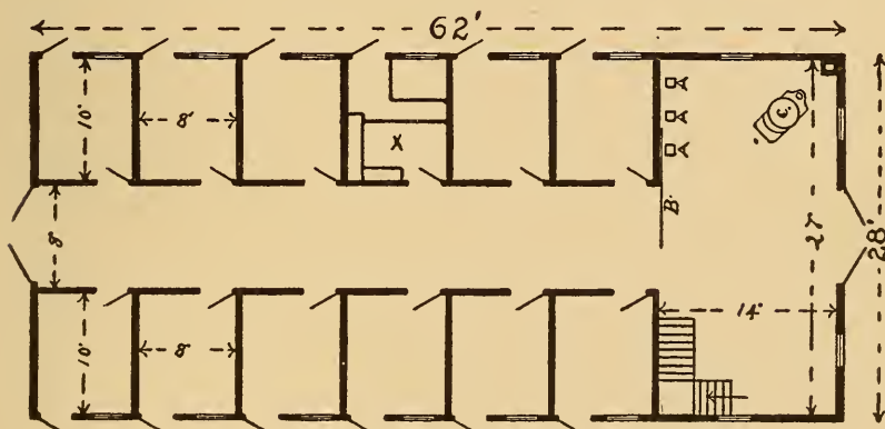
FLOOR PLAN OF HOG HOUSE.
