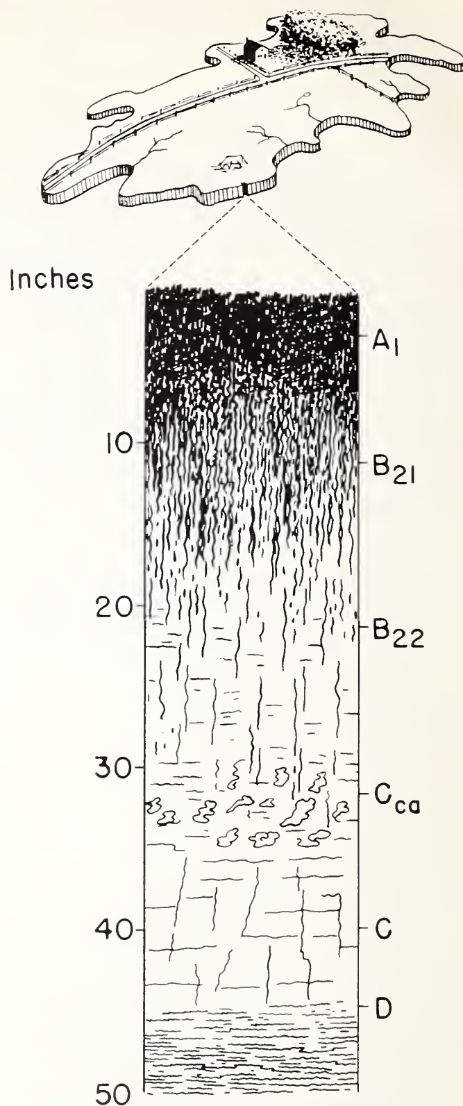
Figure 3.—Solid horizons, or layers, in Morton silt loam.
