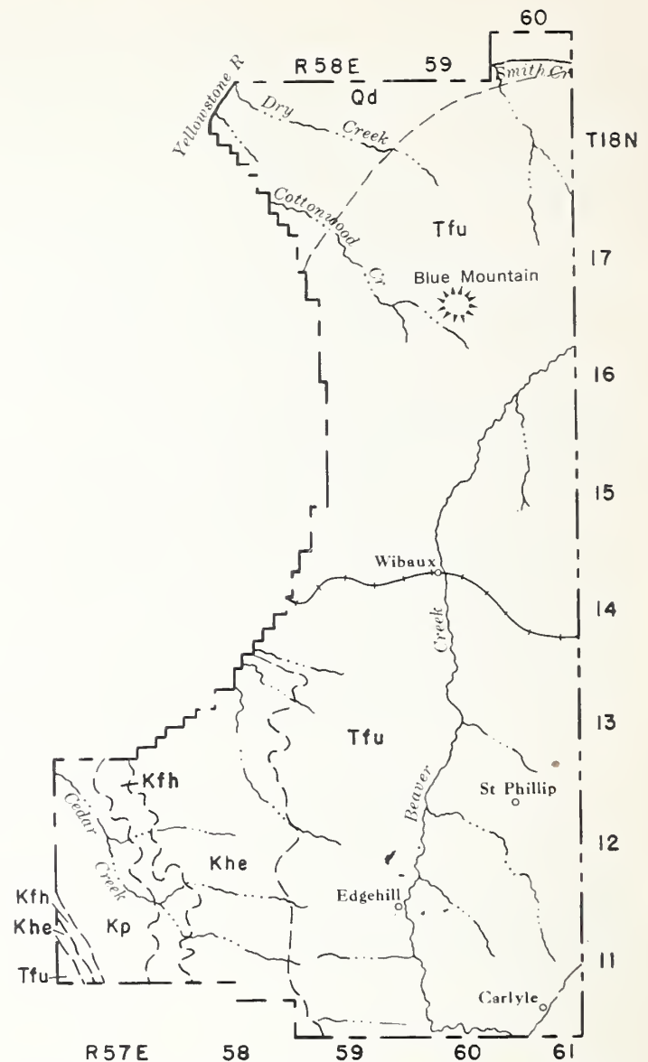
Figure 18.—Geological formation of Wibaux County, Mont.: Qd, Border of continental ice sheet; glacial drift. Tfu, Fort Union formation; includes the Tongue River member, Lebo shale member, and Tullock member. Khe, Hell Creek formation. Kfh, Fox Hills sandstone. Kp, Bearpaw shale.
