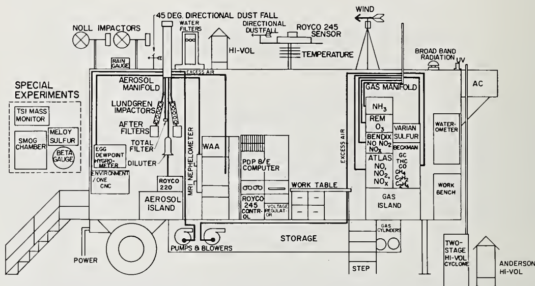
Figure 12. Schematic of a large mobile air pollution laboratory constructed for the Air Resources Board of the State of California. This laboratory includes a comprehensive array of automatic aerosol size analyzers, particle samplers, gas analyzer, and meteorological instruments (Whitby et al. , 1973).
