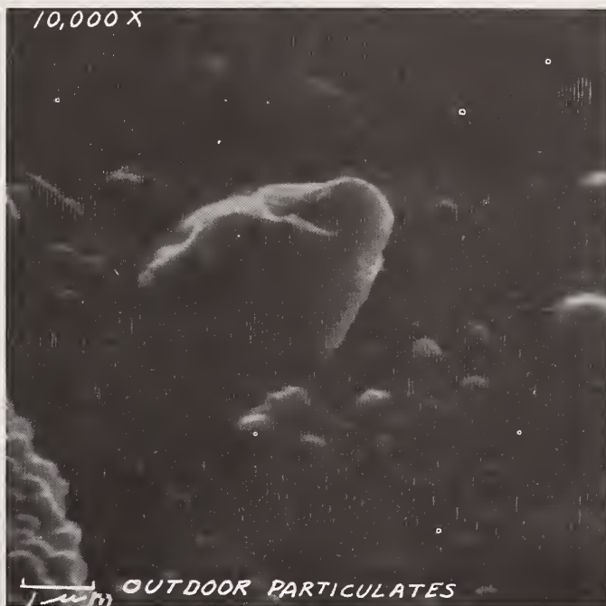
Figure 8. 10,000X SEM of impaction area of smog sample (same as in fig. 7).
