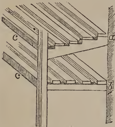
Fig. 25. Section showing the arrangement of the Shelves.
