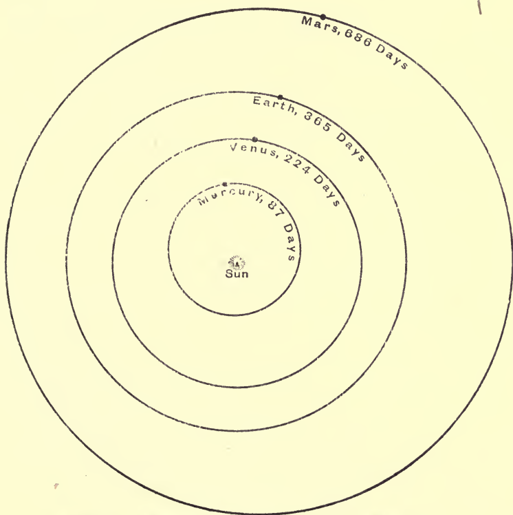
ORBITS OF MARS, THE EARTH, VENUS, AND MERCURY.
