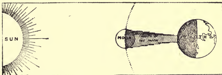
AN ECLIPSE OF THE SUN.
