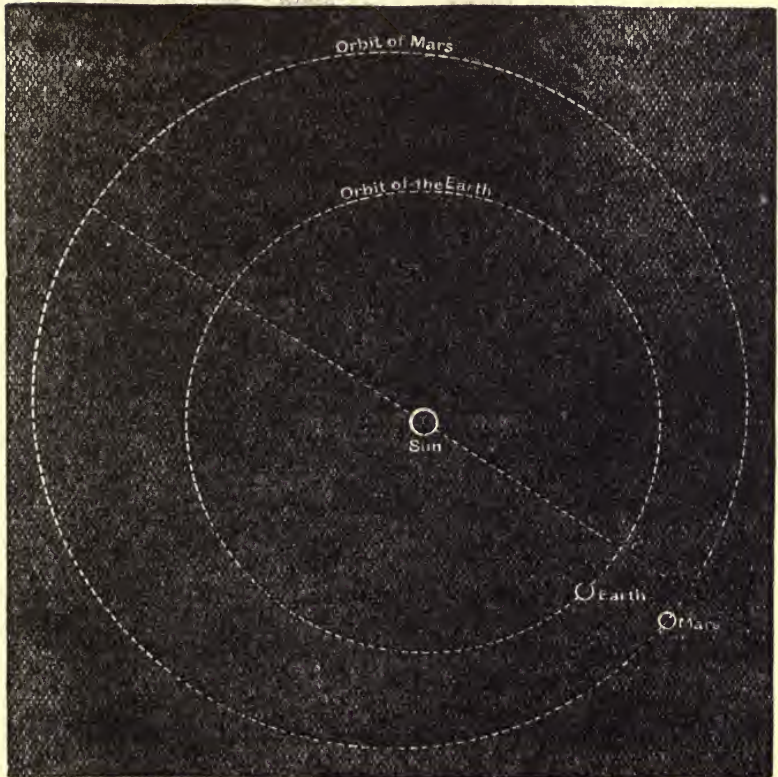
ORBITS OF THE EARTH AND MARS.
