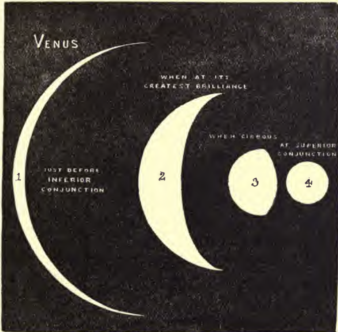
DIFFERENT PHASES OF VENUS.
