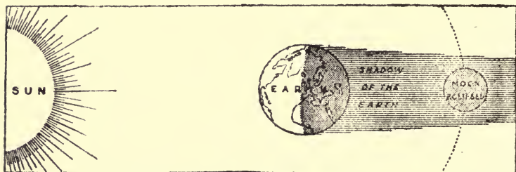
AN ECLIPSE OF THE MOON.
