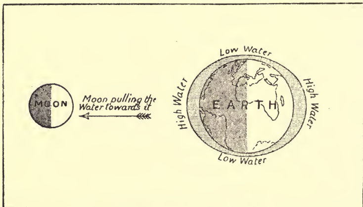
THE MOON RAISING THE TIDES.
