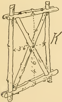
Fig. 315. K Frame (make one).
