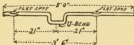
Fig. 284. The Crank Shaft.
