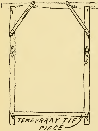
Fig. 101. The King Post Frame.
