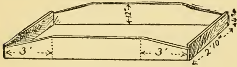
Fig. 59. Frame of the Scow.
