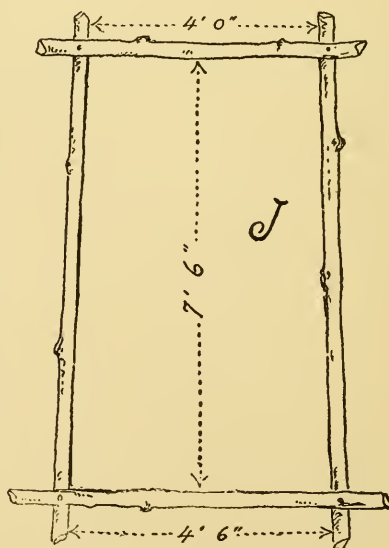
Fig. 314. J Frame (make one).
