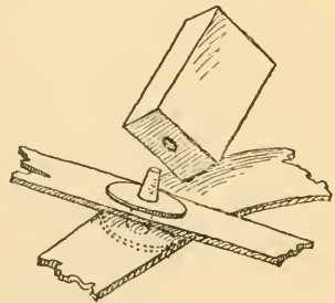
Fig. 214. Riveting the Straps Together.
