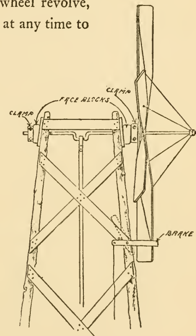
Fig. 290. Side View of the Wind Wheel, showing Brake.
