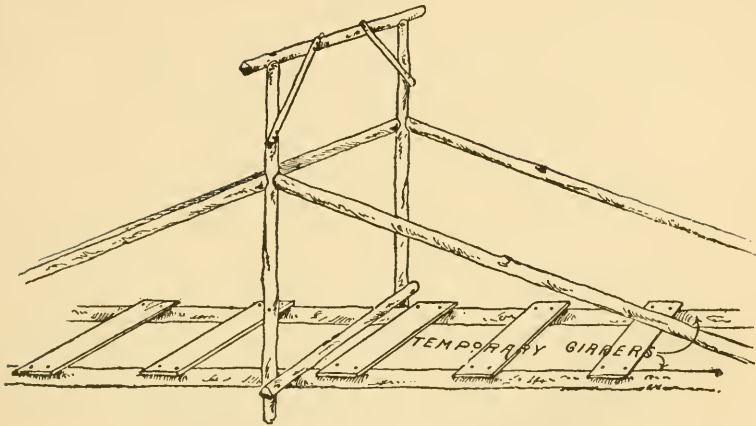
Fig. 102. The King Posts Set in Position.
