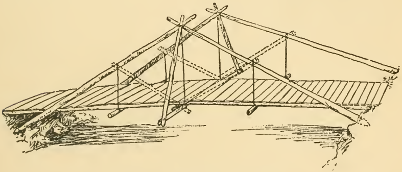
Fig. 100. The King Rod Bridge.
