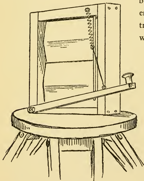
Fig. 158. General View of Screen.
