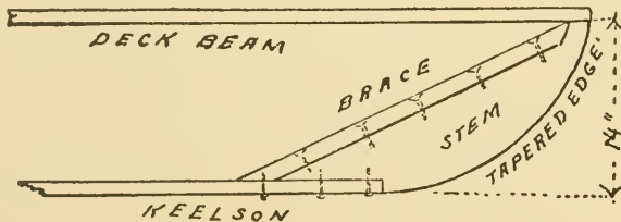
Fig. 105. Stem of the Canoe.
