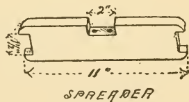
Fig. 174. A Spacing Block.
