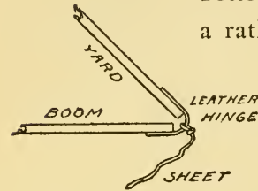
Fig. 12. Hinge for Spars.
