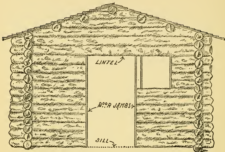
Fig. 272. The Finished Roof.
