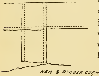
Fig. 38 The Sail Stitch.
