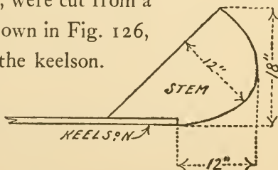
Fig. 126. The Stem Piece.
