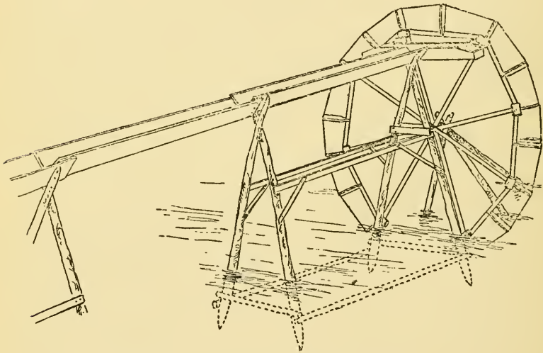
Fig. 260. The Water Wheel in Action.
