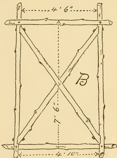
Fig. 306. B Frame (make four).
