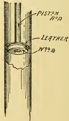
Fig. 293. The Piston Valve.
