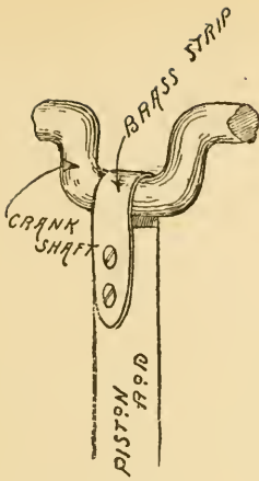
Fig. 294. Connection of Rod and Crank.
