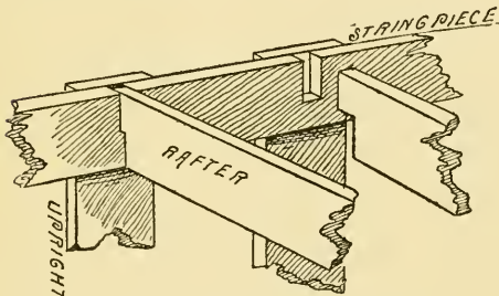
Fig. 185. Notching in the Rafters.
