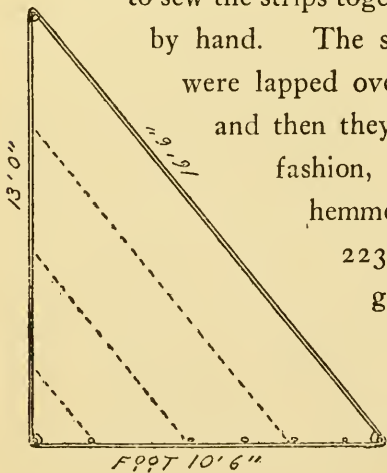
Fig. 222. Leg-of-Mutton Sail.
