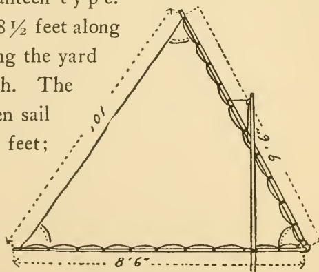
Fig. 118. The Mainsail.
