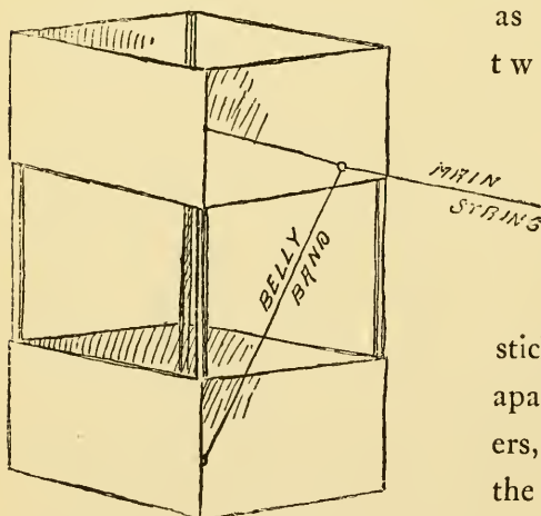
Fig. 249. The Diamond Box Kite.
