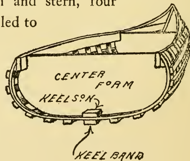
Fig. 128. Section at Center of Canoe.
