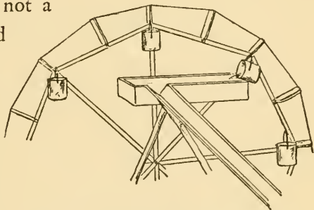
Fig. 263. Mr. Halliday's Water Wheel.
