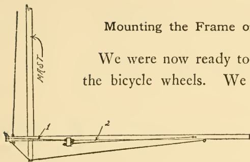
Fig. 219. Bracing the Mast.
