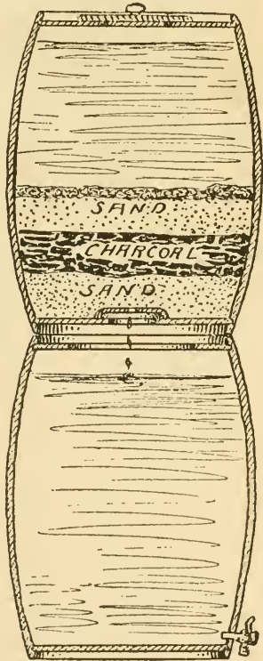
Fig. 69. The Barrel Filter.
