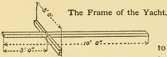
Fig. 215. The Backbone and Crosspiece.
