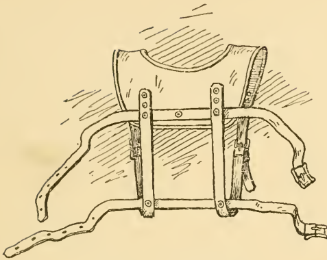
Fig. 213. Pack Harness.
