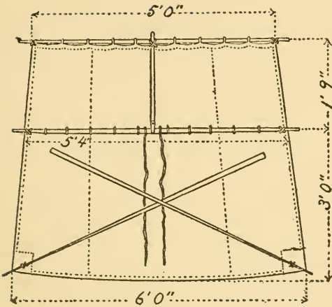
Fig. 15. The Danish Sail.
