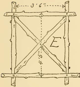
Fig. 309. E Frame (make four)
