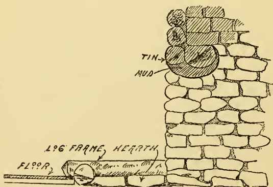
Fig. 275. Section through the Fireplace.
