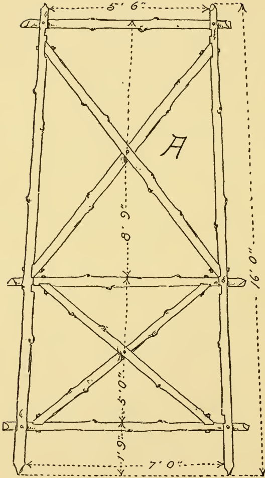
Fig. 305. A Frame (make four).
