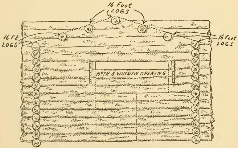
Fig. 271. How the Roof Logs were Laid.
