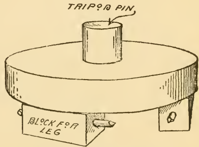
Fig. 73. The Tripod Head.
