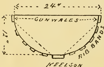
Fig. 106. Center Form.
