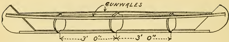
Fig. 127. Skeleton Frame of Canoe.
