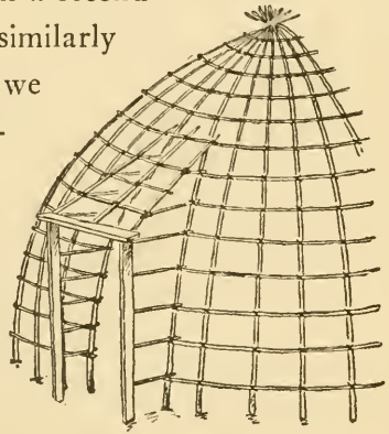
Fig. 132. Doorway of the Hut.
