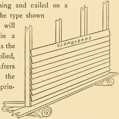
Fig. 141. Nailing on the Clapboards.
