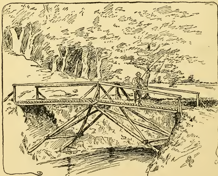
Fig 93. The Spar Bridge.
