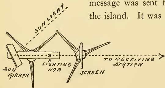
Fig. 160. Top View, showing position of Mirror and Shutter.
