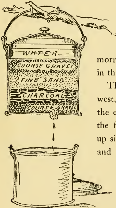
Fig. 68. The Small Filter.
