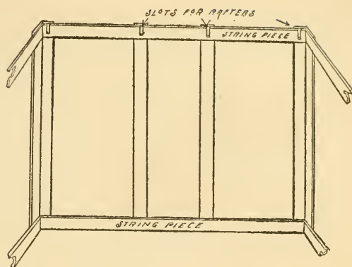
Fig. 183. Framework of the Cave.
