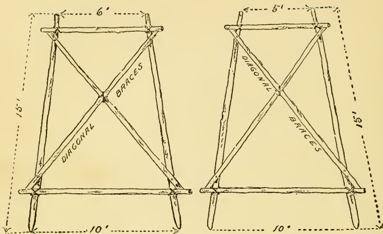
Figs. 91 and 92. Frames for the Spar Bridge.
