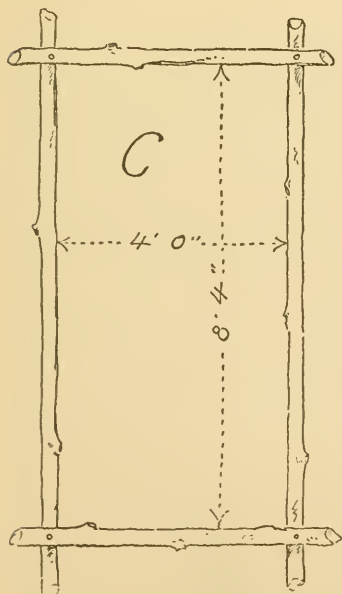
Fig. 307. C Frame (make four).
