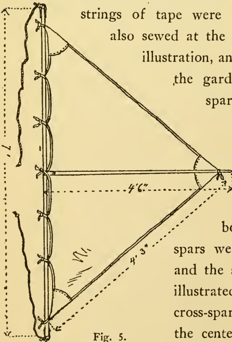
Fig. 5. "Bill's" Sail Complete.
