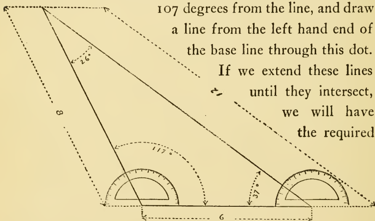
Fig. 83. Diagram of Our First Lesson in Surveying.
