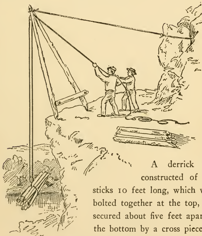
Fig. 137. The Derrick in Use.
