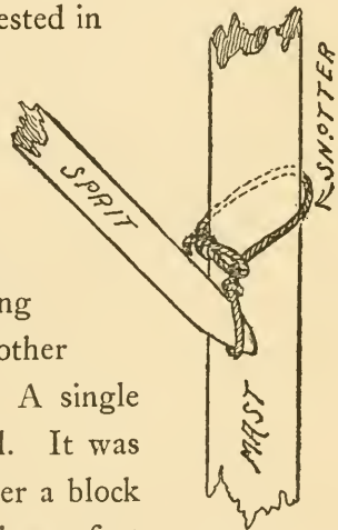
Fig. 193. The Snotter.
