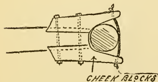
Fig. 170. Jaws of the Boom.
