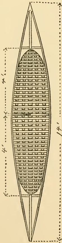
Fig. 109. Top View of the Canoe Frame.
