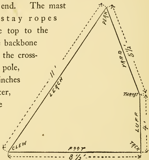
Fig. 169. The Mainsail.
