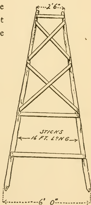
Fig. 283. Frame for the Tower.
