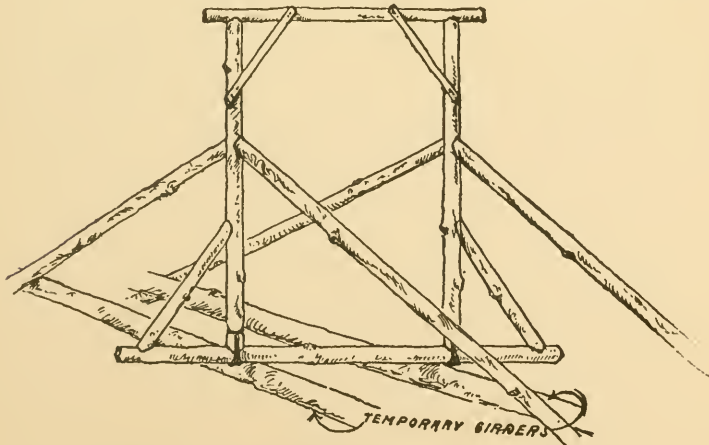
Fig. 103. The Permanent Cross Beam Made Fast.
