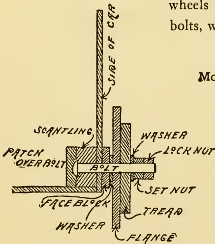
Fig. 300. Section Showing How to Fasten on the Wheel.
