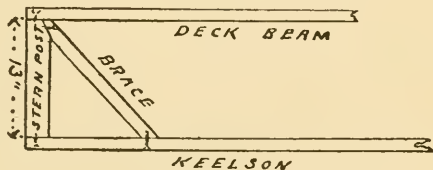
Fig. 104. Stern Post of the Canoe.
