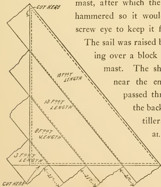
Fig. 224. Laying Out the Sail.
