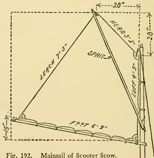
Fig. 192. Mainsail of Scooter Scow.
