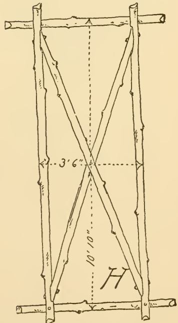
Fig. 312. H Frame (make one).
