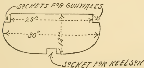
Fig. 124. Center Form.
