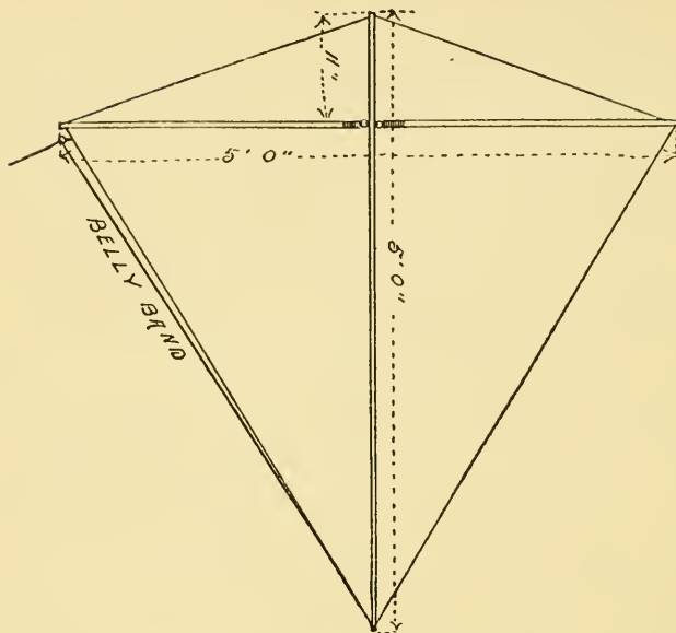
Fig. 241. The 5-foot Malay Kite.
