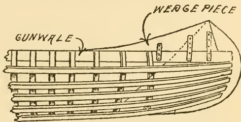
Fig. 129. Wedge Pieces at the Ends.
