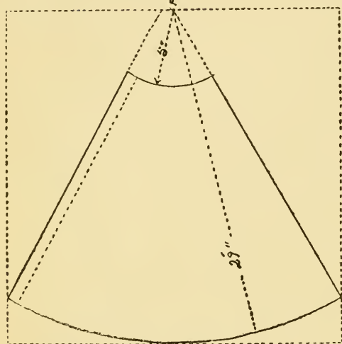
Fig. 55. Layout of the Megaphone.
