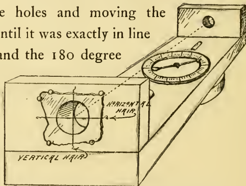
Fig. 72. Sighting Blocks on the Baseboard.
