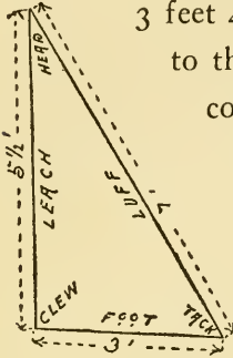
Fig. 172. The Jib-sail.
