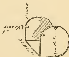
Fig. 202. Headboards.
