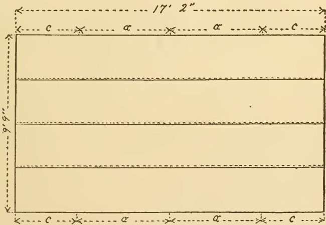
Fig. 37. Breadths sewed together for Roof and Side Walls of Tent.
