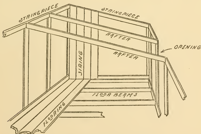
Fig. 184. The Siding and Flooring.
