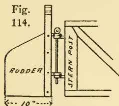
The Rudder Hinge.
