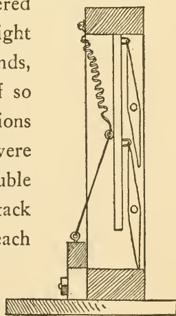
Fig. 157. Section through Shutter.
